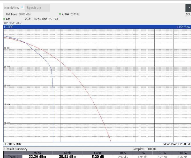
Band71-5MHz-16QAM-133297-25RB#0
