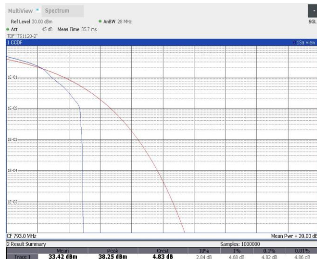
Band14-10MHz-16QAM-23330-50RB#0
