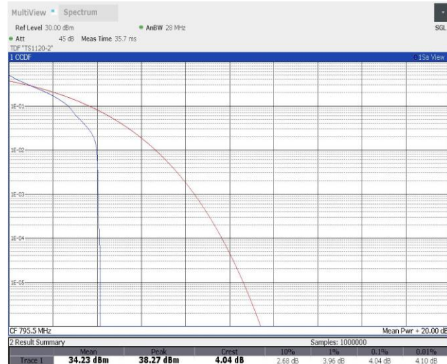
Band14-5MHz-QPSK-23355-25RB#0
