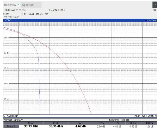
Band14-5MHz-16QAM-23330-25RB#0
