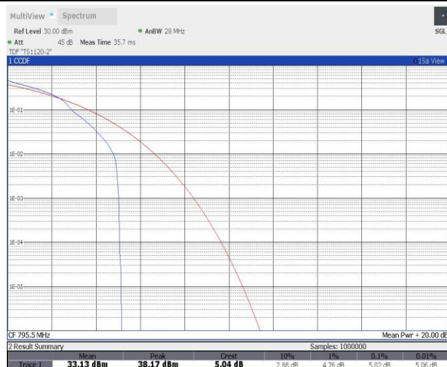
Band14-5MHz-16QAM-23355-25RB#0
