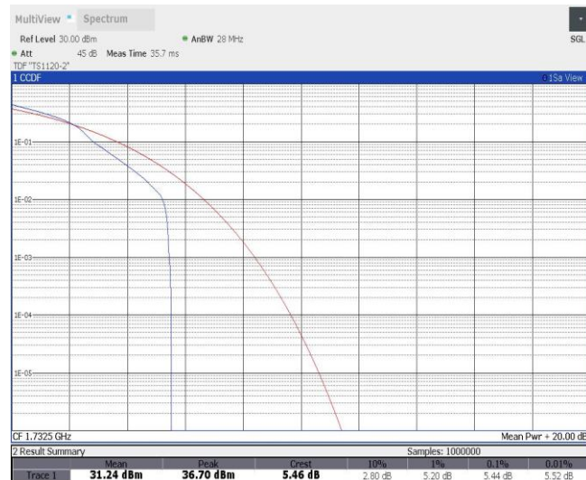
Band4-15MHz-16QAM-20175-75RB#0
