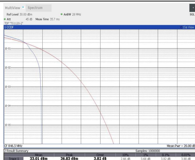
Band5-5MHz-16QAM-20625-25RB#0
