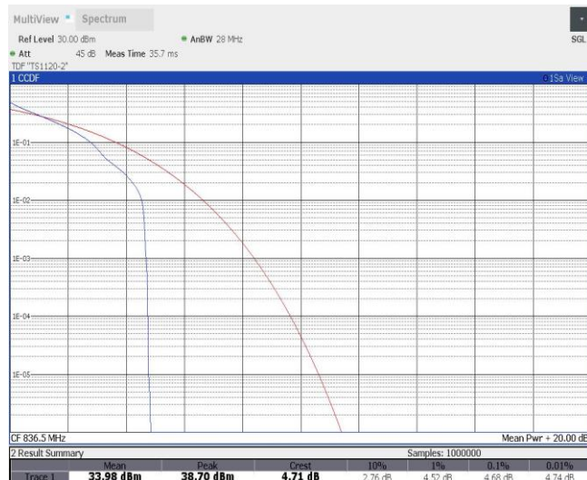
Band5-1.4MHz-QPSK-20525-6RB#0
