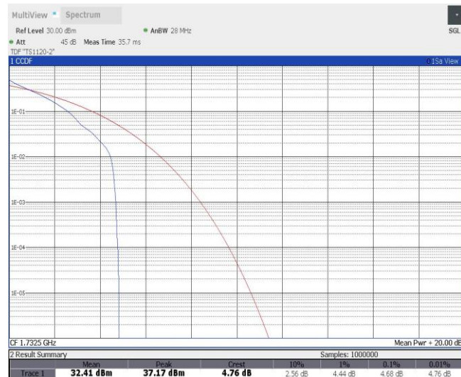
Band4-3MHz-QPSK-20175-15RB#0
