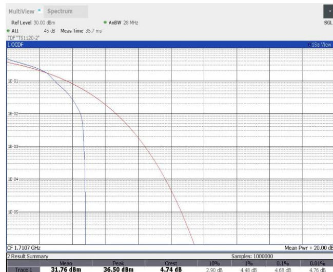
Band4-1.4MHz-16QAM-19957-6RB#0
