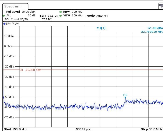
Band5-4132-1-0.15~30MHz
