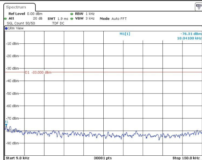
Band5-4132-4-0.009~0.15MHz
