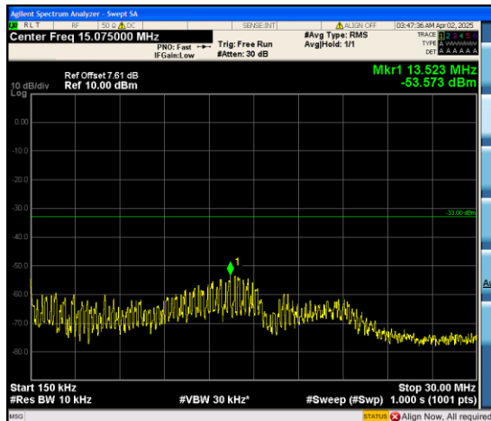
Band2_1.4MHz_QPSK_18900_6RB#0_0.15~30 _0.15~30
