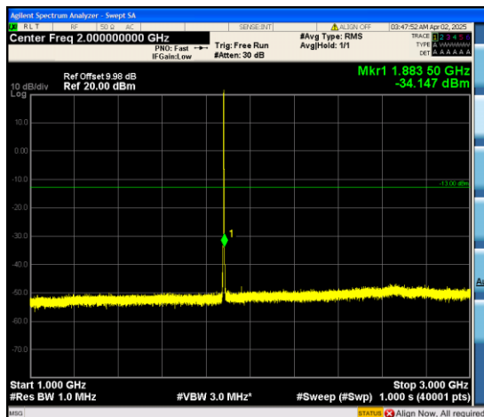
Band2_1.4MHz_QPSK_18900_6RB#0_1000~30 00_1000~3000
