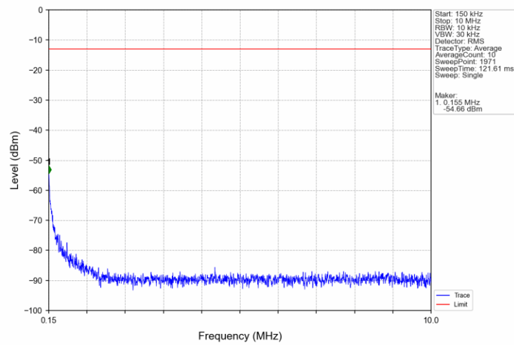
Band71_10MHz_16QAM_HCH_693MHz_RB_1_0_NTNV
