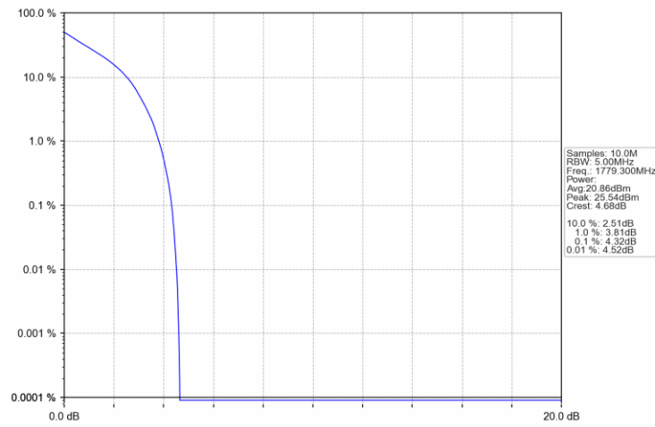
Band66_1.4MHz_QPSK_HCH_1779.3MHz_RB_6_0_NTNV
