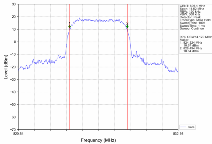
Band5_HSDPA_LCH_826.4MHz_Subtest 1_NTNV
