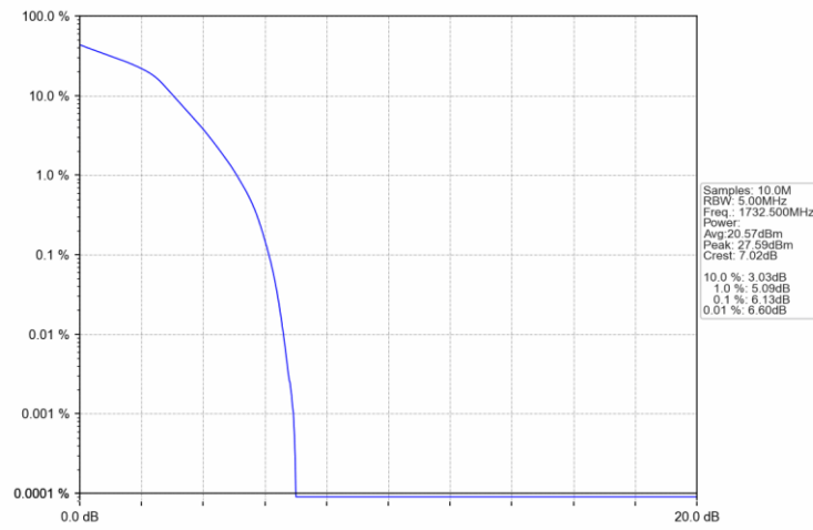
Band4_1.4MHz_16QAM_MCH_1732.5MHz_RB_6_0_NTNV
