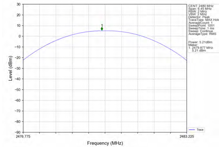
Pi/4DQPSK_2DH5_HCH_2480MHz_Ant1_NTNV
