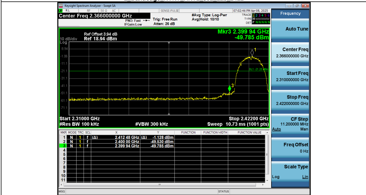
2 Bandedge_NVNT_ANT1_802_11b_2412
