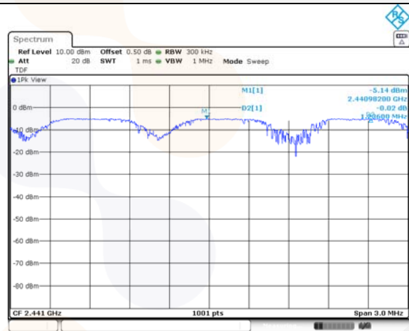
GFSK / Mid ch.
