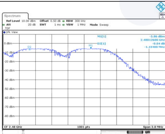
GFSK / High ch.
