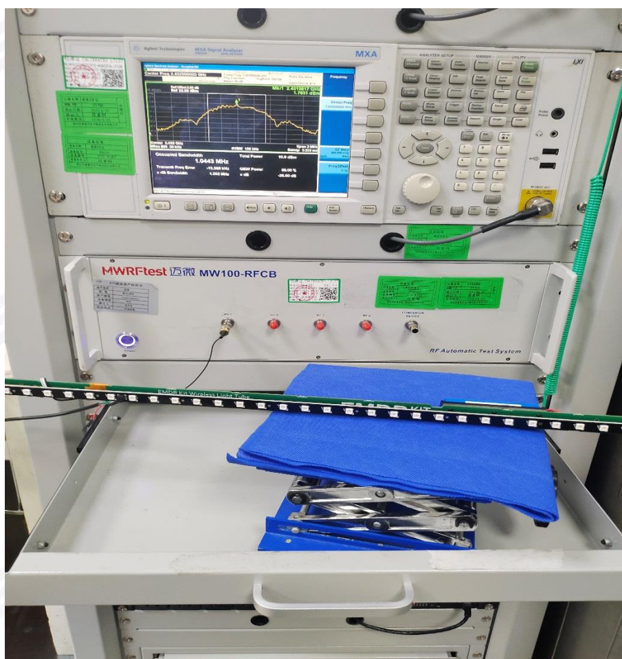
RF conduction
