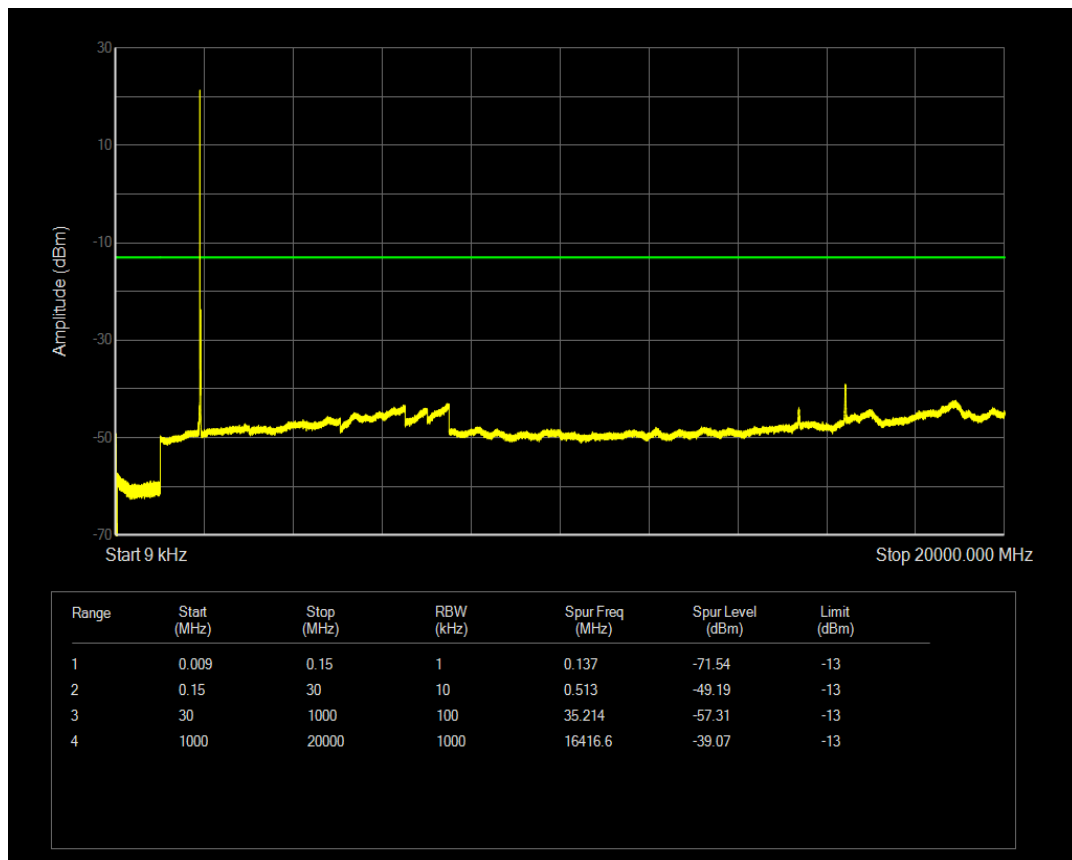
LTE Band38 QPSK BW=5MHz Channel=37775 RB Size=1 Position=#0
