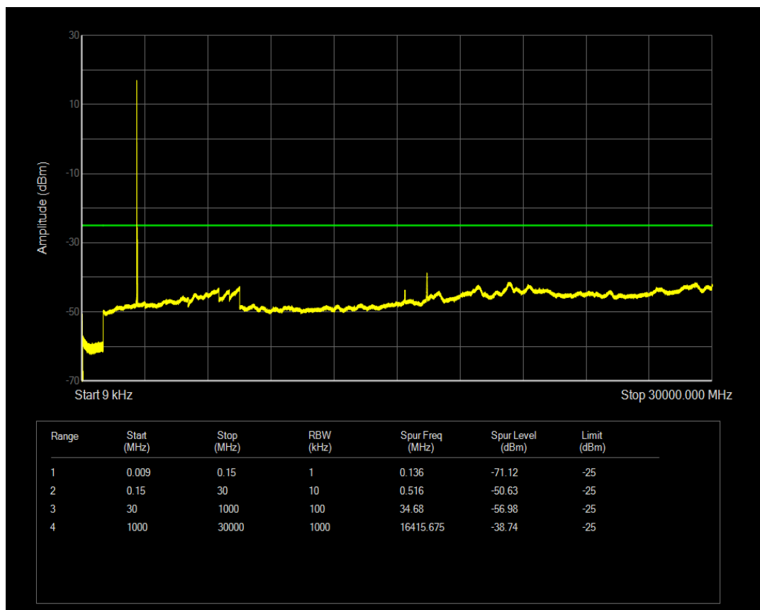
LTE Band41 QPSK BW=5MHz Channel=39675 RB Size=1 Position=#0
