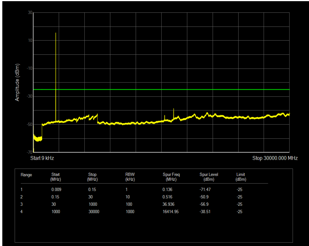
LTE Band38 QPSK BW=10MHz Channel=37800 RB Size=1 Position=#0
