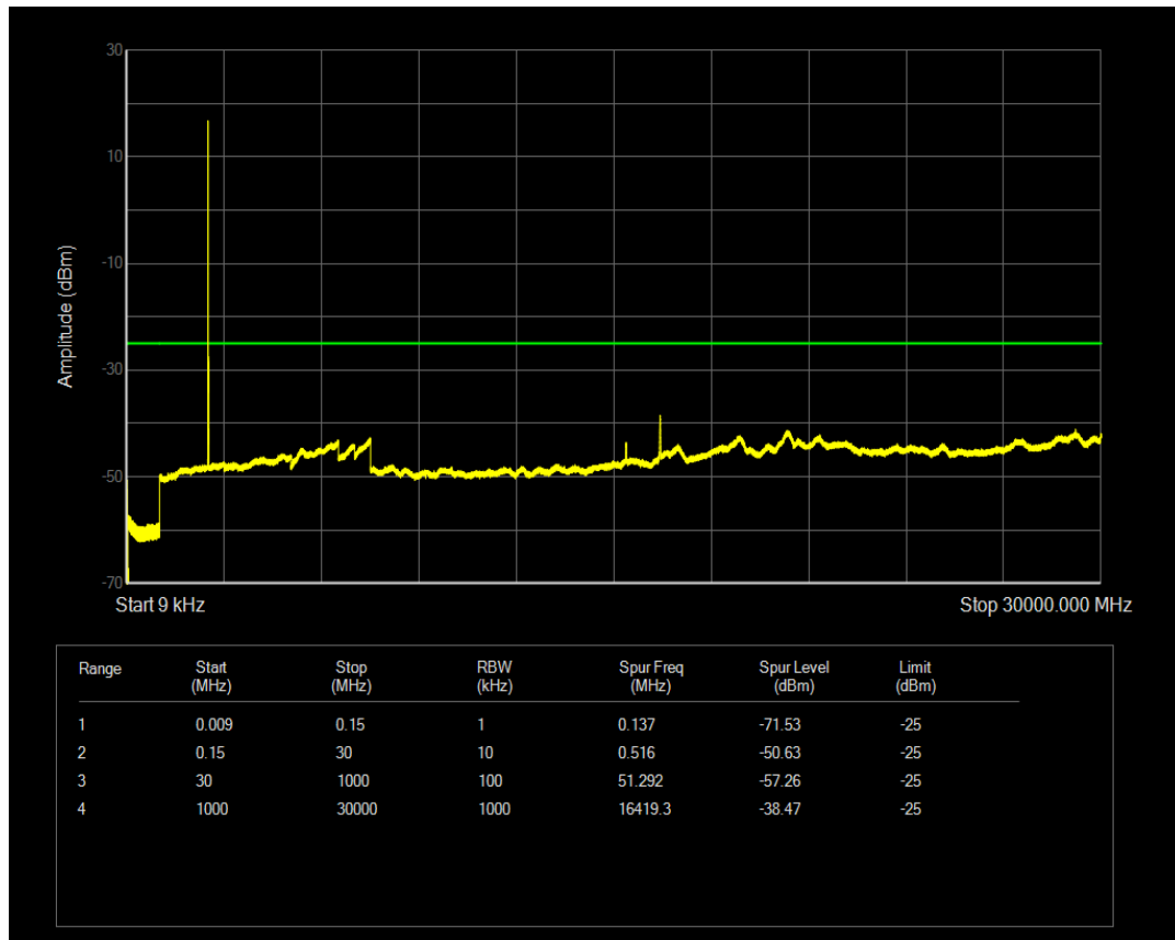
LTE Band41 QPSK BW=5MHz Channel=40620 RB Size=1 Position=#0
