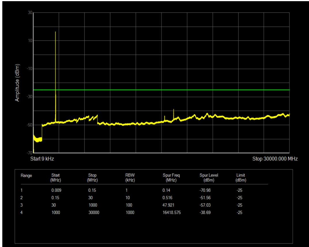
LTE Band41 QPSK BW=20MHz Channel=41490 RB Size=1 Position=#0
