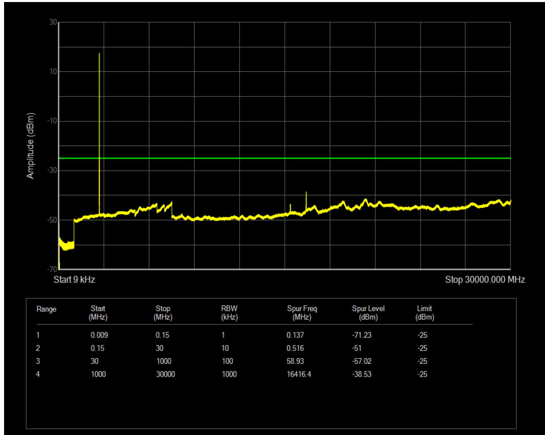
LTE Band41 QPSK BW=10MHz Channel=39700 RB Size=1 Position=#0
