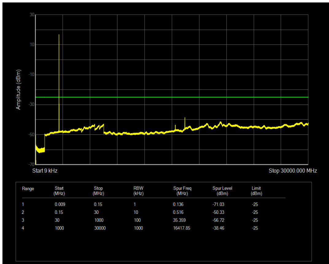
LTE Band38 QPSK BW=10MHz Channel=38000 RB Size=1 Position=#0
