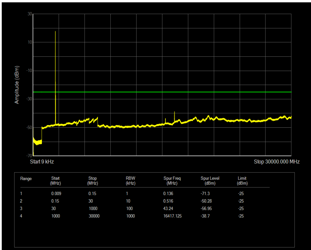
LTE Band41 QPSK BW=15MHz Channel=41515 RB Size=1 Position=#0
