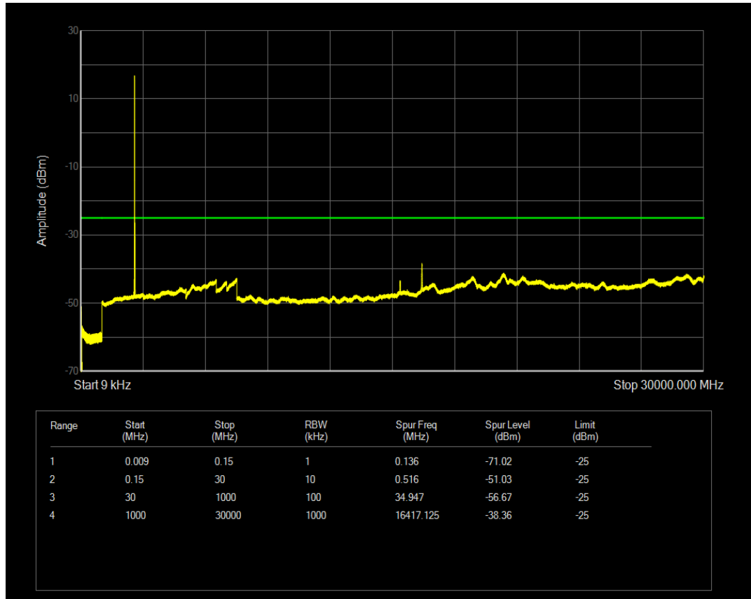
LTE Band38 QPSK BW=15MHz Channel=38000 RB Size=1 Position=#0
