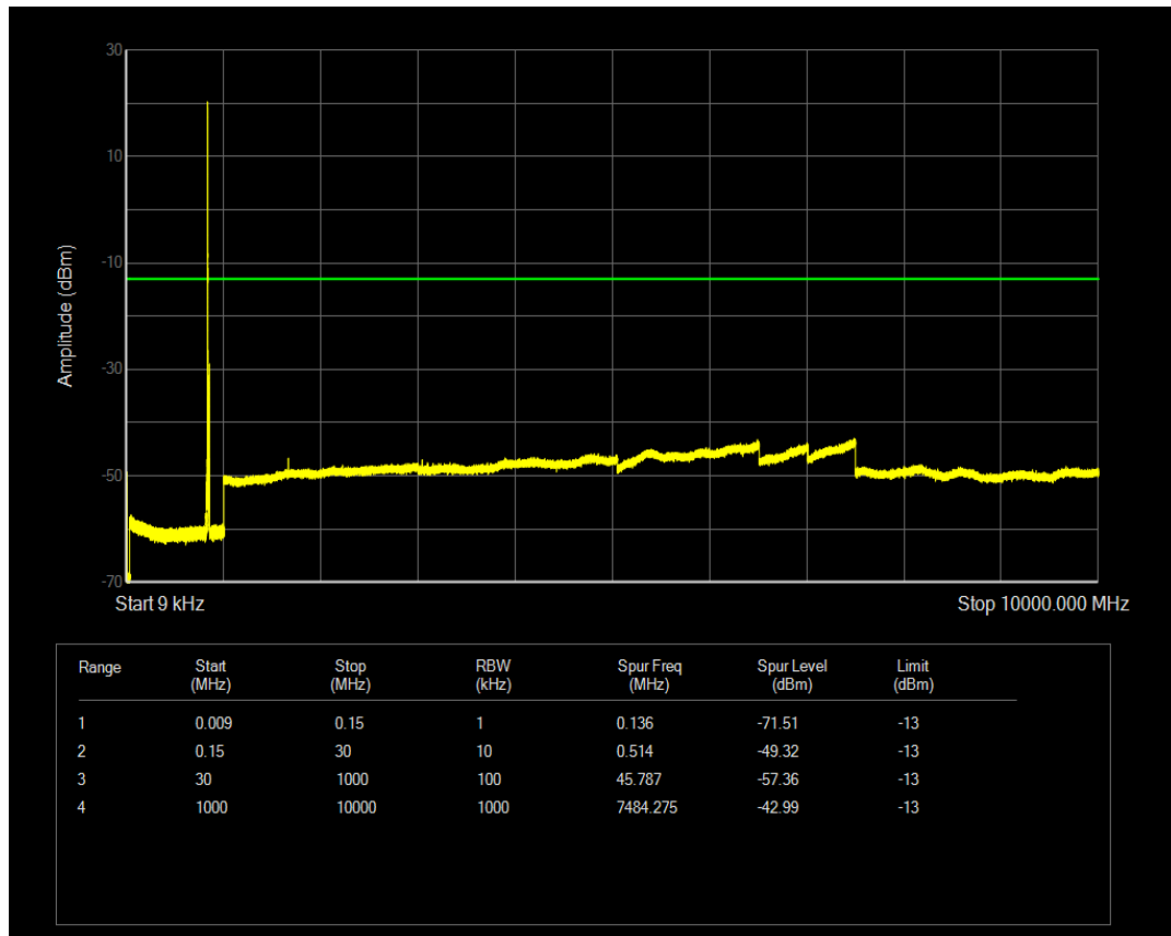
LTE Band5 QPSK BW=10MHz Channel=20600 RB Size=1 Position=#0
