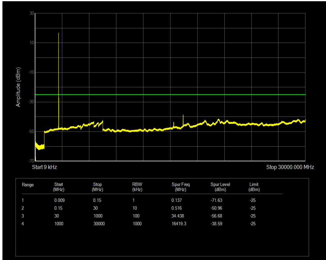
LTE Band38 QPSK BW=10MHz Channel=38200 RB Size=1 Position=#0
