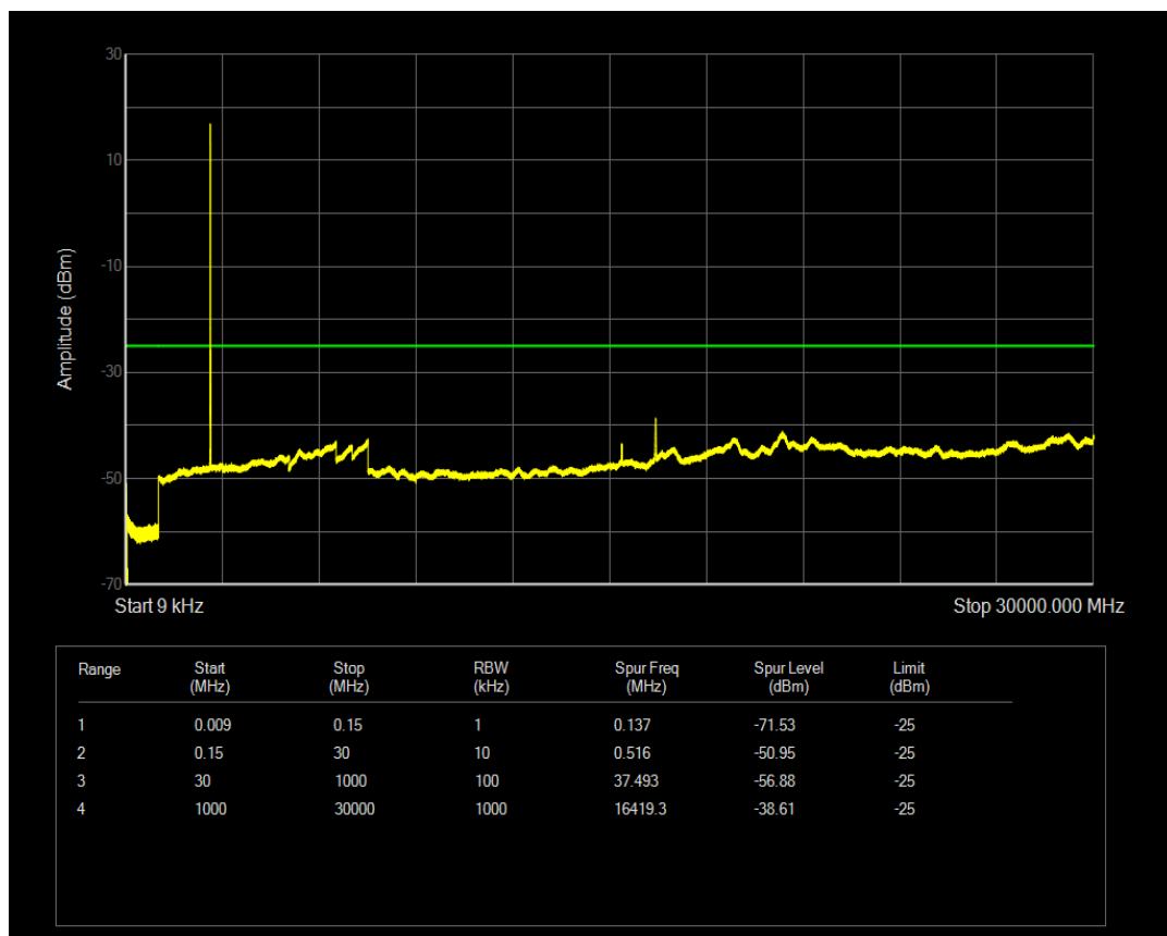
LTE Band38 QPSK BW=15MHz Channel=37825 RB Size=1 Position=#0
