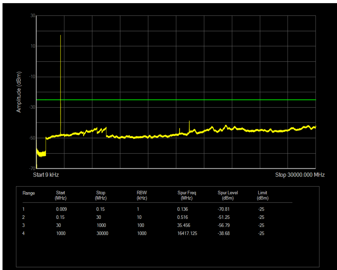
LTE Band41 QPSK BW=5MHz Channel=41565 RB Size=1 Position=#0
