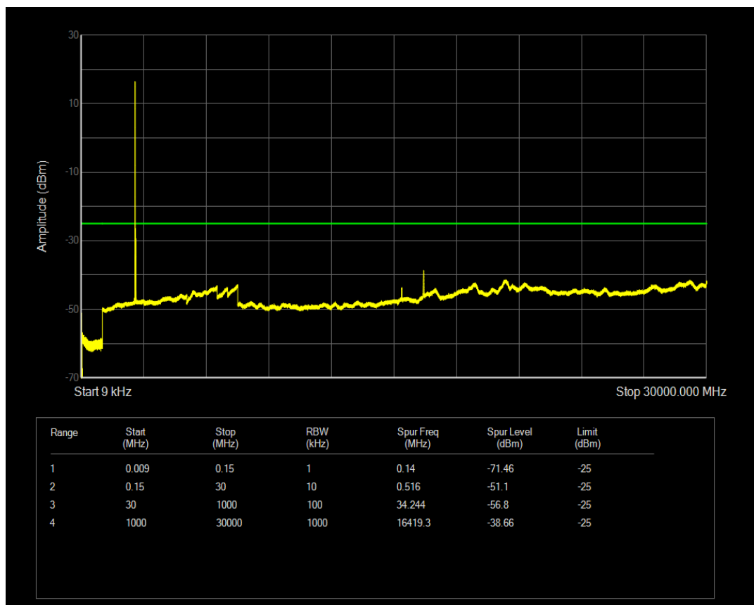
LTE Band38 QPSK BW=20MHz Channel=38000 RB Size=1 Position=#0
