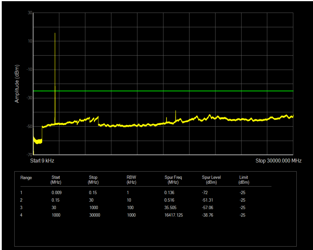
LTE Band41 QPSK BW=15MHz Channel=40620 RB Size=1 Position=#0
