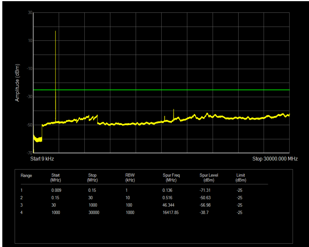
LTE Band41 QPSK BW=10MHz Channel=41540 RB Size=1 Position=#0
