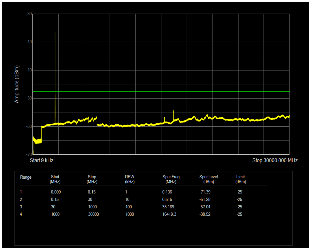
LTE Band38 QPSK BW=5MHz Channel=38225 RB Size=1 Position=#0
