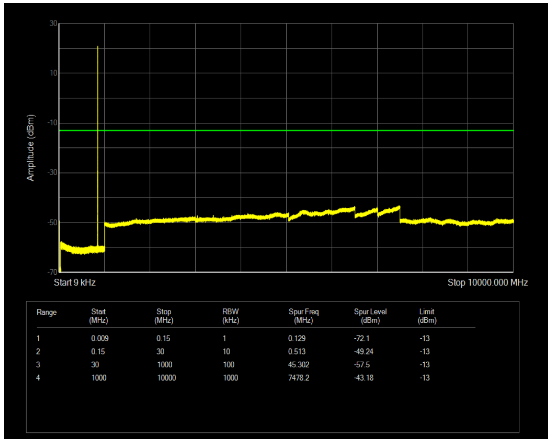
LTE Band5 QPSK BW=3MHz Channel=20415 RB Size=1 Position=#0
