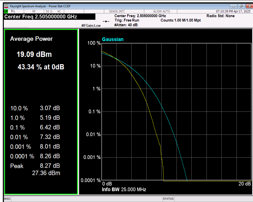
Band7 64QAM BW=10MHz Channel=20800 RB Size=50 Position=#0
