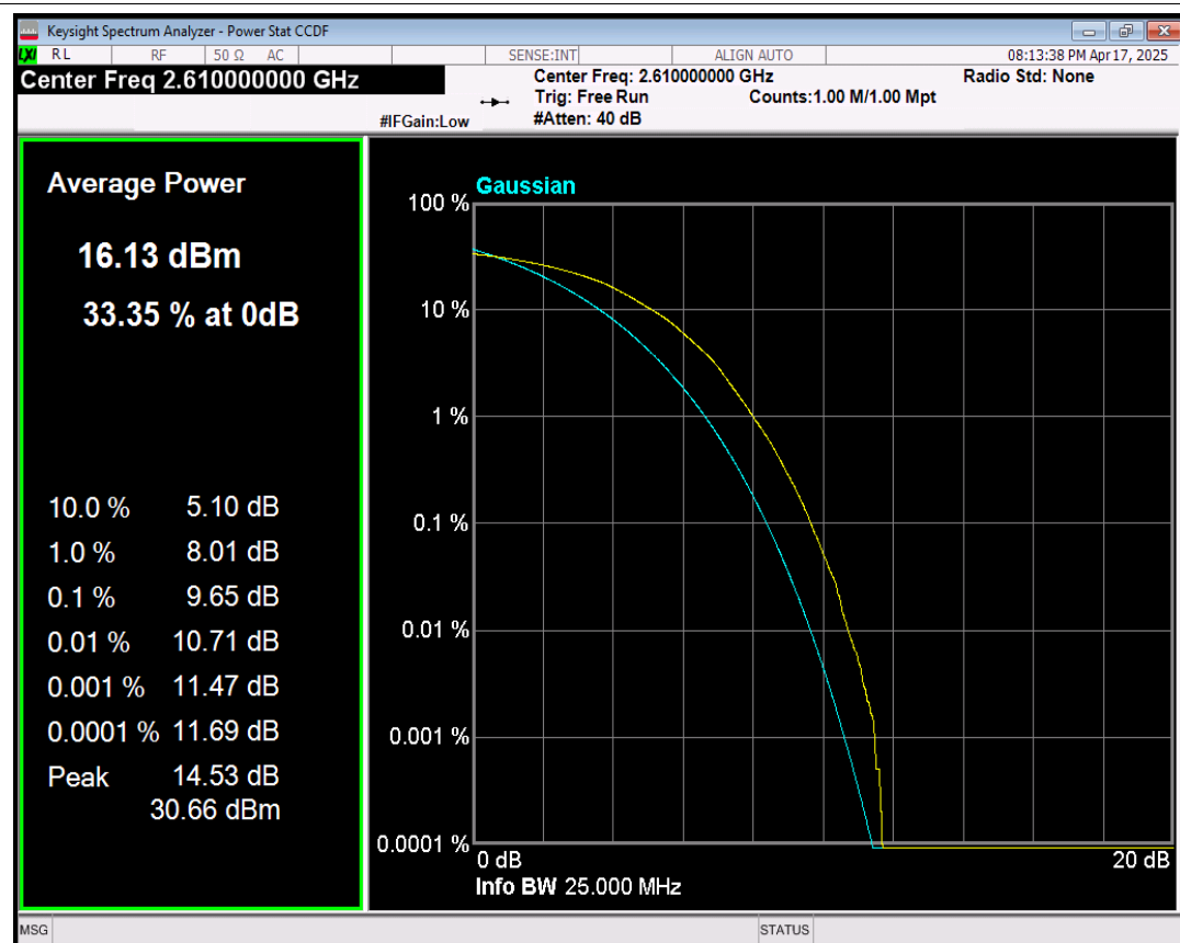
Band38 64QAM BW=20MHz Channel=38150 RB Size=100 Position=#0
