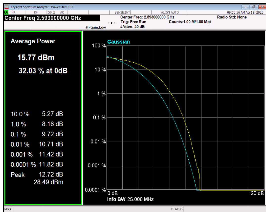
Band41 64QAM BW=5MHz Channel=40620 RB Size=25 Position=#0
