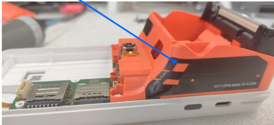
Main Antenna
