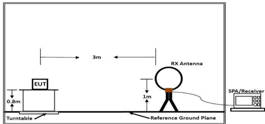
Below 30MHz
