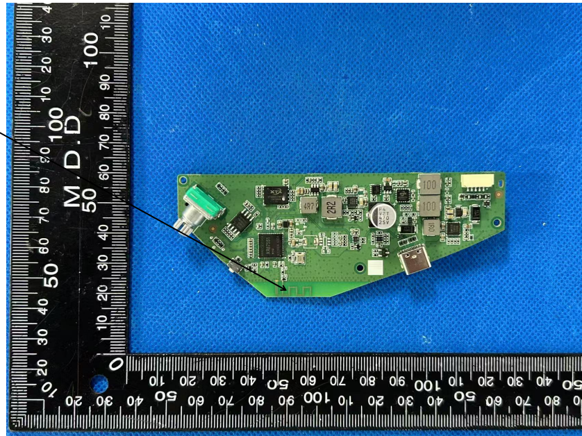
PCB Antenna
