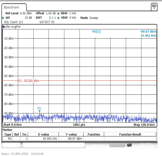
Band41_20MHz_16QAM_39750_1RB#0_0.009~0.15
