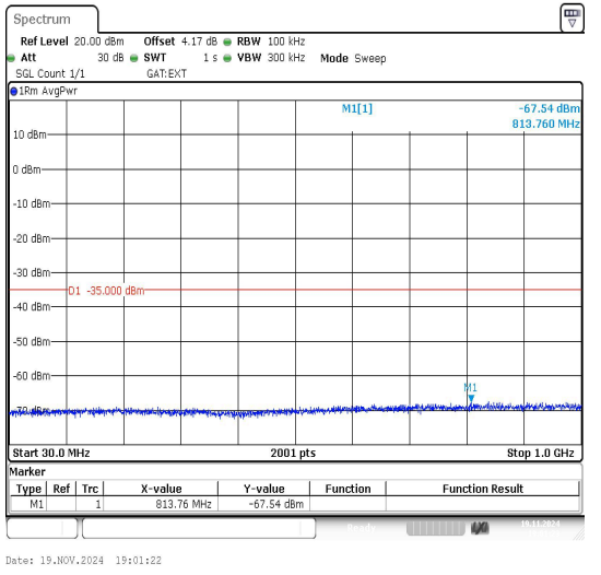
Band41_20MHz_16QAM_39750_1RB#0_30~1000
