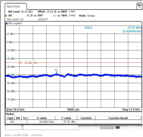
Band41_20MHz_QPSK_39750_1RB#0_20000~27000
