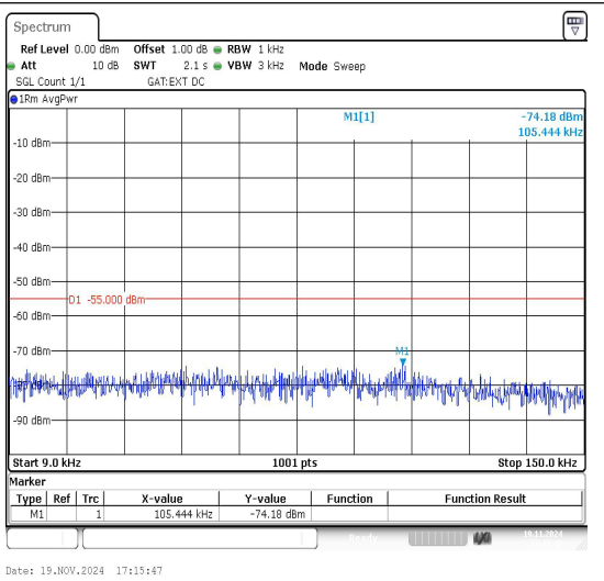
Band41_10MHz_16QAM_41540_1RB#0_0.009~0.15
