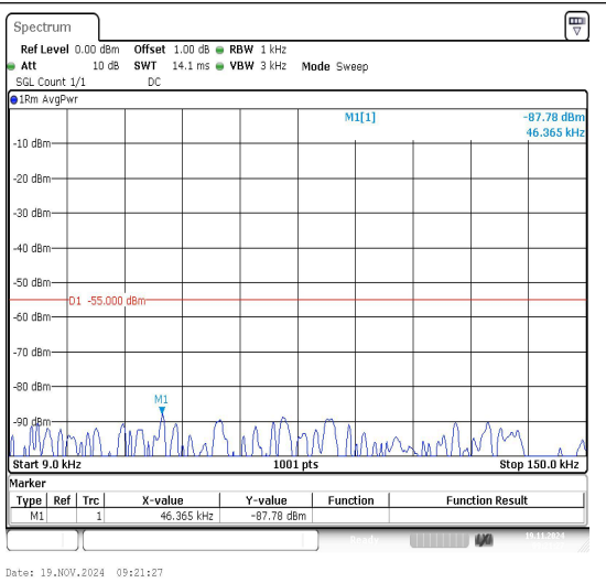
Band7_5MHz_16QAM_20775_1RB#0_0.009~0.15_0.009~0.15
