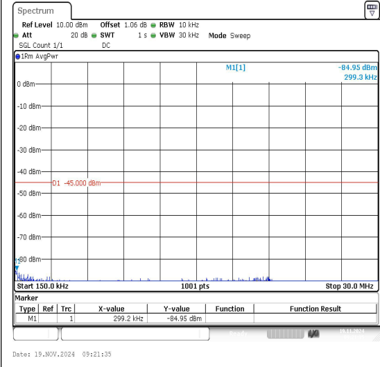
Band7_5MHz_16QAM_20775_1RB#0_0.15~30_0.15~30
