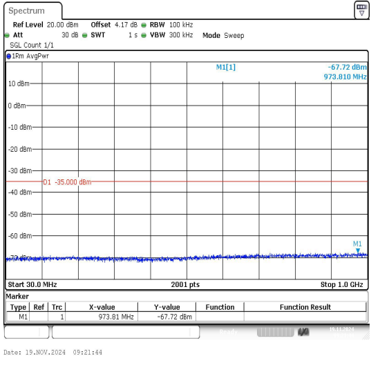
Band7_5MHz_16QAM_20775_1RB#0_30~1000_30~1000
