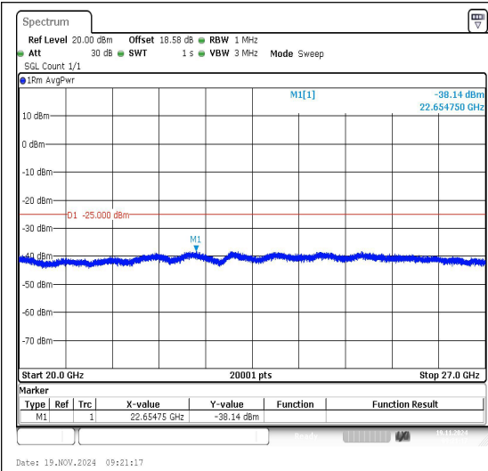
Band7_5MHz_QPSK_20775_1RB#0_20000~27000_20000~27000
