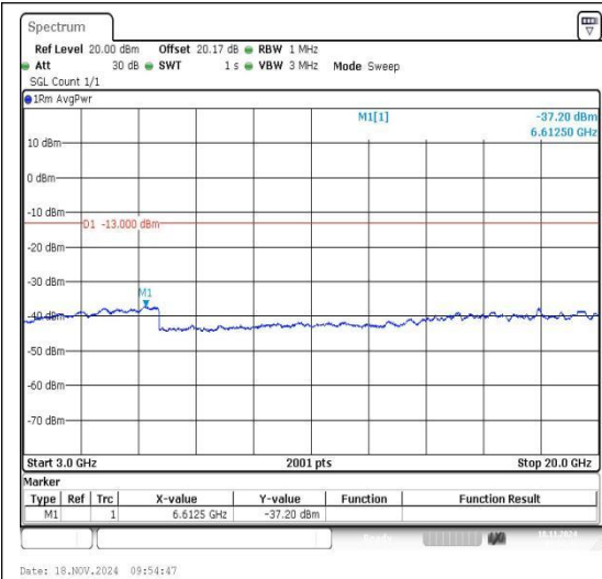
Band2_10MHz_QPSK_18900_1RB#0_3000~20000_3000~20000
