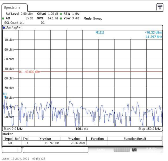
Band2_10MHz_16QAM_19150_1RB#0_0.009~0.15_0.009~0.15
