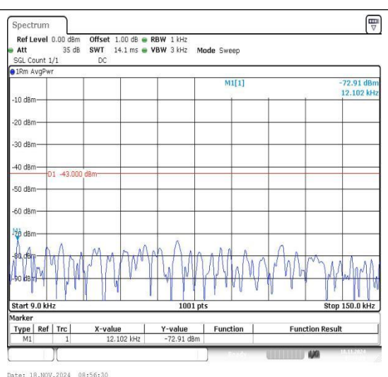
Band2_3MHz_16QAM_19185_1RB#0_0.009~0.15 0.009~0.15
