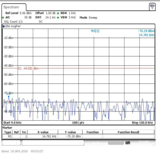
Band2_10MHz_16QAM_18650_1RB#0_0.009~0.15_0.009~0.15
