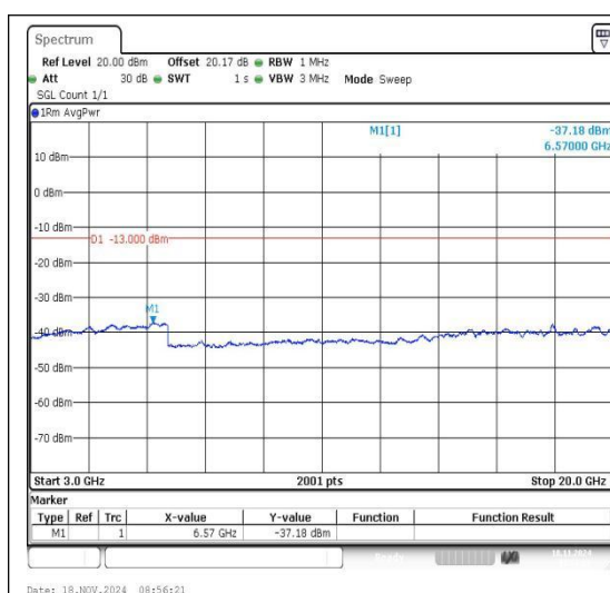
Band2_3MHz_QPSK_19185_1RB#0_3000~2000 0 3000~20000
