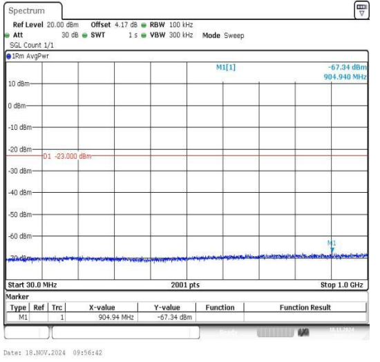
Band2_10MHz_16QAM_19150_1RB#0_30~1000_30~1000
