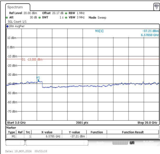
Band2_10MHz_QPSK_18650_1RB#0_3000~20000_3000~20000
