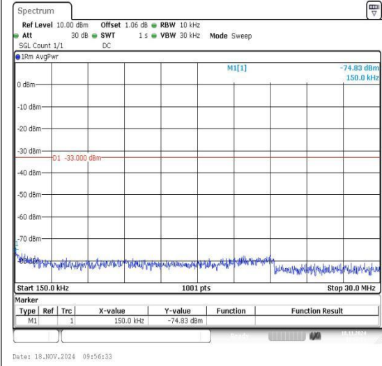
Band2_10MHz_16QAM_19150_1RB#0_0.15~30_0.15~30
