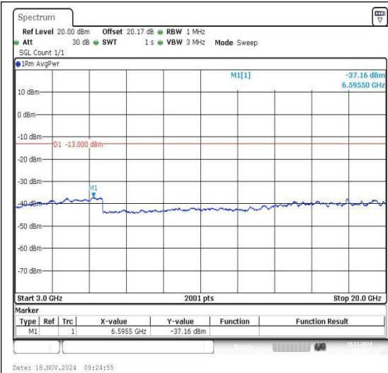
Band2_5MHz_QPSK_18900_1RB#0_3000~2000 0_3000~20000
