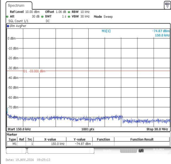
Band2_5MHz_16QAM_18900_1RB#0_0.15~30 0.15~30
