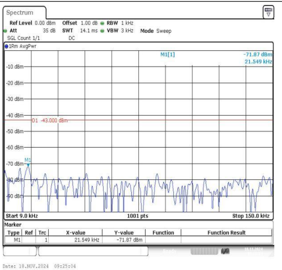
Band2_5MHz_16QAM_18900_1RB#0_0.009~0.15 _0.009~0.15
