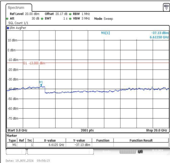
Band2_10MHz_QPSK_19150_1RB#0_3000~20000_3000~20000
