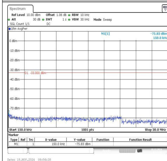
Band2_3MHz_16QAM_19185_1RB#0_0.15~30_0.15~30
