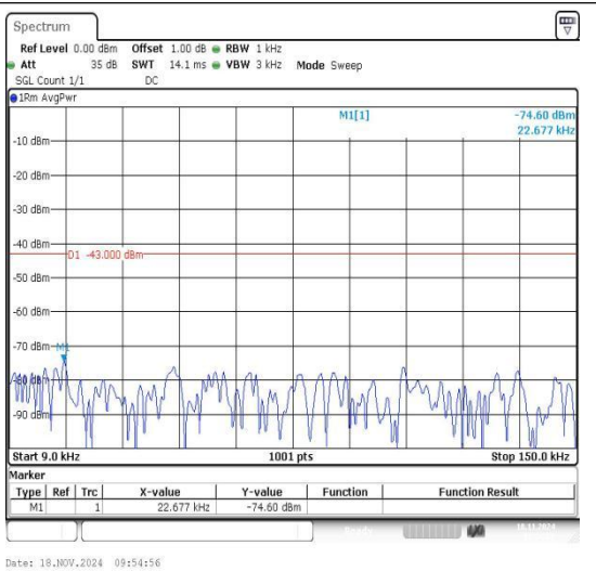
Band2_10MHz_16QAM_18900_1RB#0_0.009~0.15_0.009~0.15
