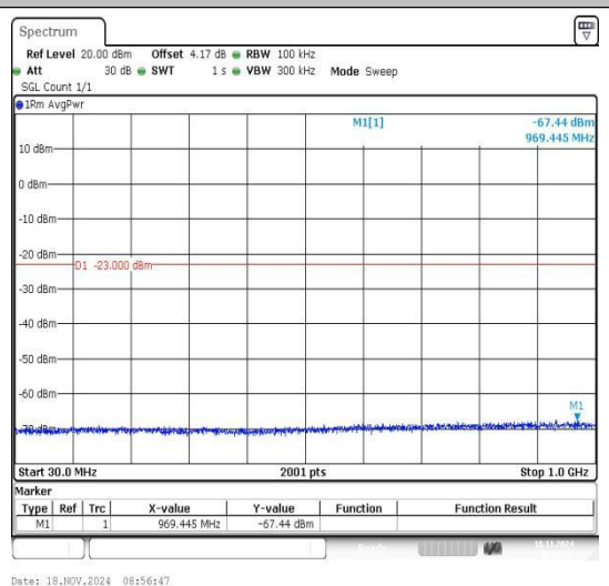
Band2_3MHz_16QAM_19185_1RB#0_30~1000_3 0~1000
