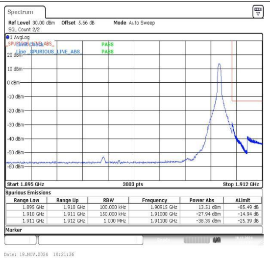
Band2_15MHz_QPSK_19125_1RB#74
