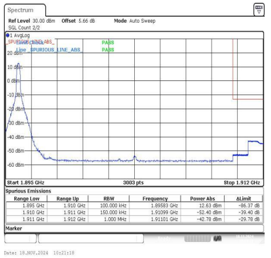
Band2_15MHz_16QAM_19125_1RB#0
