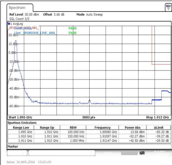
Band2_15MHz_QPSK_19125_1RB#0
