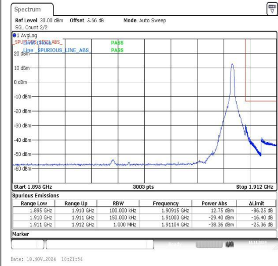
Band2_15MHz_16QAM_19125_1RB#74
