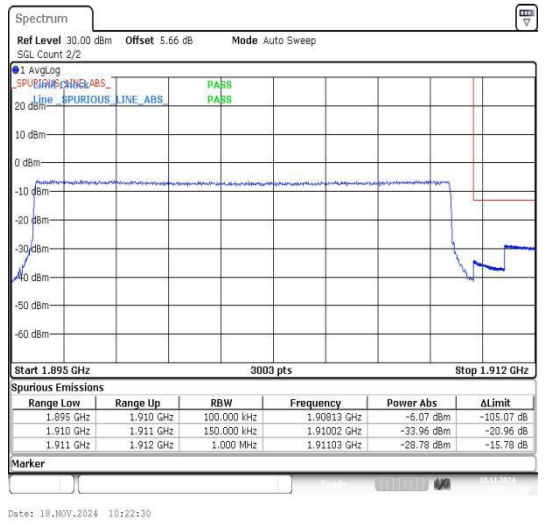
Band2_15MHz_16QAM_19125_75RB#0
