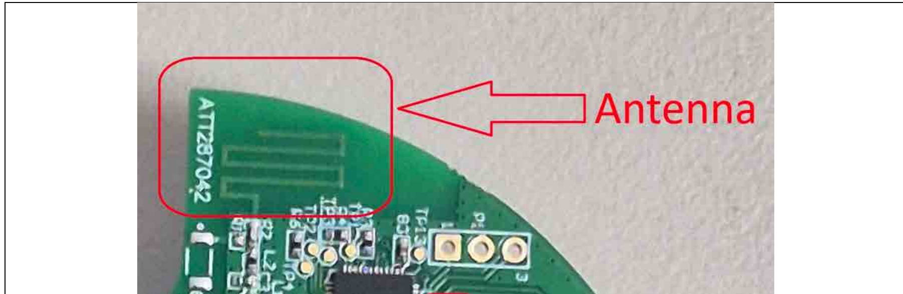
Antenna MIFA PCB printed
