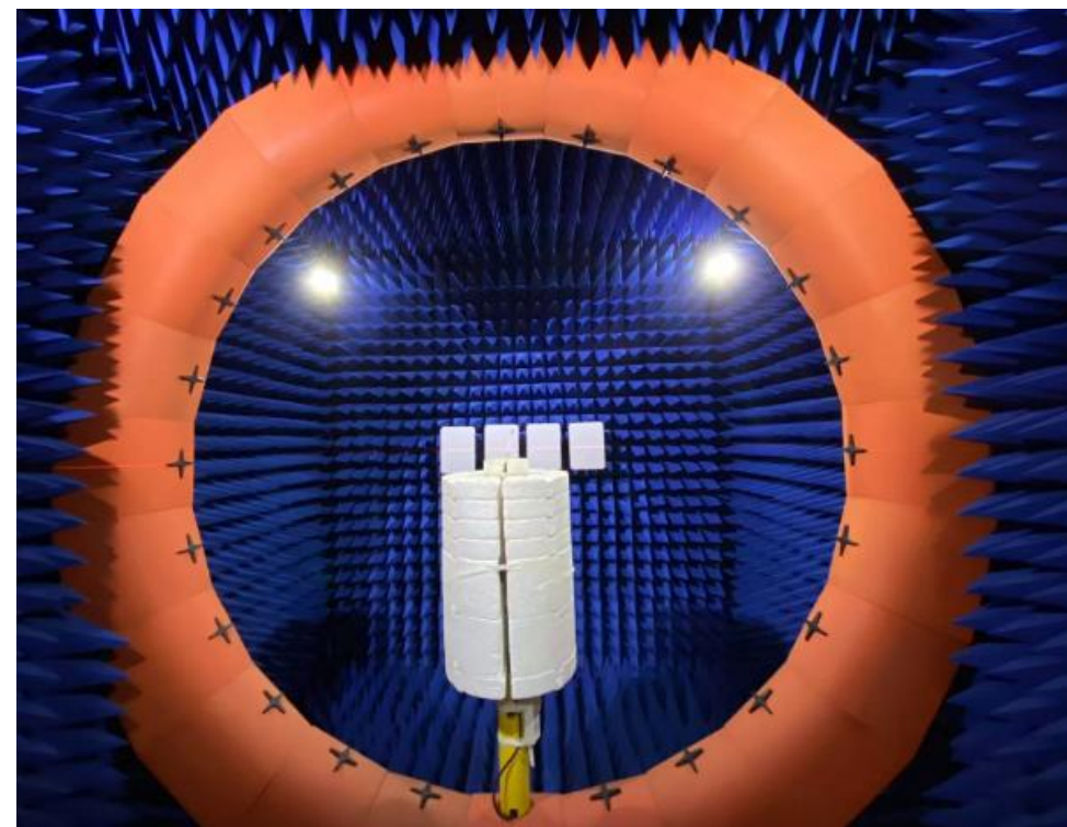
Testing 3D microwave darkroom(6m*6m*6m)
