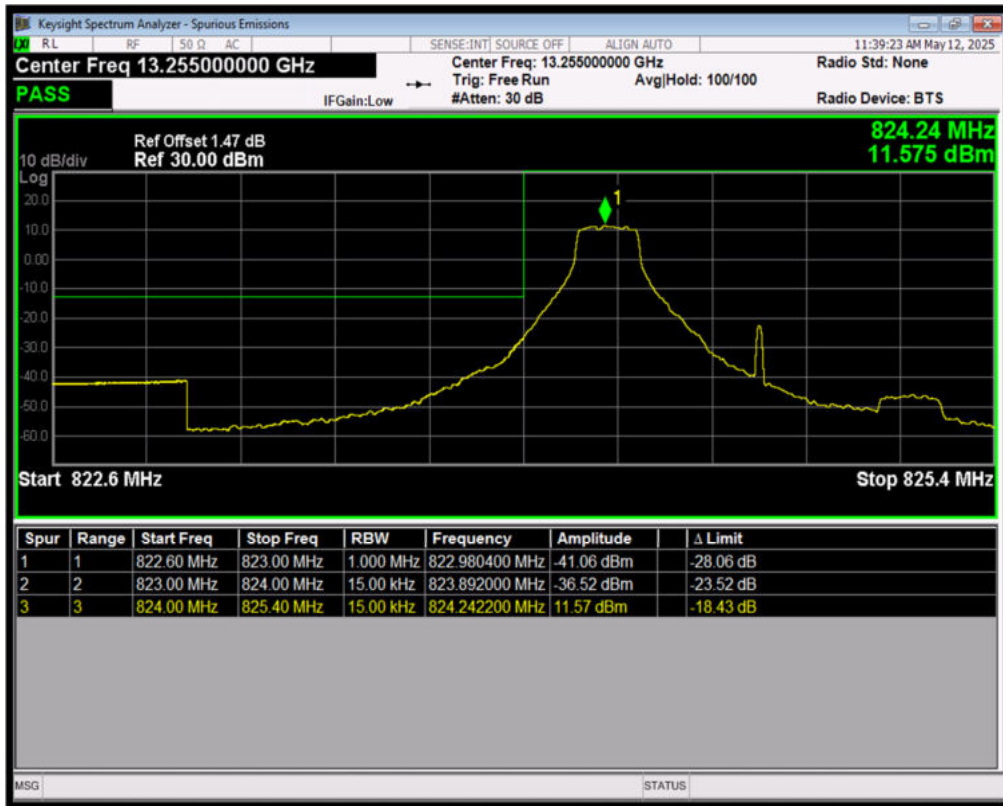
Band5 16QAM BW=1.4MHz LowChannel=20407 RB Size=1 Position=#0
