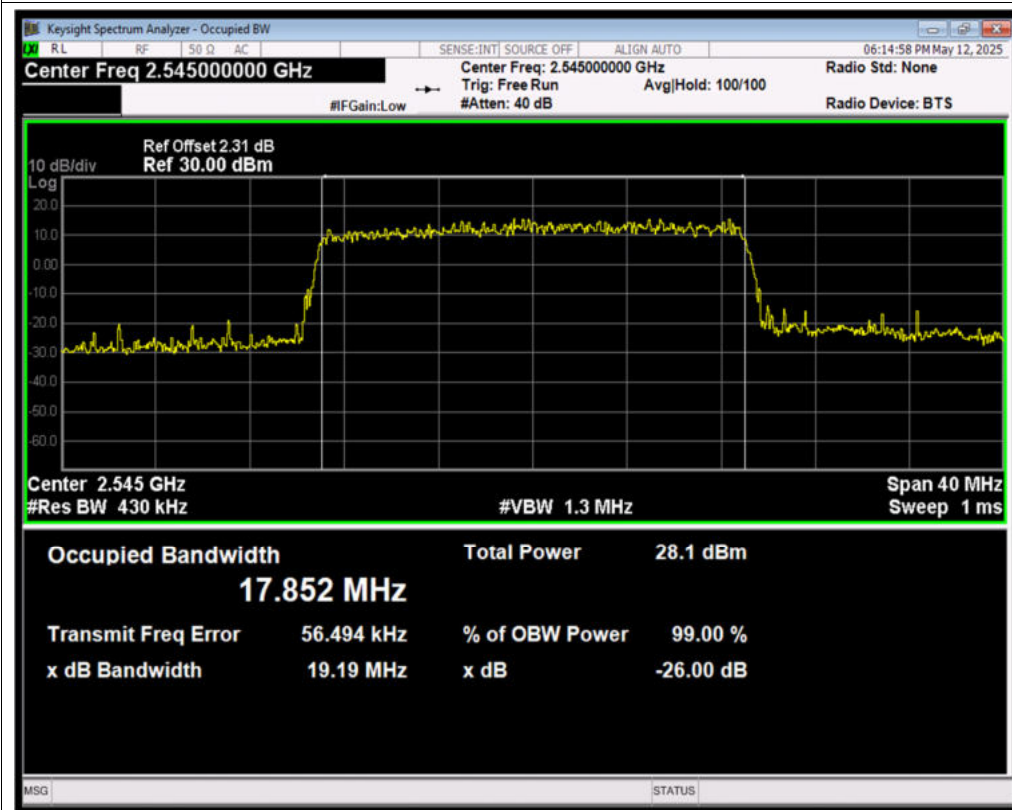
Band41(2535-2655) QPSK BW=20MHz Channel=40140 RB Size=100 Position=#0
