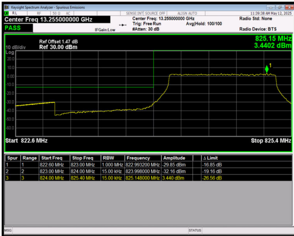
Band5 16QAM BW=1.4MHz LowChannel=20407 RB Size=6 Position=#0
