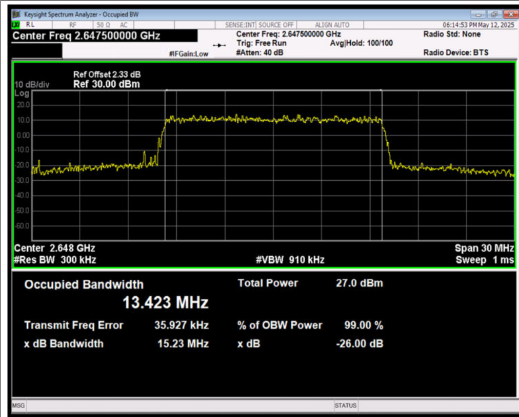
Band41(2535-2655) 64QAM BW=15MHz Channel=41165 RB Size=75 Position=#0
