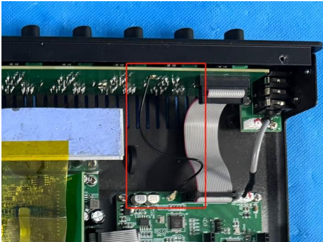
View of wireless antenna
