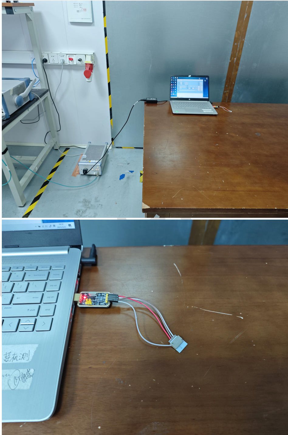
Conducted emissions at AC power line (150kHz-30MHz)
