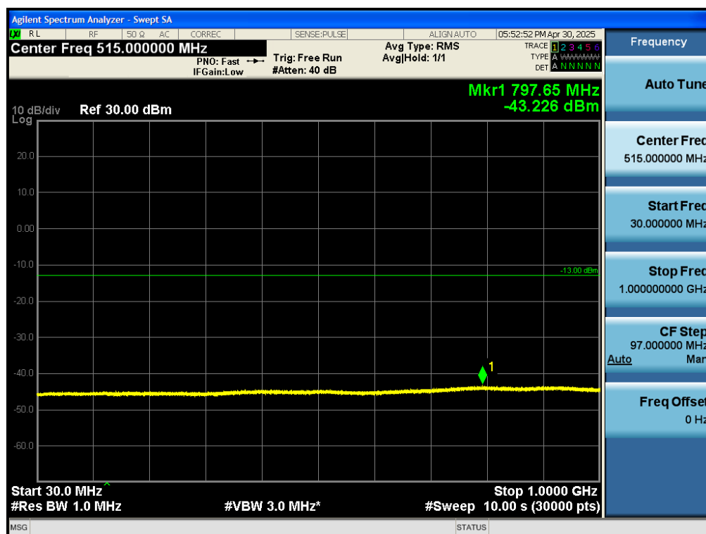
Test_Graph_band66_1745MHz_15M_QPSK_75RB#LOW_30M_1G_TX
