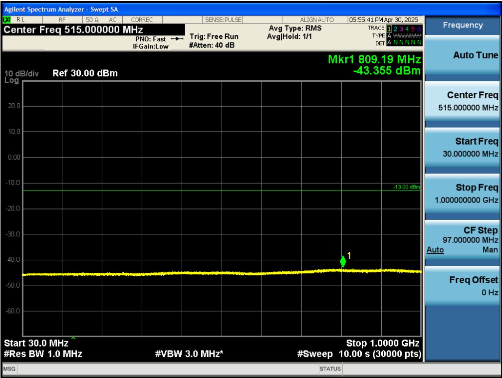
Test_Graph_band66_1770MHz_20M_QPSK_100RB#LOW_30M_1G_TX
