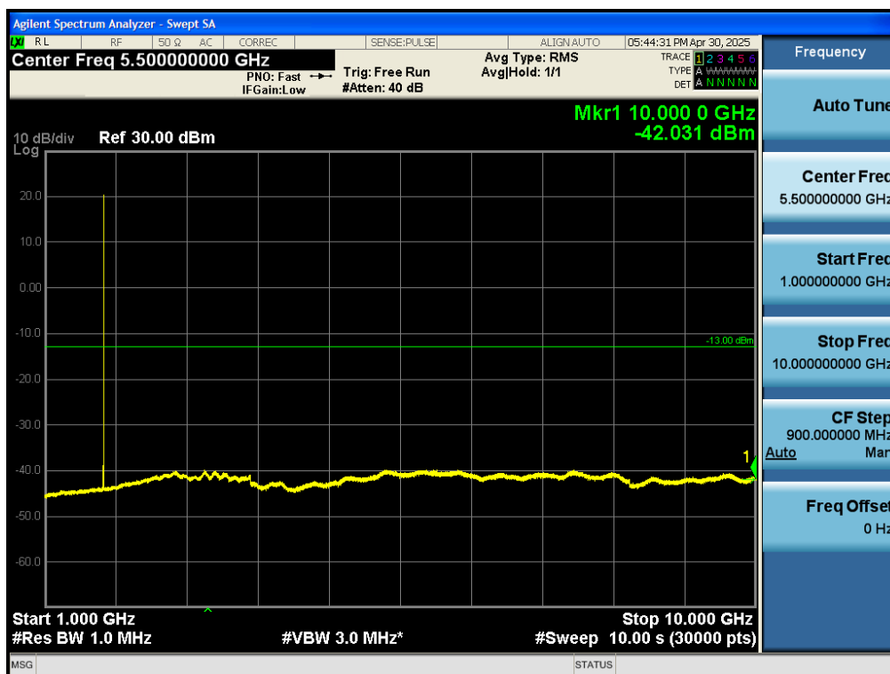
Test_Graph_band66_1745MHz_1.4M_QPSK_6RB#LOW_1G_10G_TX
