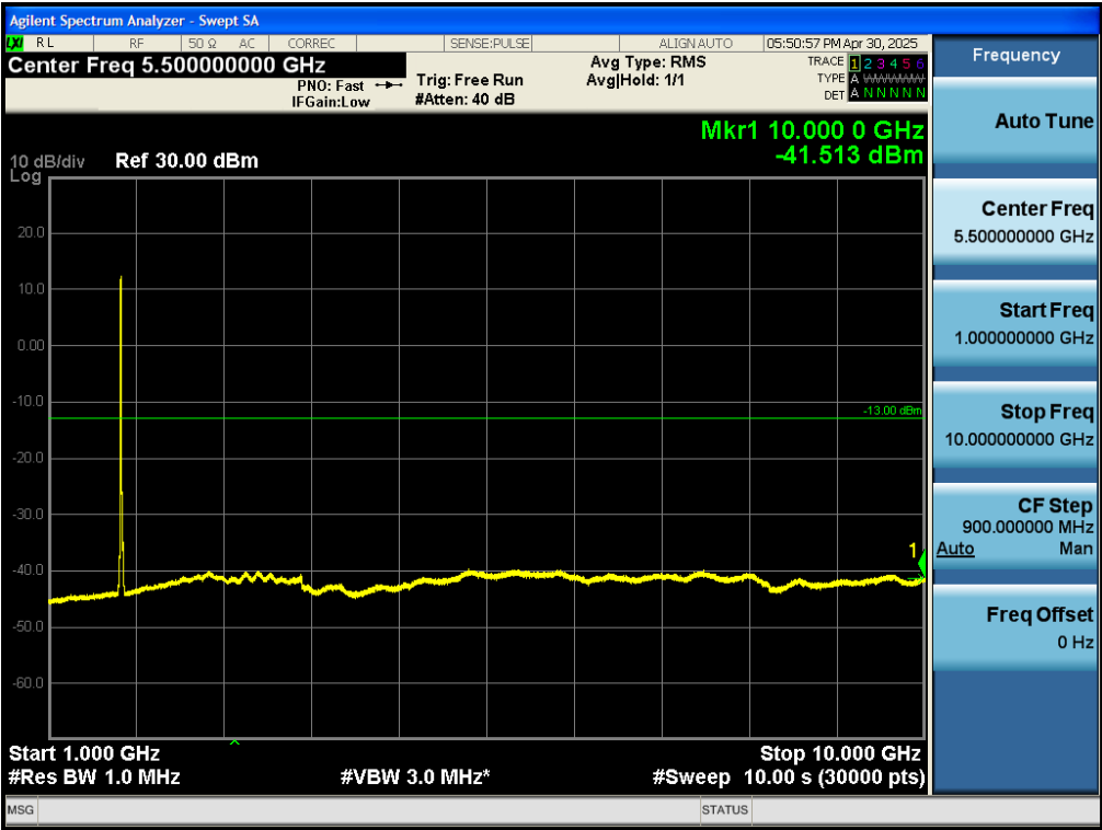
Test_Graph_band66_1745MHz_10M_QPSK_50RB#LOW_1G_10G_TX
