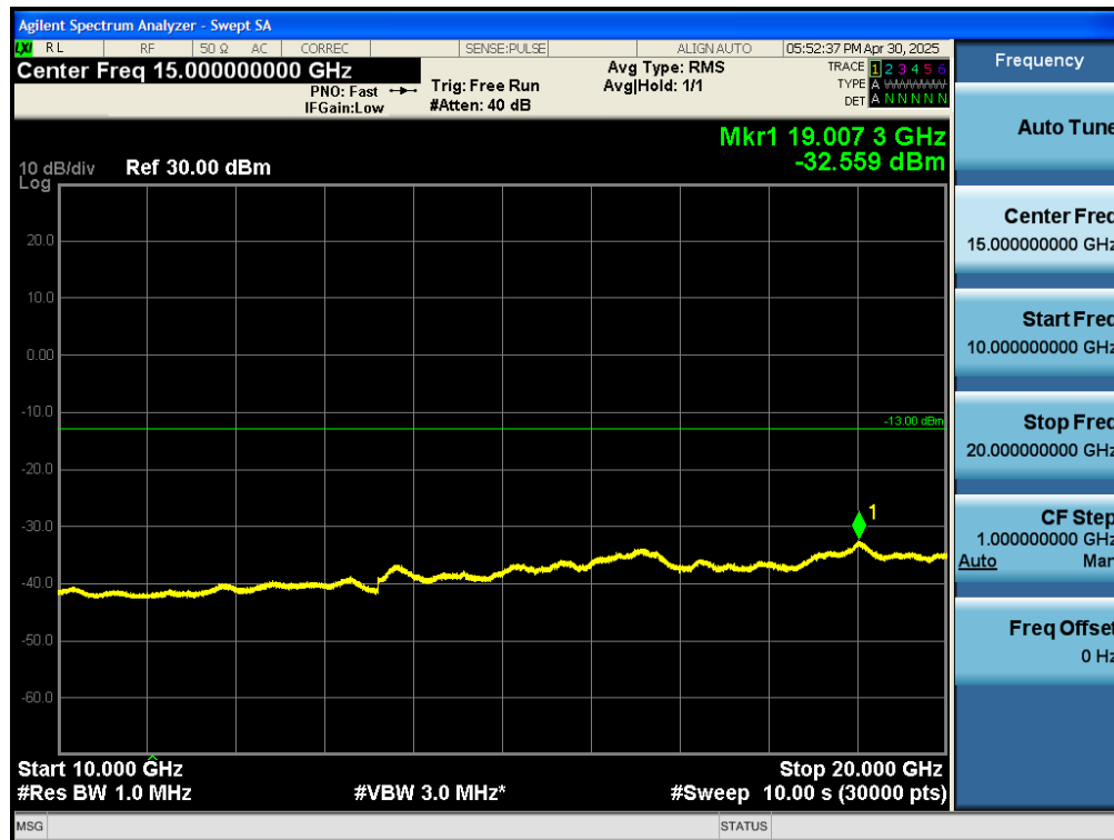
Test_Graph_band66_1717.5MHz_15M_QPSK_75RB#LOW_10G_20.0G_TX
