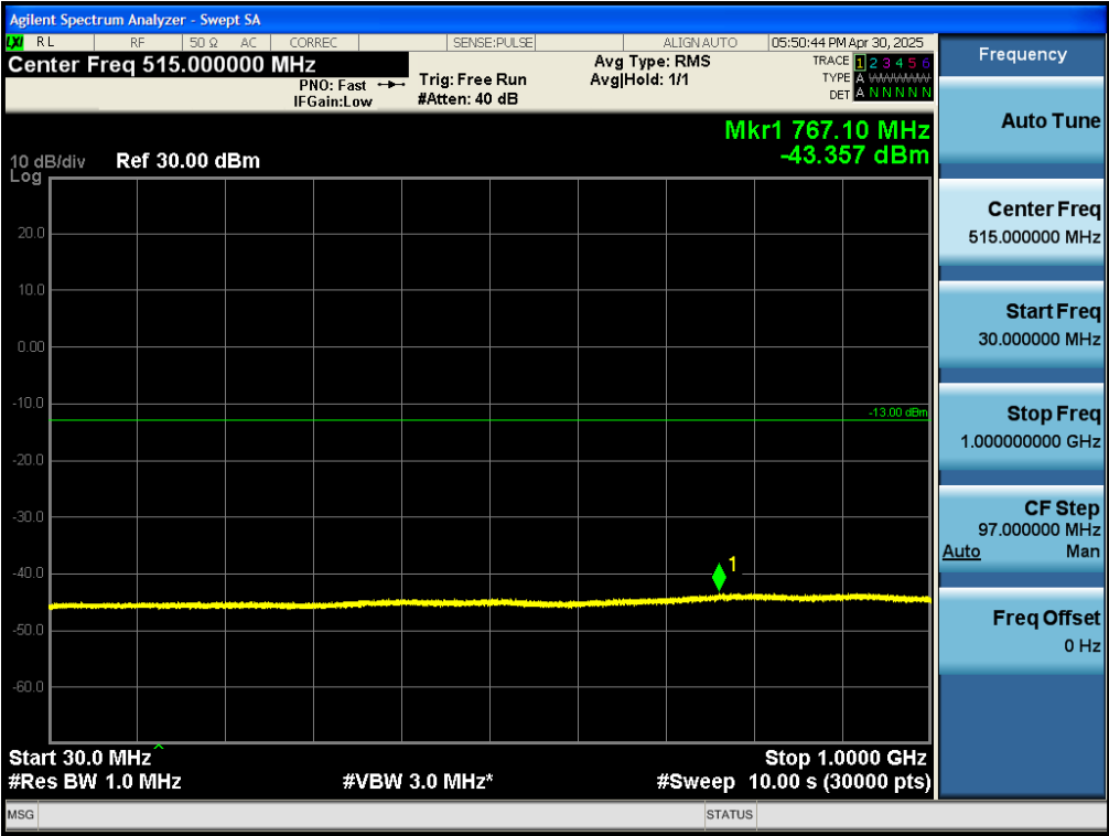
Test_Graph_band66_1745MHz_10M_QPSK_50RB#LOW_30M_1G_TX
