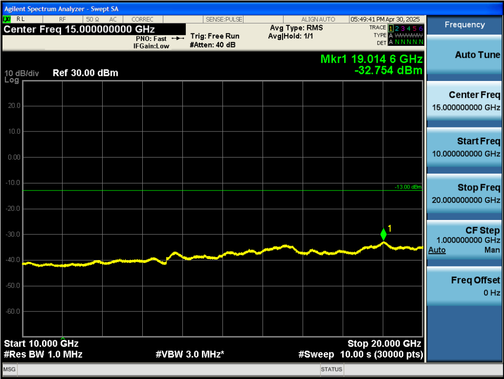
Test_Graph_band66_1777.5MHz_5M_QPSK_25RB#LOW_10G_20.0G_TX
