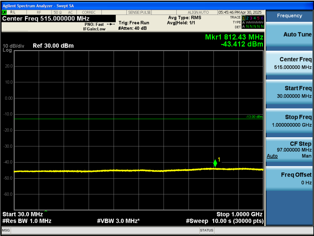
Test_Graph_band66_1711.5MHz_3M_QPSK_15RB#LOW_30M_1G_TX
