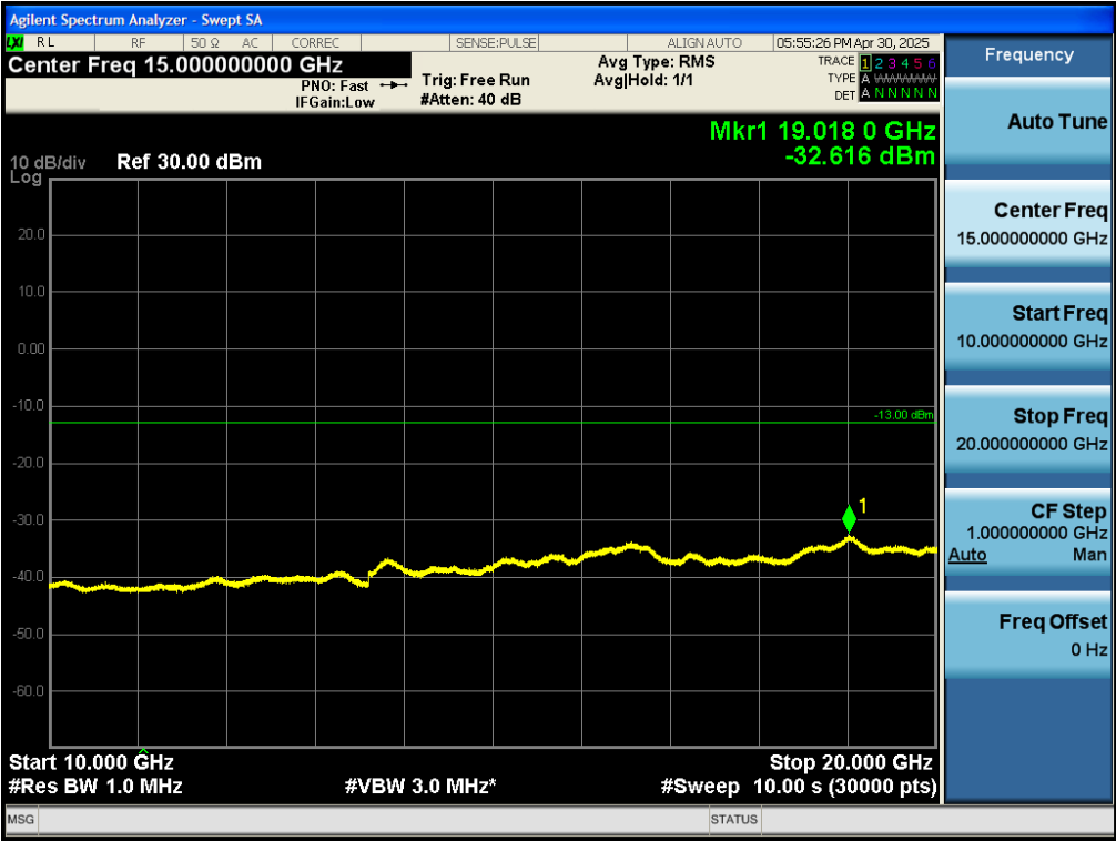
Test_Graph_band66_1745MHz_20M_QPSK_100RB#LOW_10G_20.0G_TX
