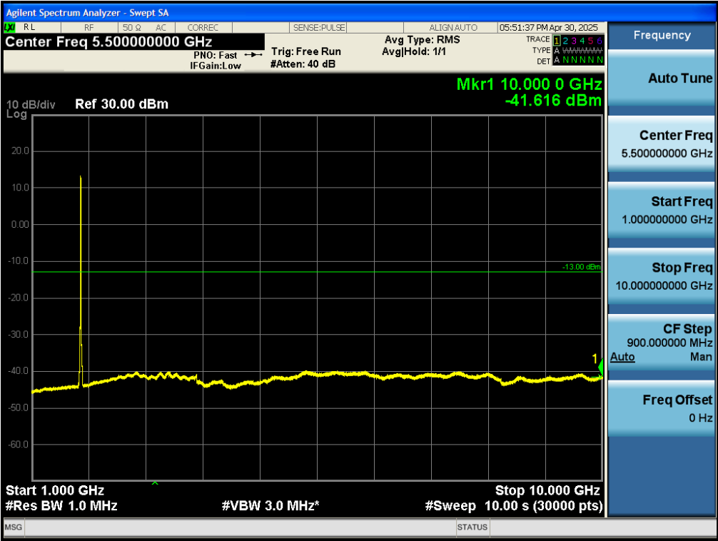
Test_Graph_band66_1775MHz_10M_QPSK_50RB#LOW_1G_10G_TX
