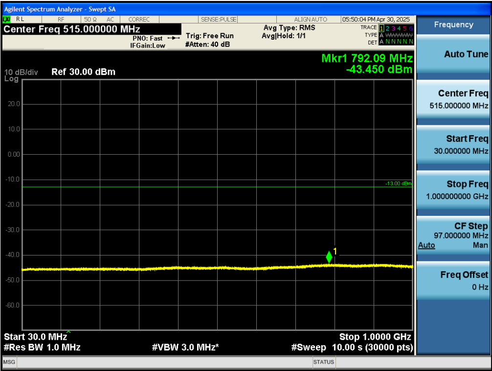
Test_Graph_band66_1715MHz_10M_QPSK_50RB#LOW_30M_1G_TX
