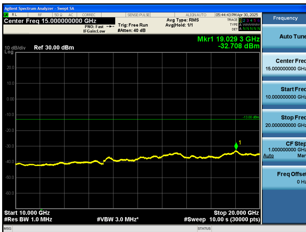
Test_Graph_band66_1745MHz_1.4M_QPSK_6RB#LOW_10G_20.0G_TX
