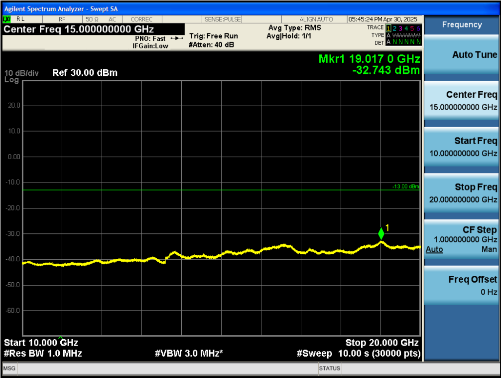
Test_Graph_band66_1779.3MHz_1.4M_QPSK_6RB#LOW_10G_20.0G_TX
