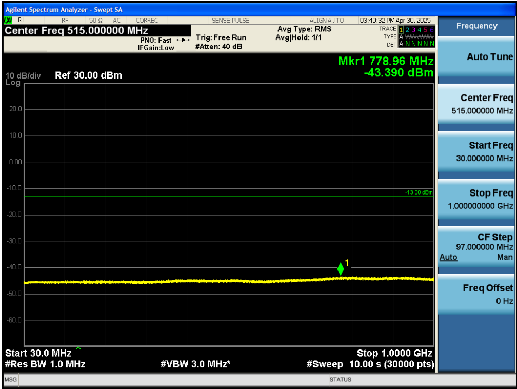
Test_Graph_band25_1882.5MHz_1.4M_QPSK_6RB#LOW_30M_1G_TX
