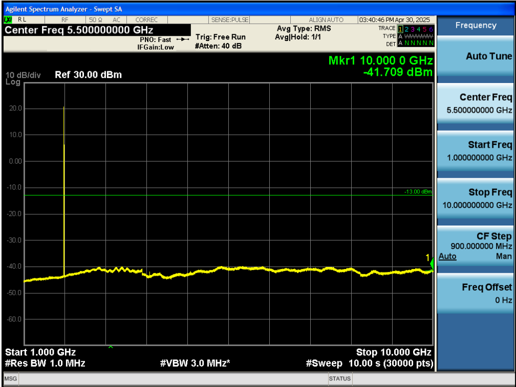
Test_Graph_band25_1882.5MHz_1.4M_QPSK_6RB#LOW_1G_10G_TX
