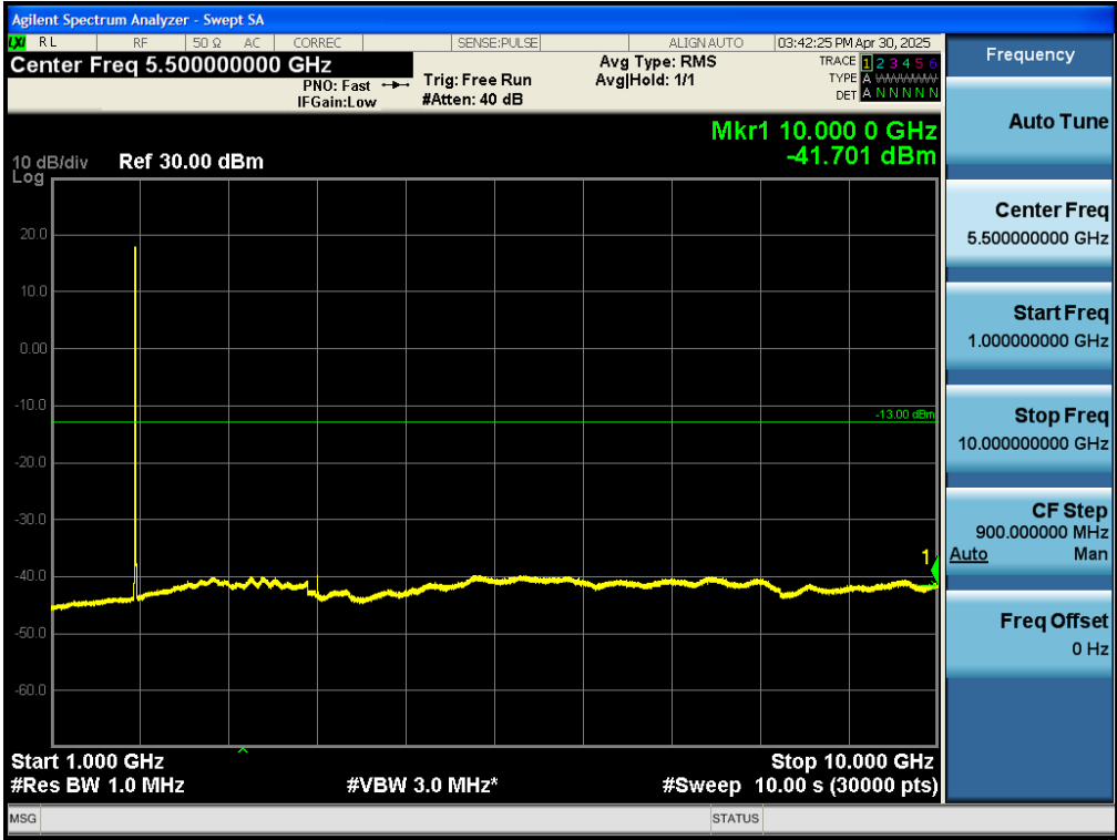
Test_Graph_band25_1851.5MHz_3M_QPSK_15RB#LOW_1G_10G_TX
