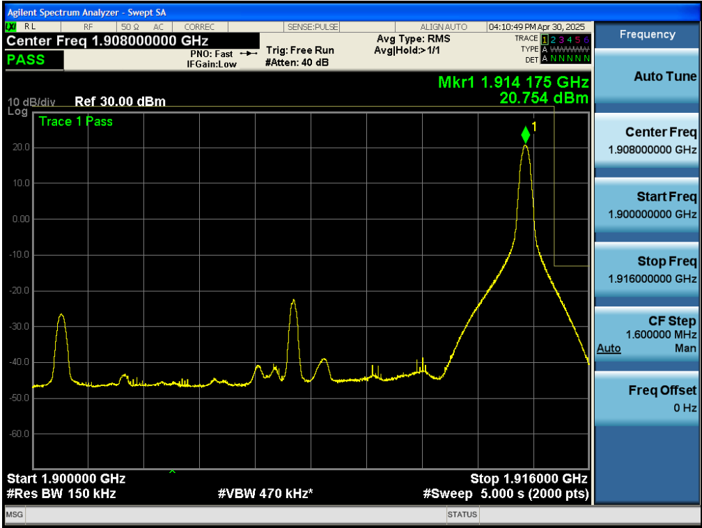
Test_Graph_band25_1907.5MHz_15M_16QAM_1RB#HIGH_Band edge
