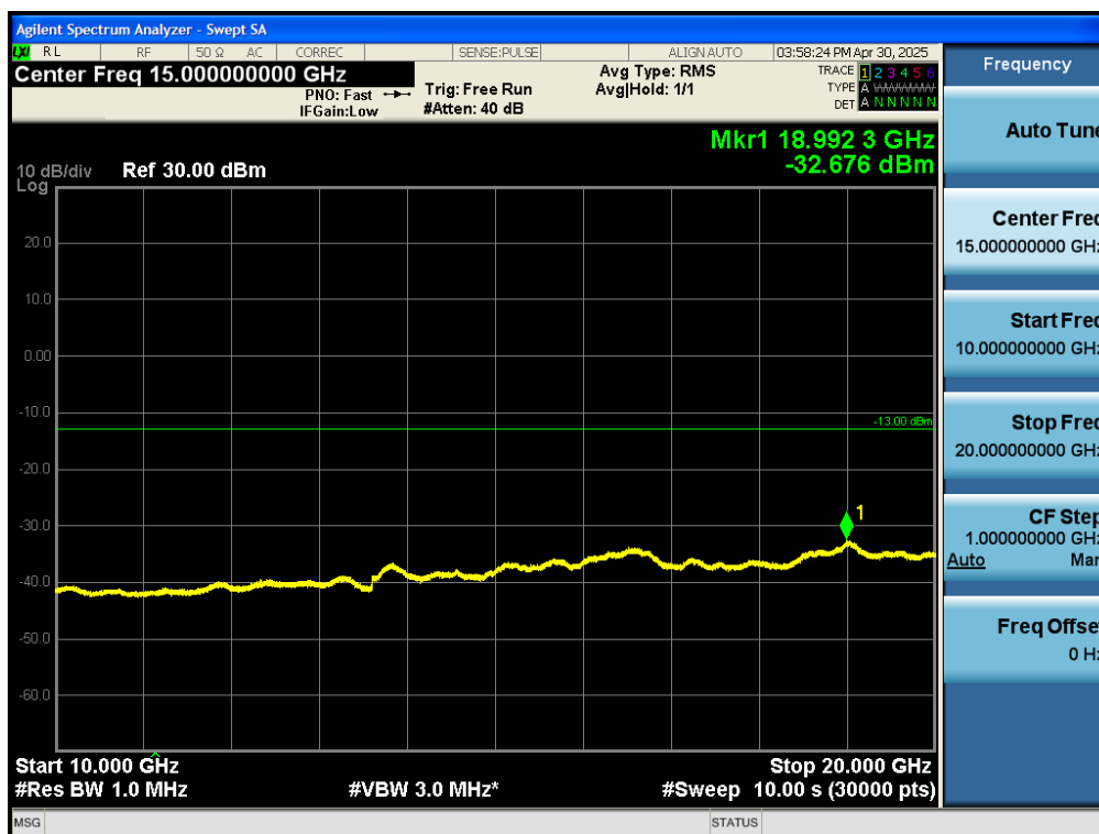
Test_Graph_band25_1882.5MHz_20M_QPSK_100RB#LOW_10G_20.0G_TX
