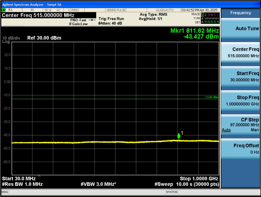
Test_Graph_band25_1882.5MHz_3M_QPSK_15RB#LOW_30M_1G_TX
