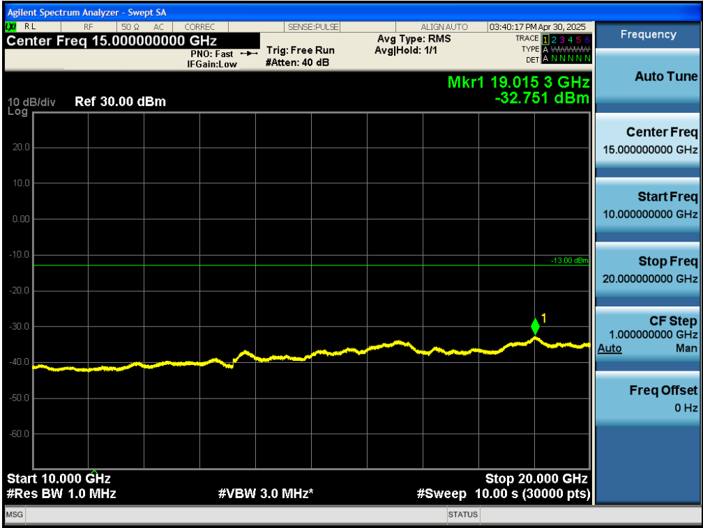
Test_Graph_band25_1850.7MHz_1.4M_QPSK_6RB#LOW_10G_20.0G_TX
