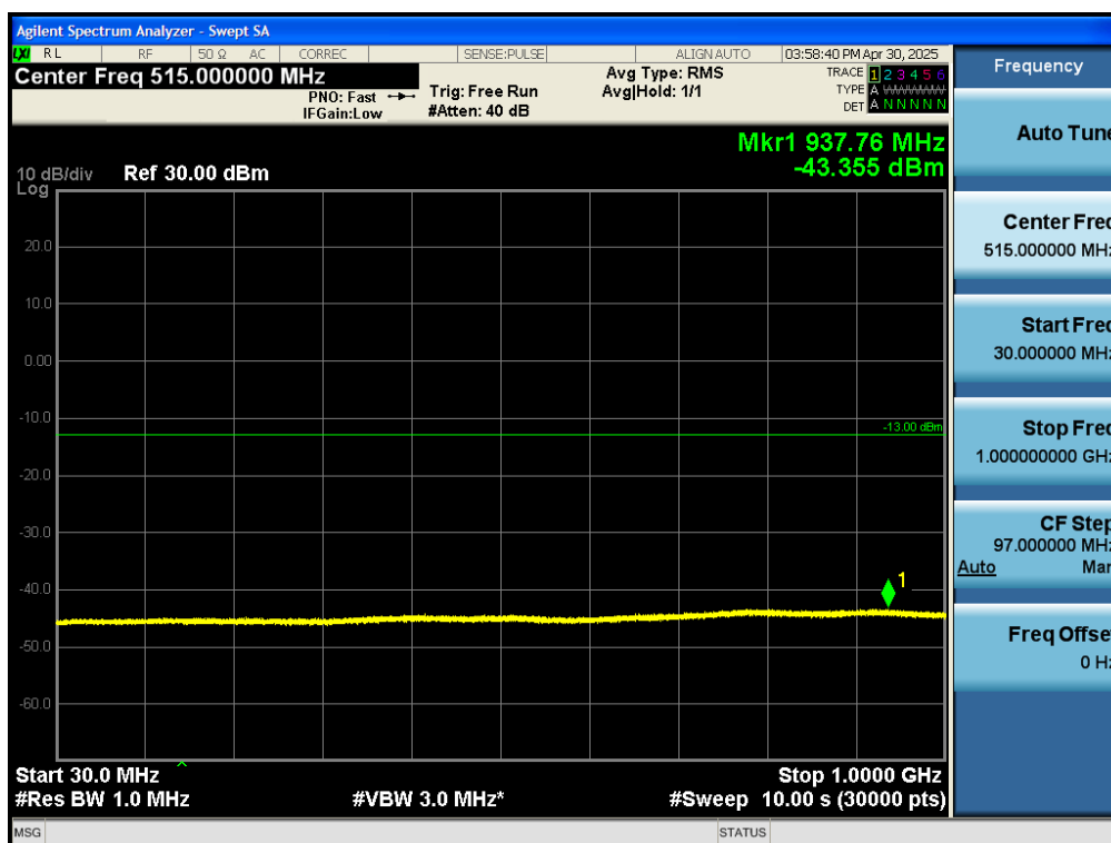
Test_Graph_band25_1905MHz_20M_QPSK_100RB#LOW_30M_1G_TX
