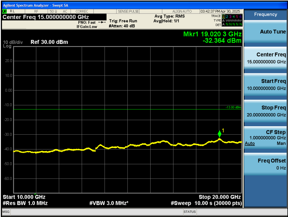
Test_Graph_band25_1851.5MHz_3M_QPSK_15RB#LOW_10G_20.0G_TX
