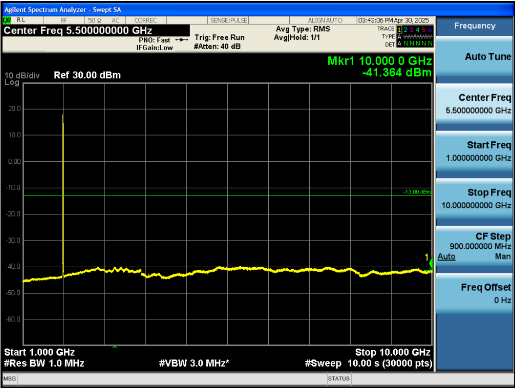
Test_Graph_band25_1882.5MHz_3M_QPSK_15RB#LOW_1G_10G_TX
