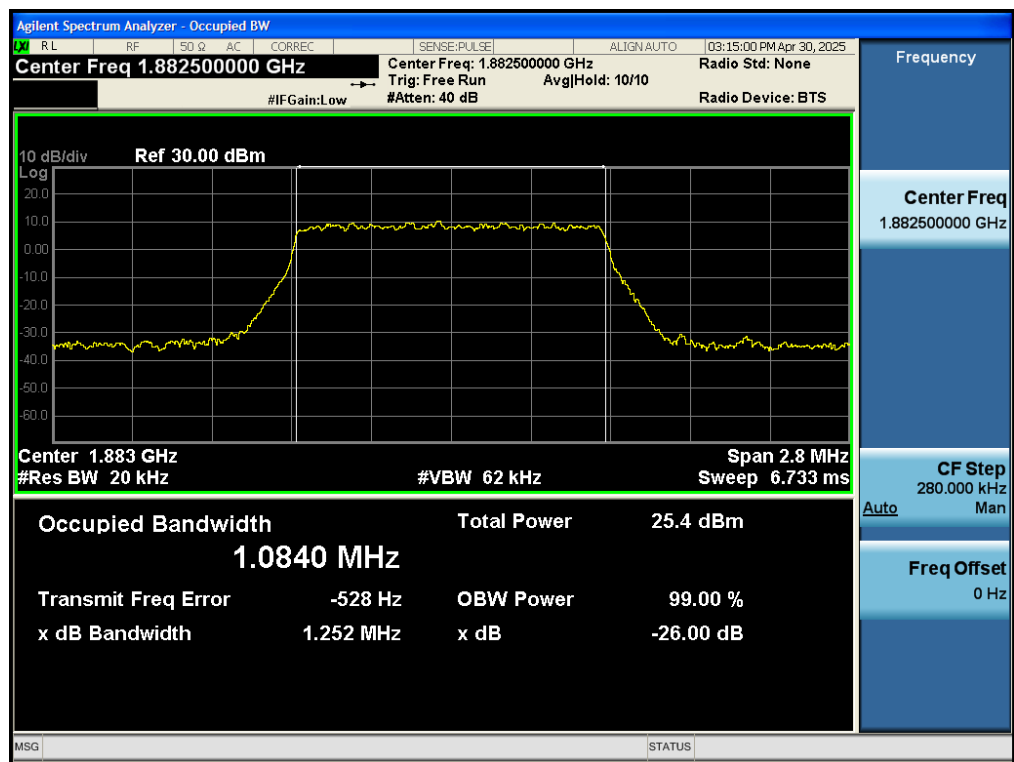
Test_Graph_band25_1882.5MHz_1.4M_QPSK_6RB#LOW_OBW&EBW
