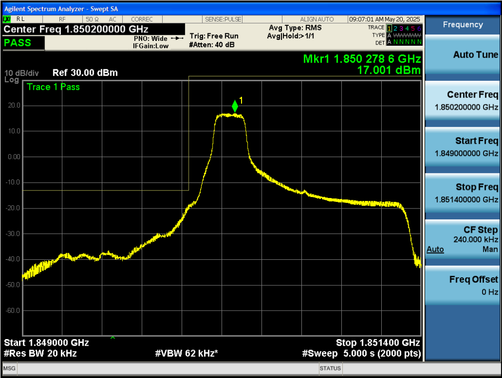
Test_Graph_band25_1850.7MHz_1.4M_QPSK_1RB#LOW_Band edge
