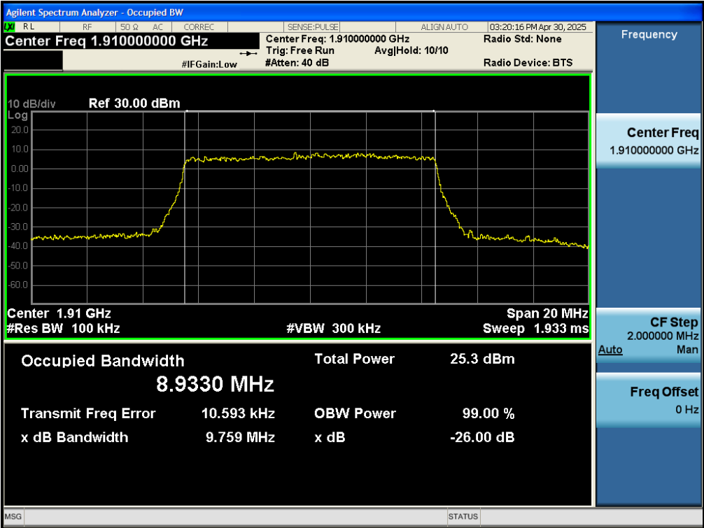
Test_Graph_band25_1910MHz_10M_16QAM_50RB#LOW_OBW&EBW
