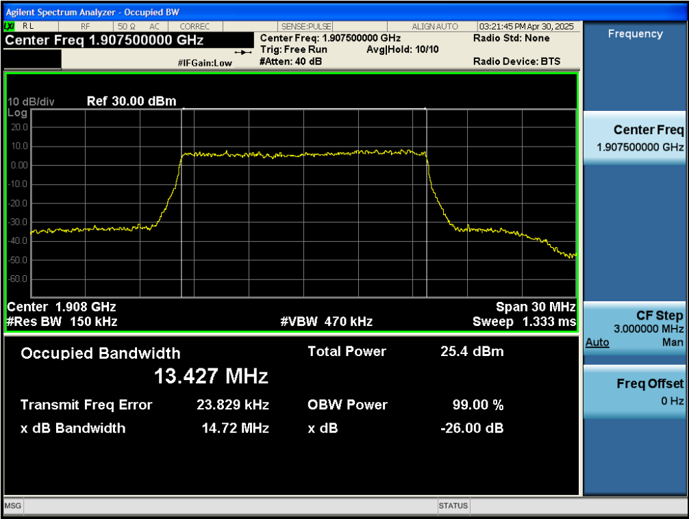
Test_Graph_band25_1907.5MHz_15M_16QAM_75RB#LOW_OBW&EBW
