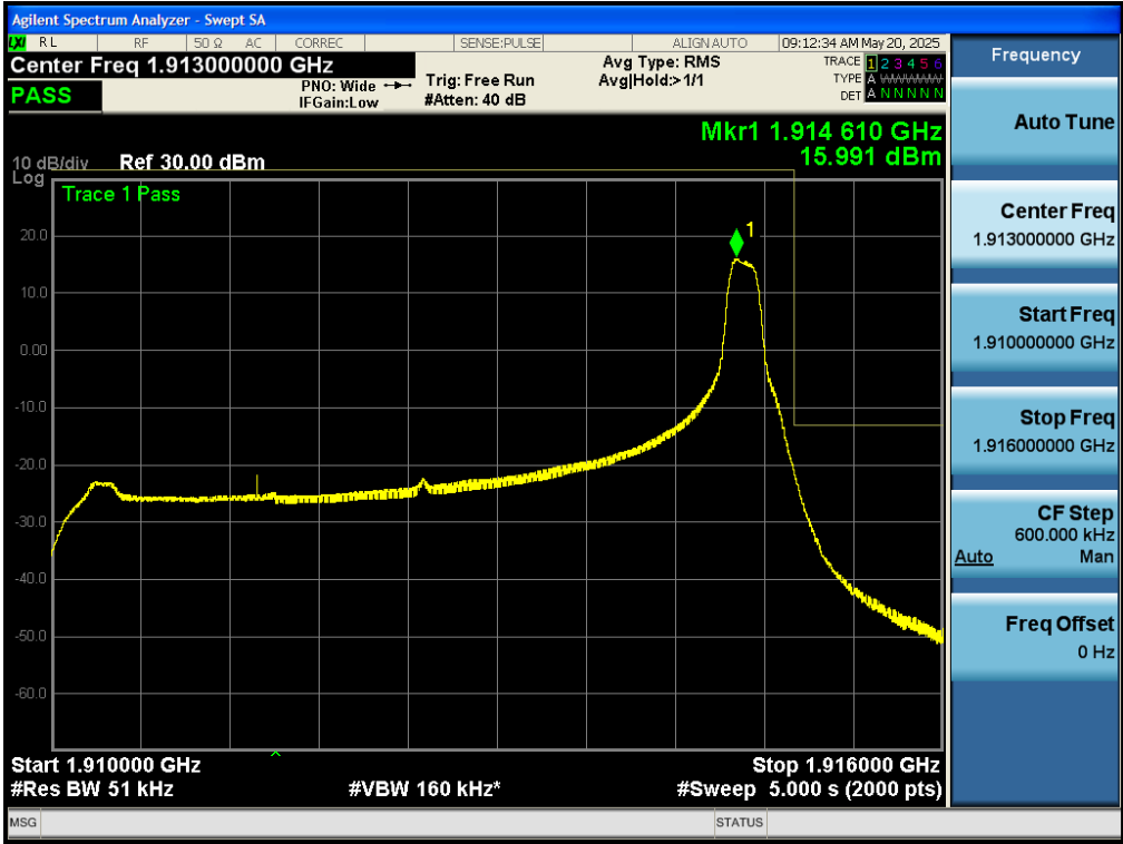
Test_Graph_band25_1912.5MHz_5M_QPSK_1RB#HIGH_Band edge
