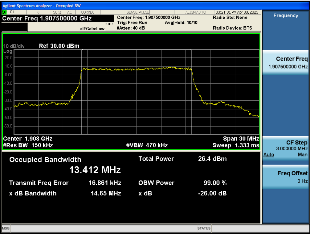
Test_Graph_band25_1907.5MHz_15M_QPSK_75RB#LOW_OBW&EBW
