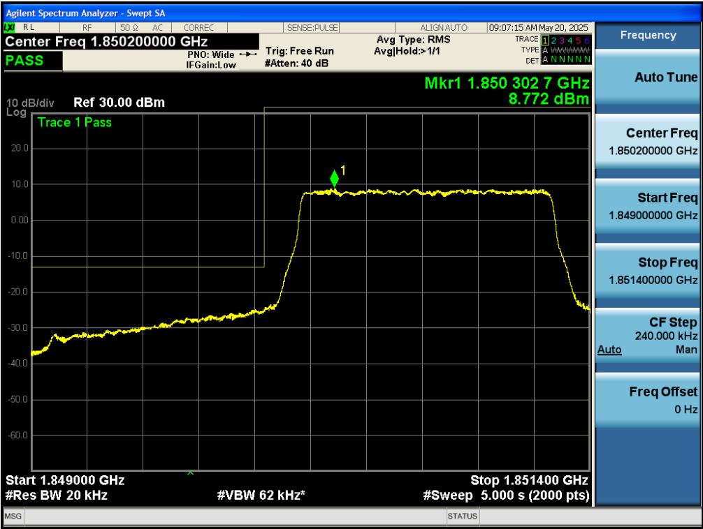
Test_Graph_band25_1850.7MHz_1.4M_QPSK_6RB#LOW_Band edge
