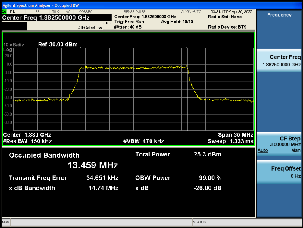
Test_Graph_band25_1882.5MHz_15M_16QAM_75RB#LOW_OBW&EBW
