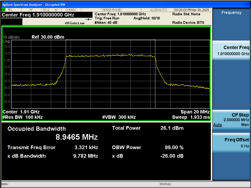
Test_Graph_band25_1910MHz_10M_QPSK_50RB#LOW_OBW&EBW
