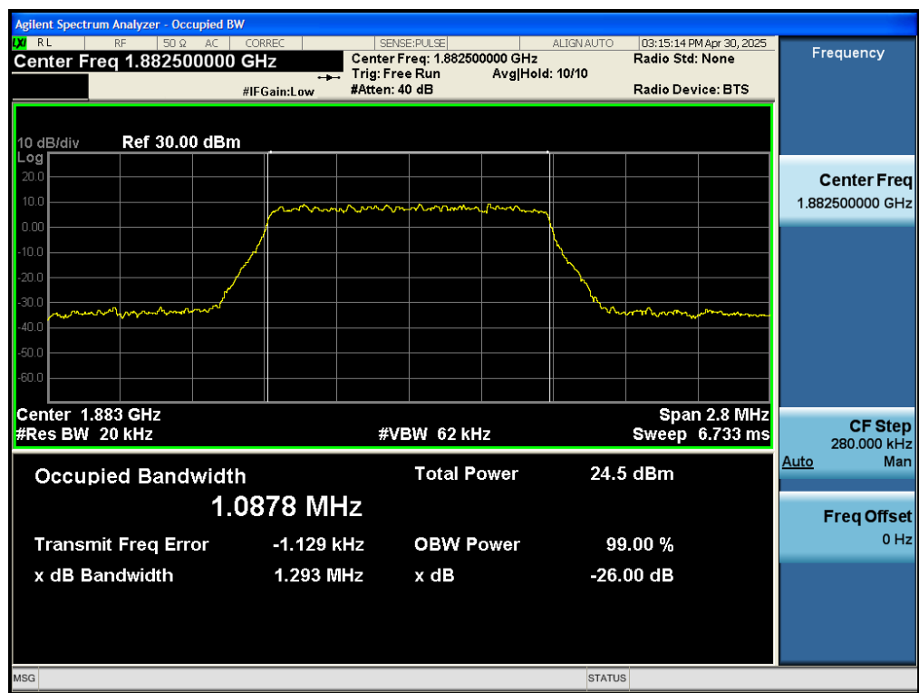
Test_Graph_band25_1882.5MHz_1.4M_16QAM_6RB#LOW_OBW&EBW
