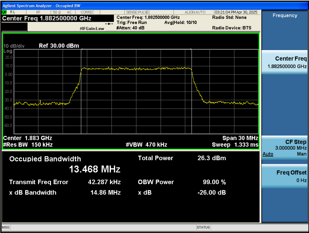
Test_Graph_band25_1882.5MHz_15M_QPSK_75RB#LOW_OBW&EBW
