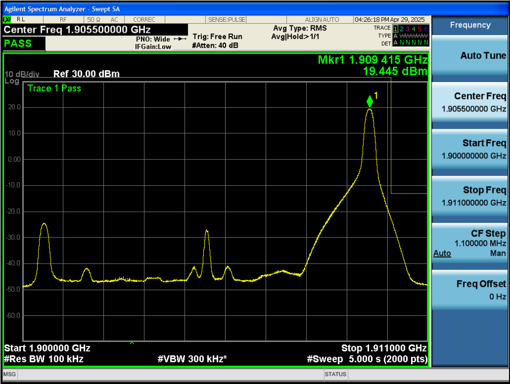
Test_Graph_band2_1905MHz_10M_16QAM_1RB#HIGH_Band edge
