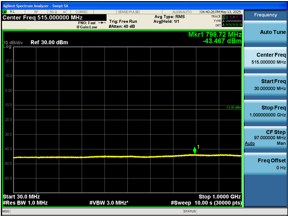
Test_Graph_band2_1850.7MHz_1.4M_QPSK_6RB#LOW_30M_1G_TX
