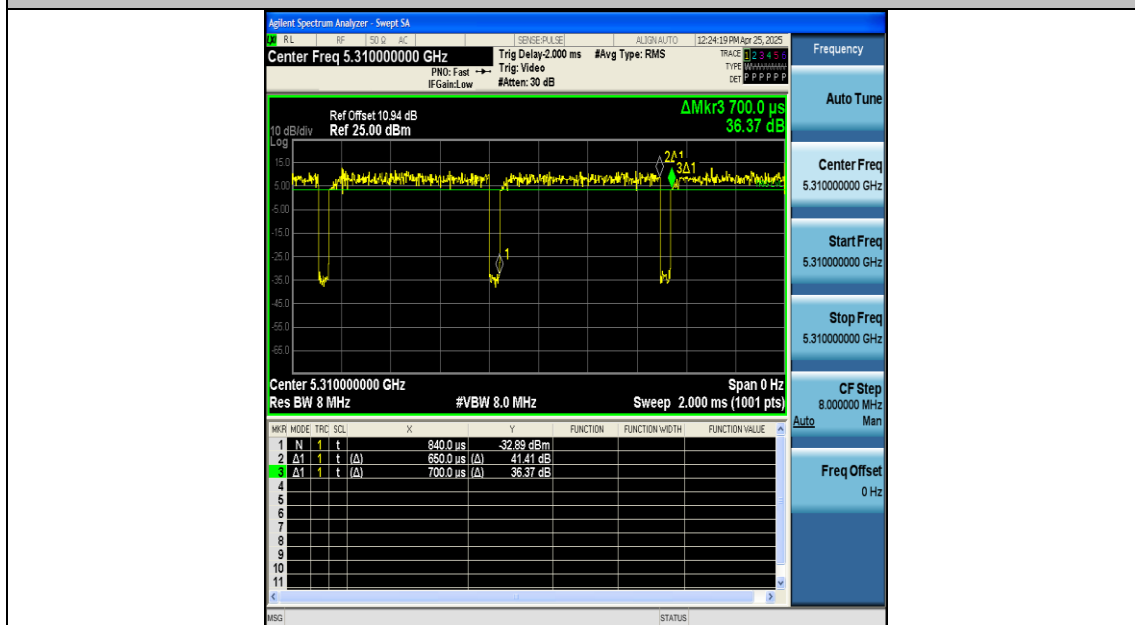
NTNV-11N40SISO-Ant1-5310
