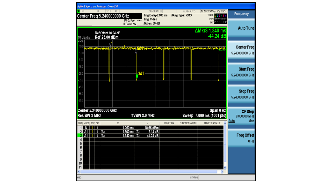
NTNV-11N20SISO-Ant1-5240
