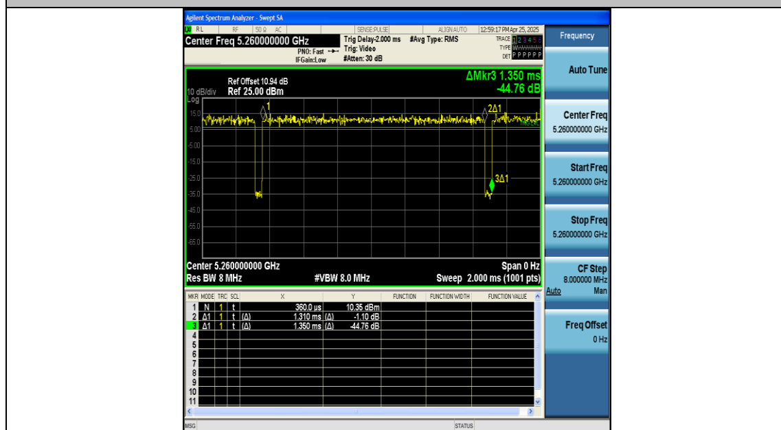
NTNV-11AC20SISO-Ant1-5260
