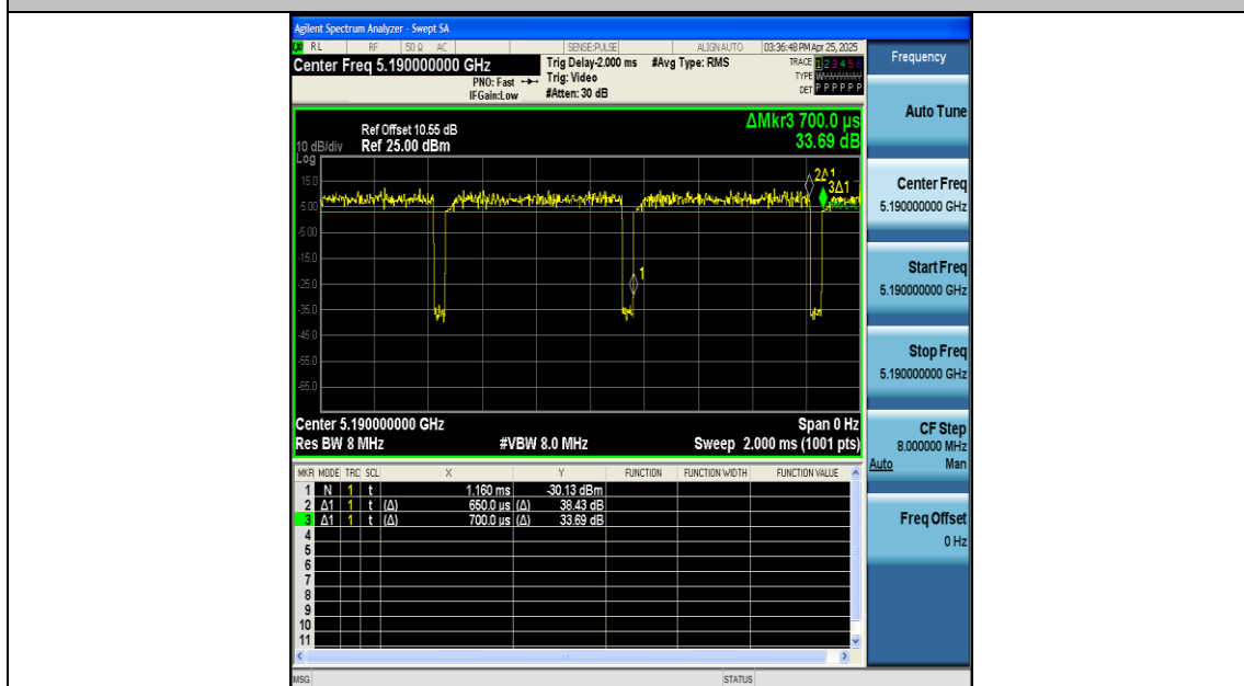
NTNV-11AC40SISO-Ant1-5190
