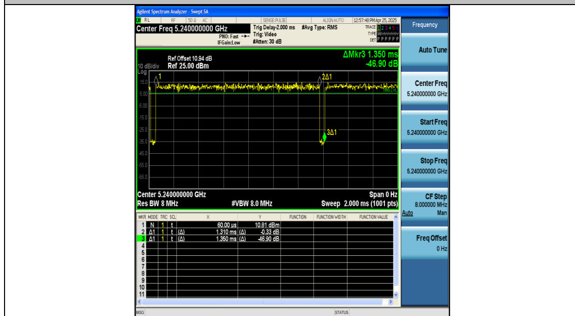
NTNV-11AC20SISO-Ant1-5240
