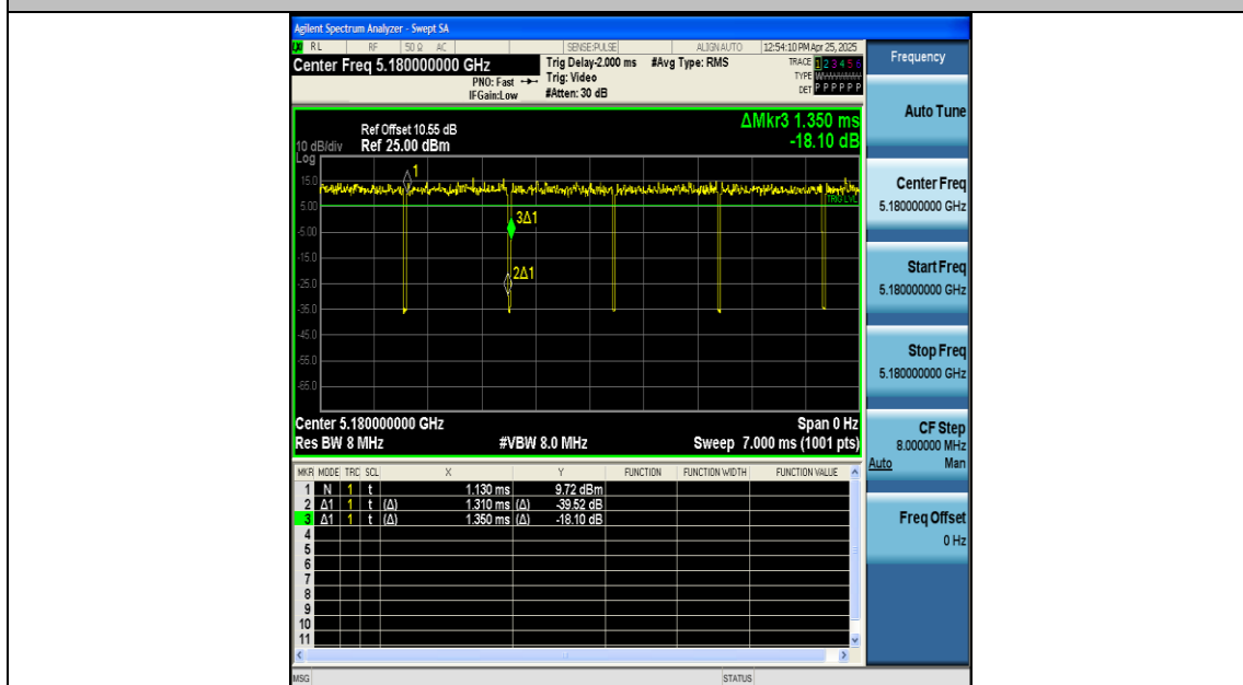
NTNV-11AC20SISO-Ant1-5180
