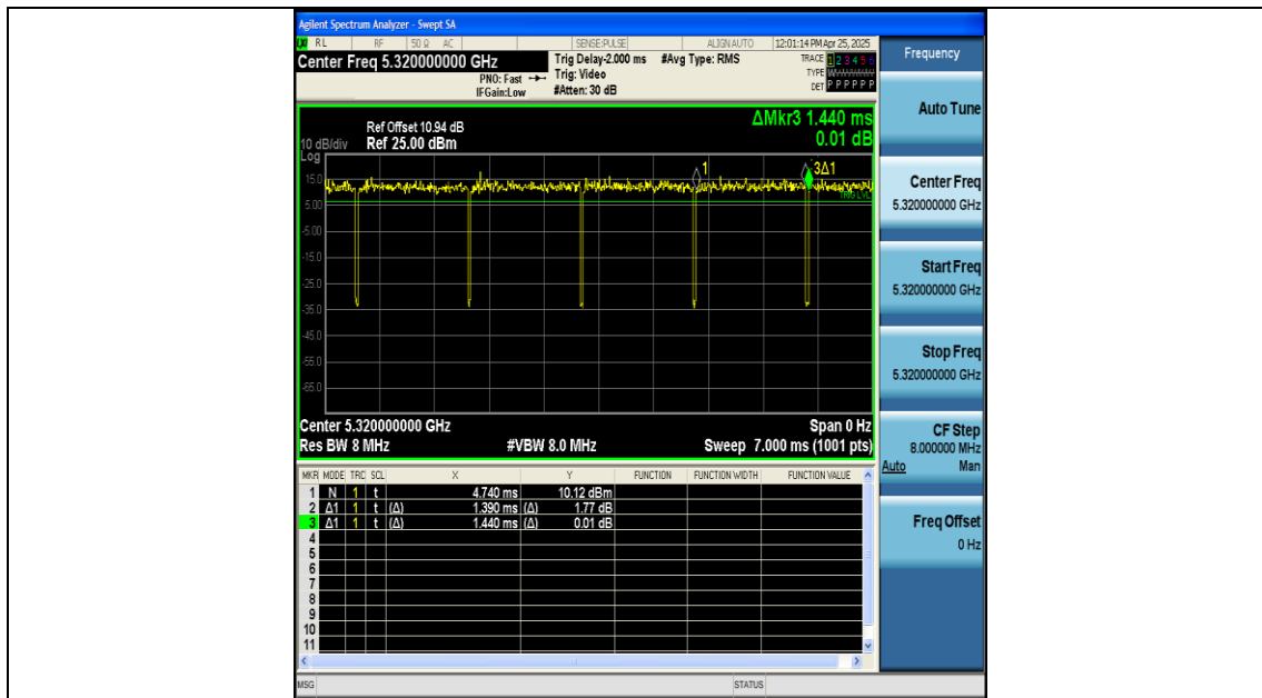
NTNV-11A-Ant1-5320
