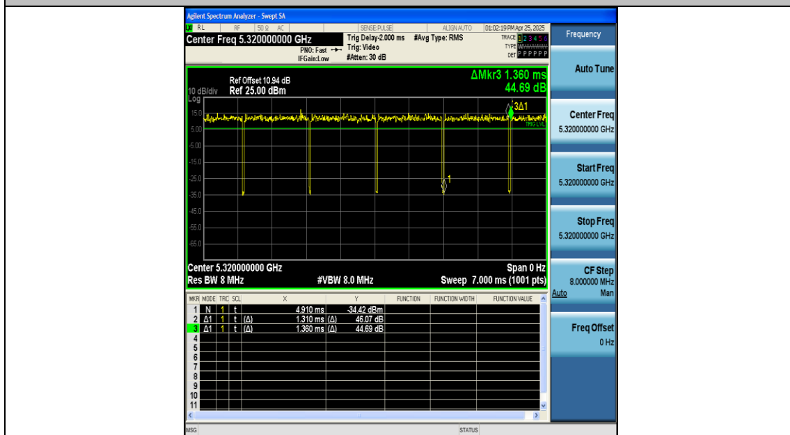
NTNV-11AC20SISO-Ant1-5320
