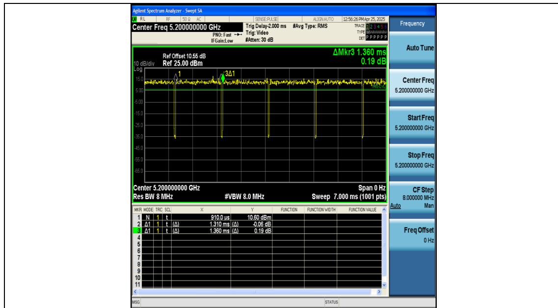
NTNV-11AC20SISO-Ant1-5200
