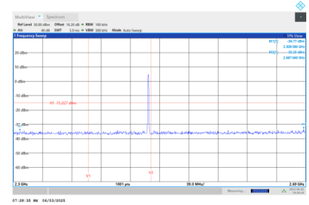
Bandedge-CH39
