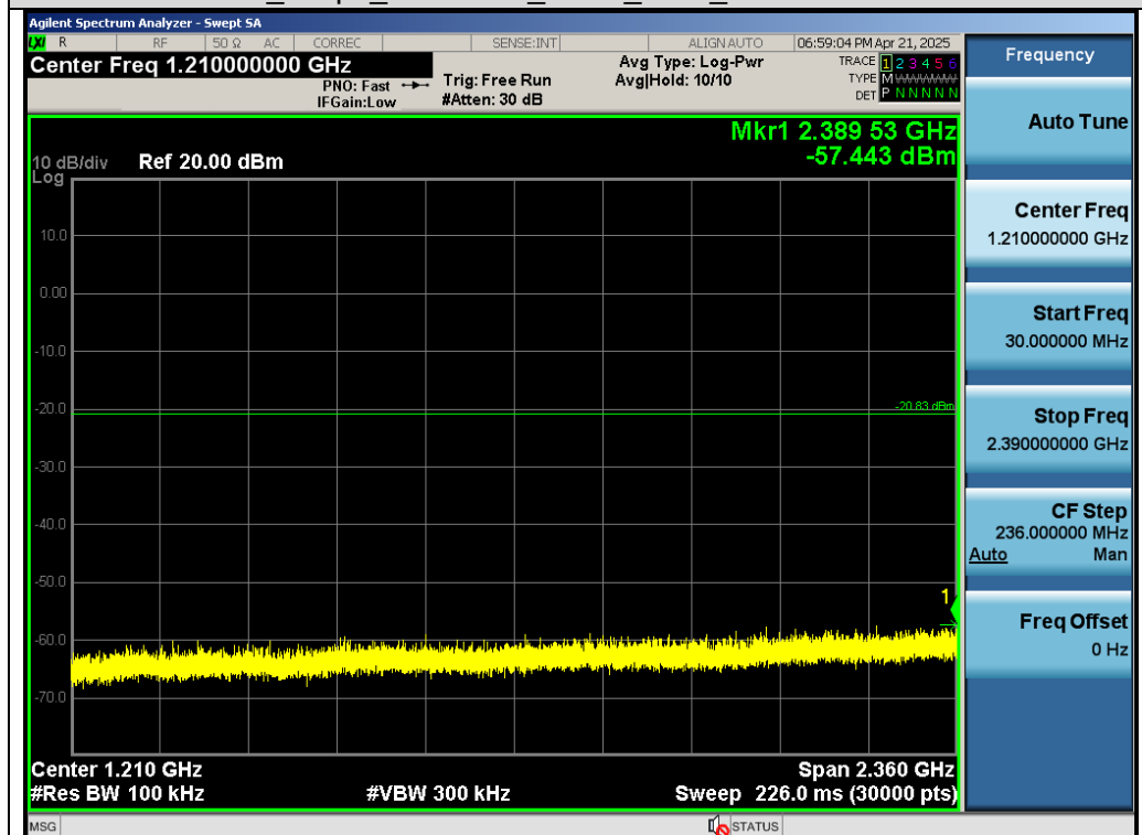
Test_Graph_SRD 2.4G_ANT1_2402_Lower Band Emissions
