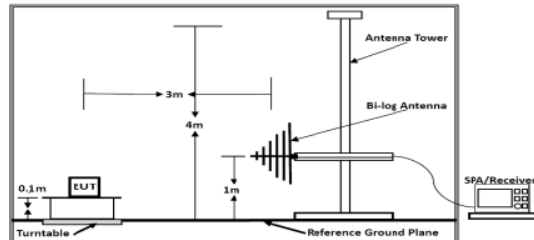
Below 1GHz Figure 2. 30MHz to 1GHz
