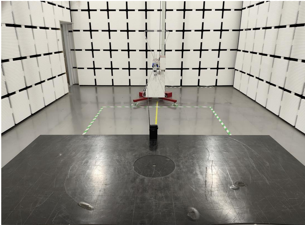
Radiation Emissions Test (<1G)
