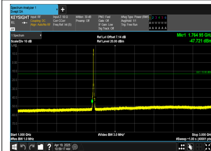
Band66-5MHz-16QAM-132647-25RB#0-1000~3000-PASS
