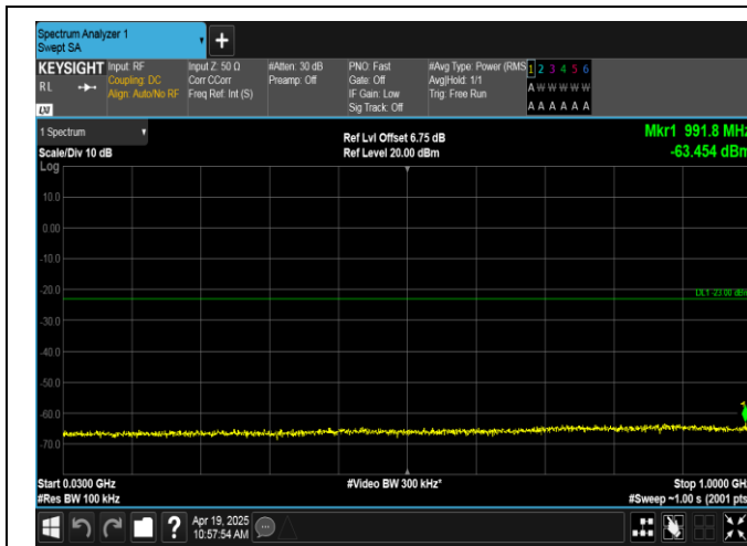
Band66-5MHz-QPSK-132647-25RB#0-30~1000-PASS
