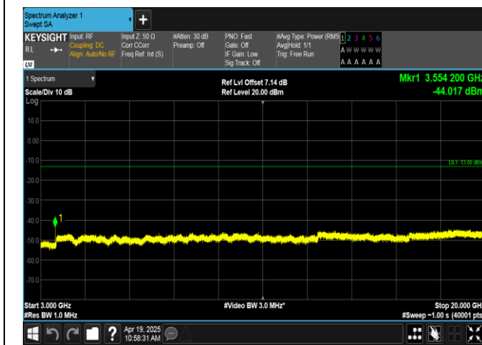
Band66-5MHz-QPSK-132647-25RB#0-3000~20000-PASS
