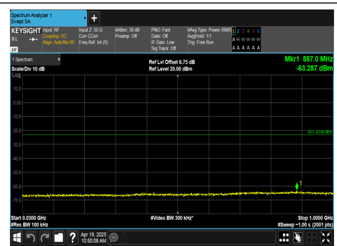
Band66-5MHz-16QAM-132322-1RB#24-30~1000-PASS
