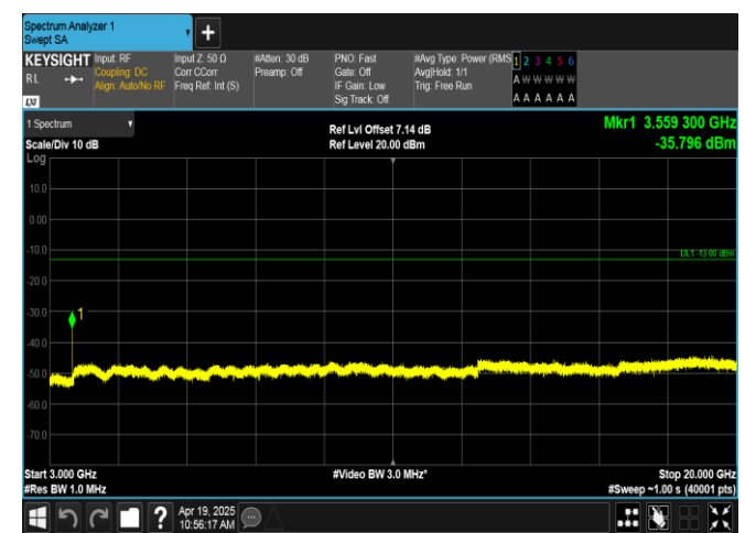
Band66-5MHz-QPSK-132647-1RB#24-3000~20000-PASS
