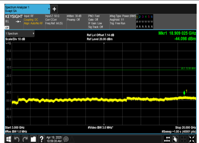
Band66-5MHz-16QAM-132647-25RB#0-3000~20000-PASS
