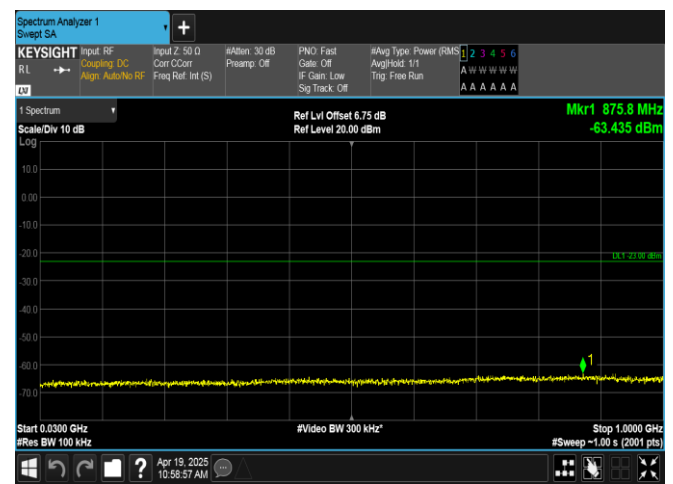
Band66-5MHz-16QAM-132647-25RB#0-30~1000-PASS
