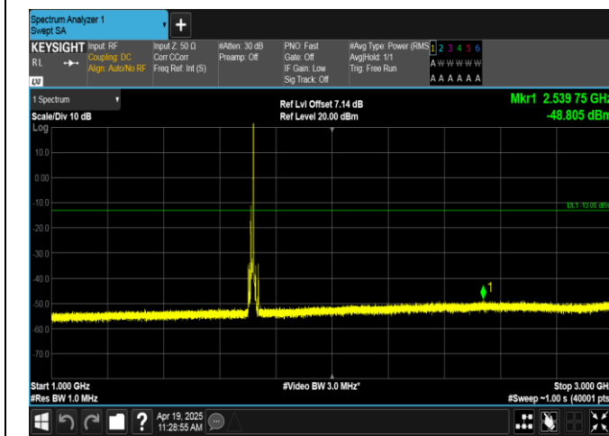
Band66-10MHz-QPSK-132022-1RB#49-1000~3000-PASS
