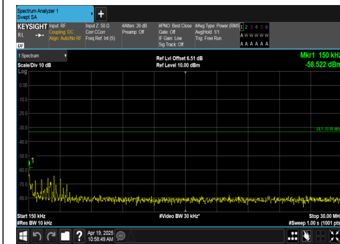
Band66-5MHz-16QAM-132647-25RB#0-0.15~30-PASS
