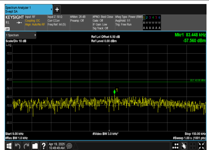
Band66-5MHz-16QAM-132322-1RB#24-0.009~0.15-PASS
