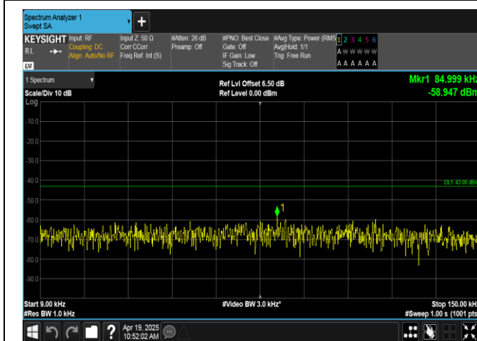
Band66-5MHz-16QAM-132322-25RB#0-0.009~0.15-PASS
