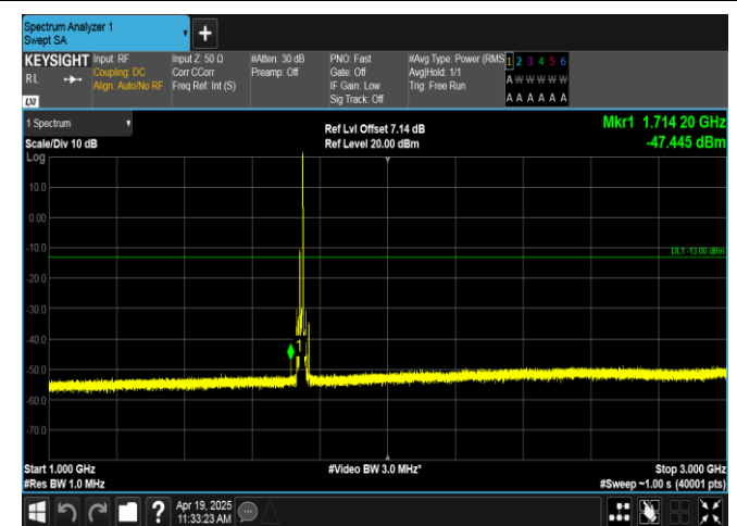
Band66-10MHz-QPSK-132322-1RB#49-1000~3000-PASS
