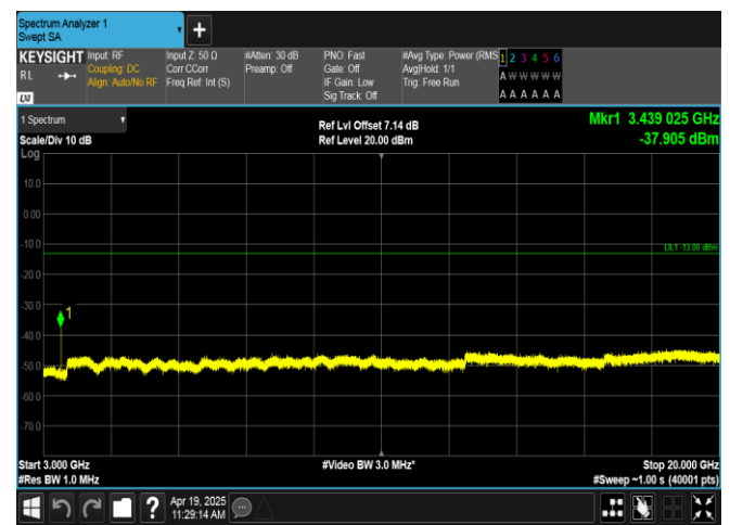
Band66-10MHz-QPSK-132022-1RB#49-3000~20000-PASS
