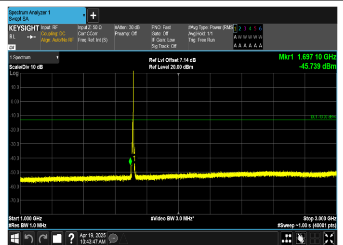
Band66-5MHz-16QAM-131997-1RB#24-1000~3000-PASS
