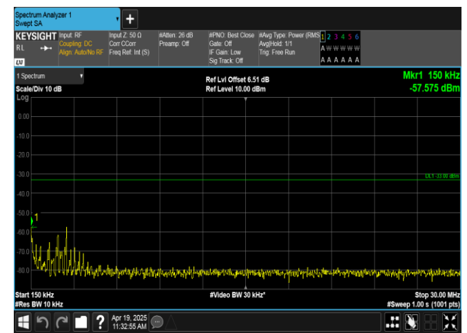
Band66-10MHz-QPSK-132322-1RB#49-0.15~30-PASS
