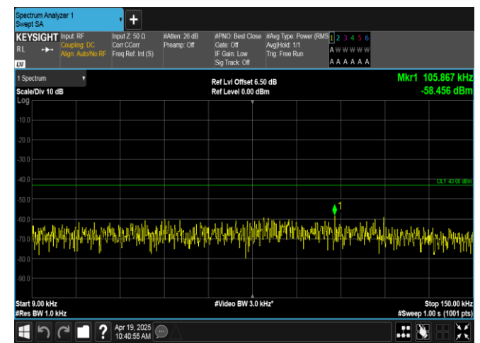
Band66-5MHz-16QAM-131997-1RB#0-0.009~0.15-PASS
