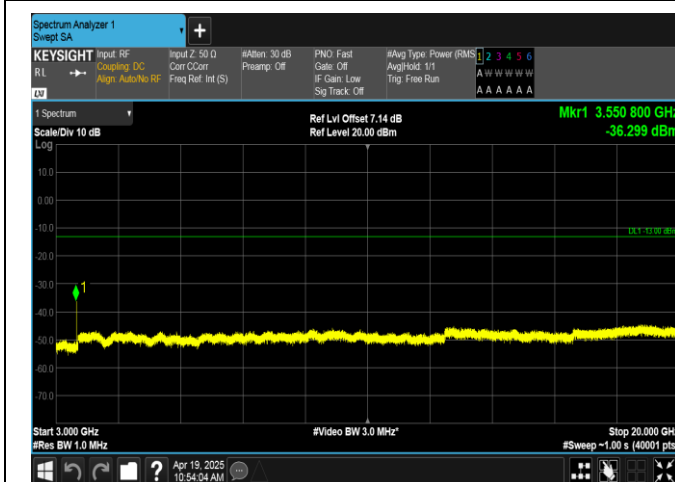
Band66-5MHz-QPSK-132647-1RB#0-3000~20000-PASS
