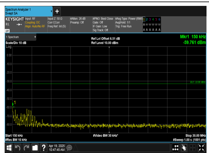
Band66-5MHz-16QAM-132322-1RB#0-0.15~30-PASS
