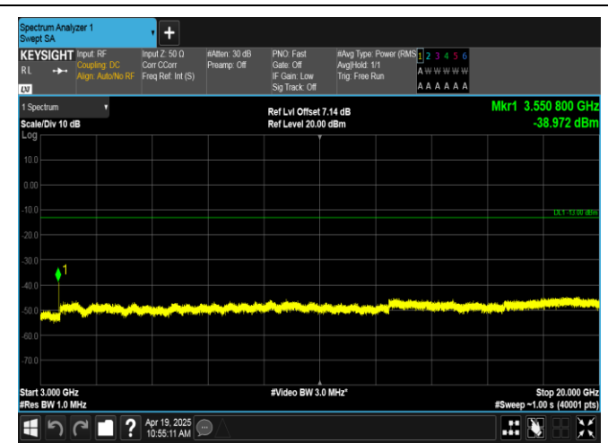
Band66-5MHz-16QAM-132647-1RB#0-3000~20000-PASS
