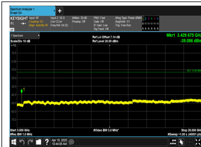
Band66-5MHz-16QAM-131997-1RB#24-3000~20000-PASS
