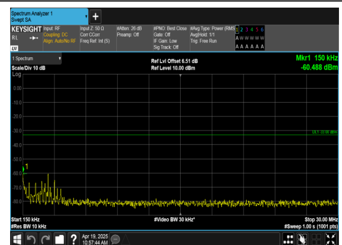
Band66-5MHz-QPSK-132647-25RB#0-0.15~30-PASS
