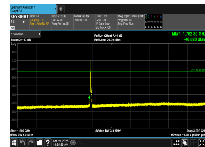
Band66-5MHz-QPSK-132647-1RB#24-1000~3000-PASS
