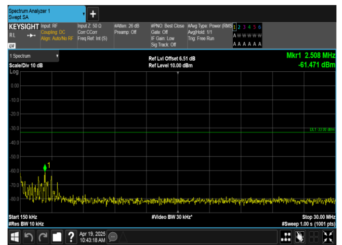
Band66-5MHz-16QAM-131997-1RB#24-0.15~30-PASS
