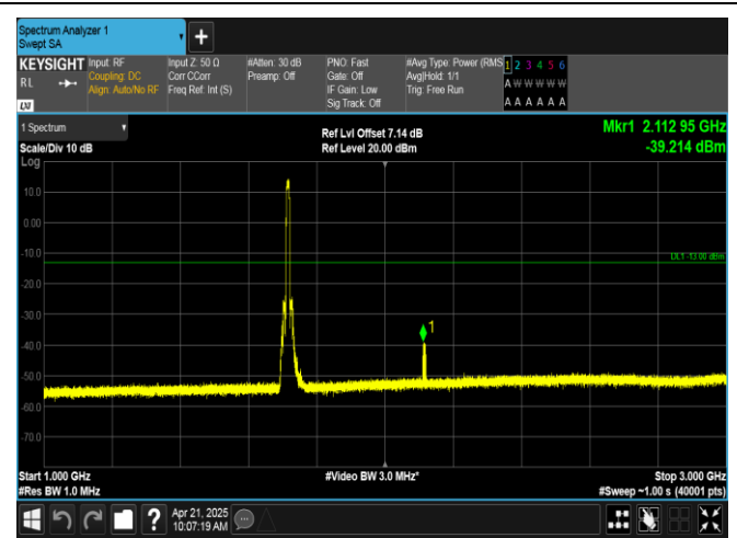
Band66-10MHz-QPSK-132022-50RB#0-1000~3000-PASS
