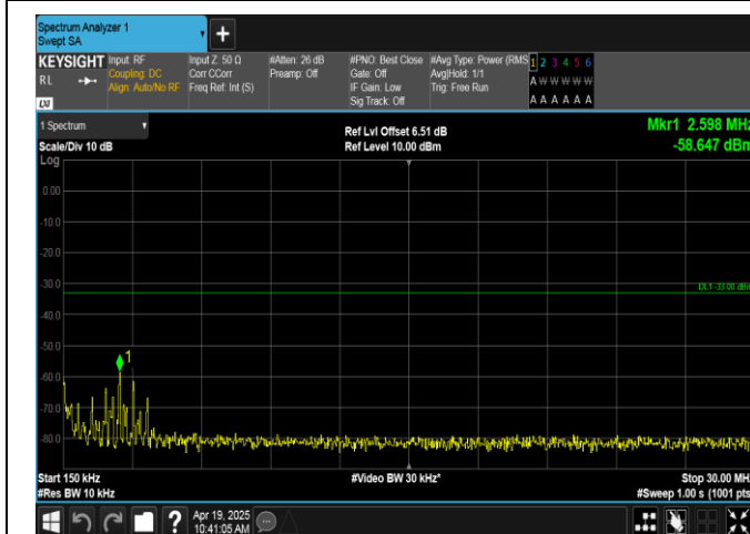
Band66-5MHz-16QAM-131997-1RB#0-0.15~30-PASS
