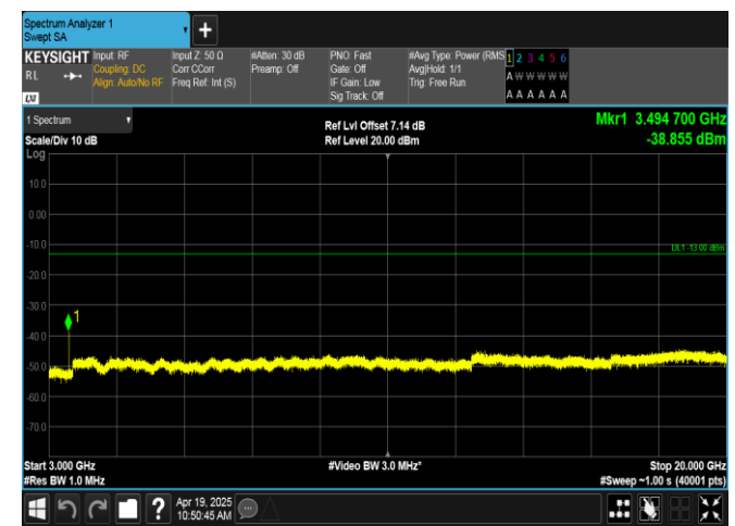
Band66-5MHz-16QAM-132322-1RB#24-3000~20000-PASS
