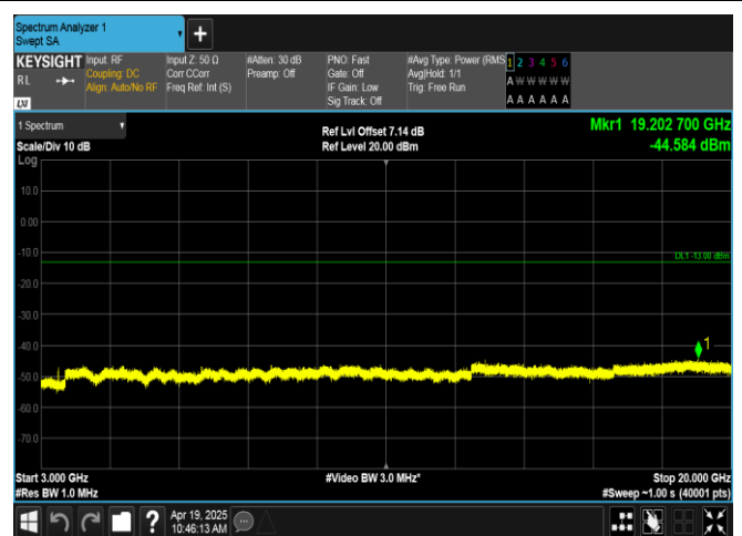
Band66-5MHz-16QAM-131997-25RB#0-3000~20000-PASS
