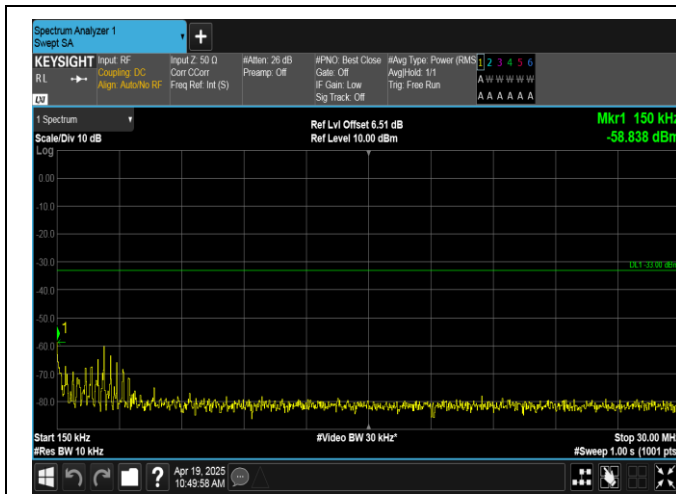
Band66-5MHz-16QAM-132322-1RB#24-0.15~30-PASS
