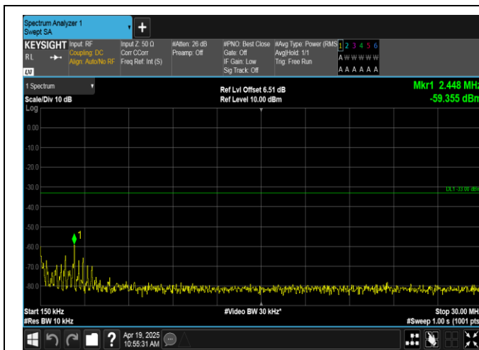
Band66-5MHz-QPSK-132647-1RB#24-0.15~30-PASS
