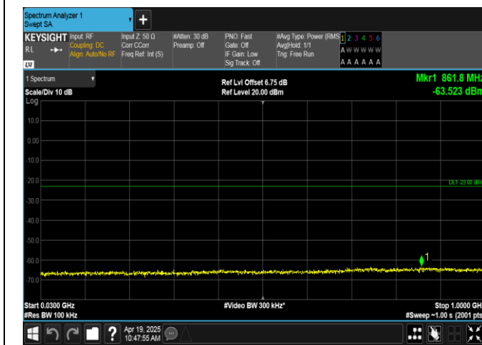
Band66-5MHz-16QAM-132322-1RB#0-30~1000-PASS
