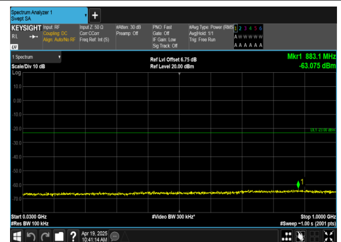
Band66-5MHz-16QAM-131997-1RB#0-30~1000-PASS
