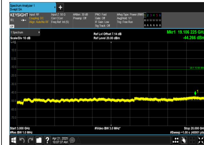
Band66-10MHz-QPSK-132022-50RB#0-3000~20000-PASS
