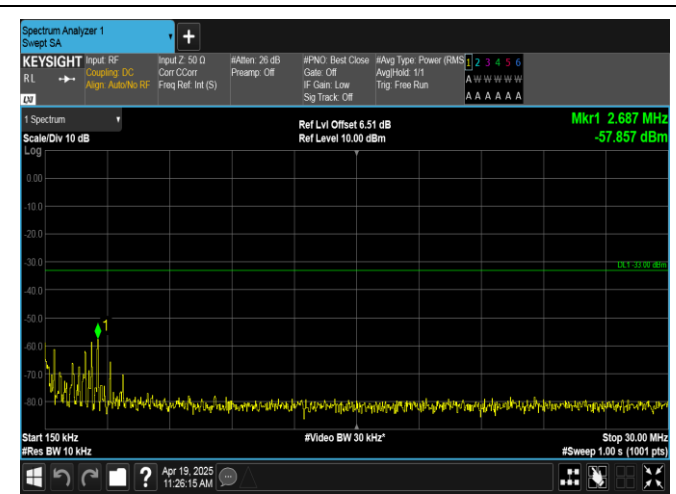
Band66-10MHz-QPSK-132022-1RB#0-0.15~30-PASS
