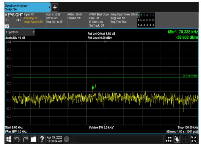
Band66-10MHz-QPSK-132322-1RB#0-0.009~0.15-PASS
