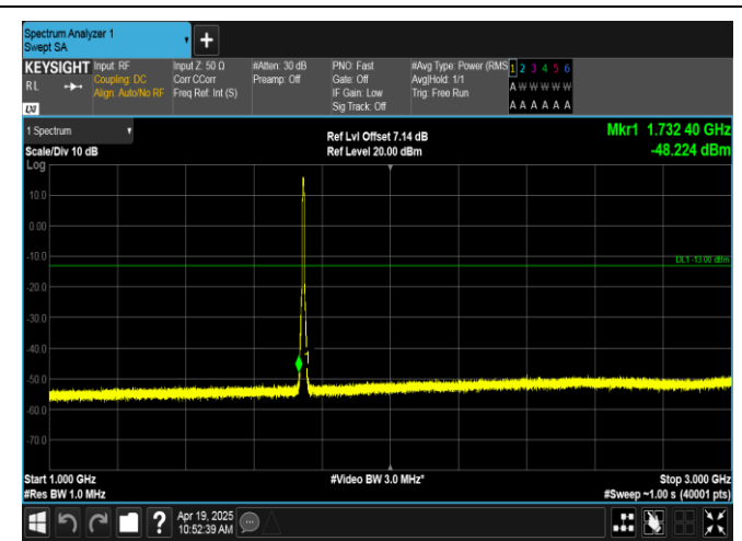
Band66-5MHz-16QAM-132322-25RB#0-1000~3000-PASS
