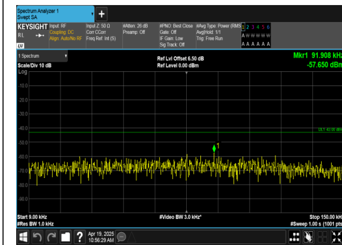
Band66-5MHz-16QAM-132647-1RB#24-0.009~0.15-PASS
