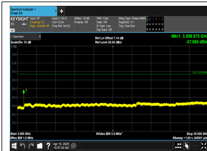
Band66-5MHz-16QAM-132647-1RB#24-3000~20000-PASS
