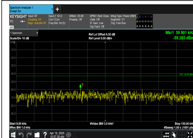
Band66-5MHz-QPSK-132647-25RB#0-0.009~0.15-PASS
