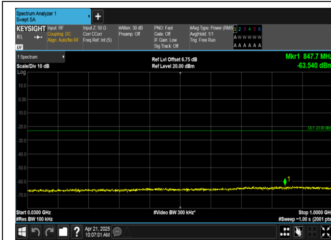
Band66-10MHz-QPSK-132022-50RB#0-30~1000-PASS
