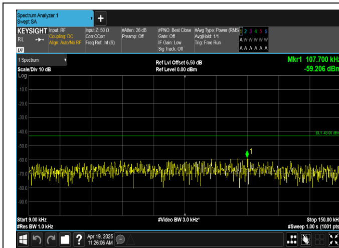
Band66-10MHz-QPSK-132022-1RB#0-0.009~0.15-PASS
