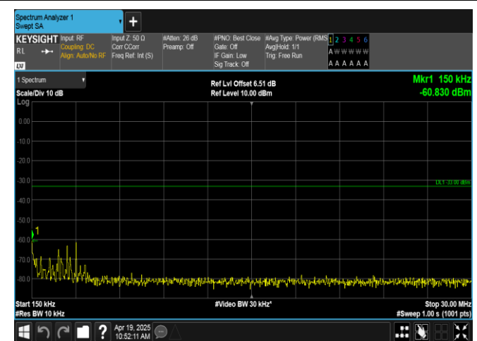
Band66-5MHz-16QAM-132322-25RB#0-0.15~30-PASS
