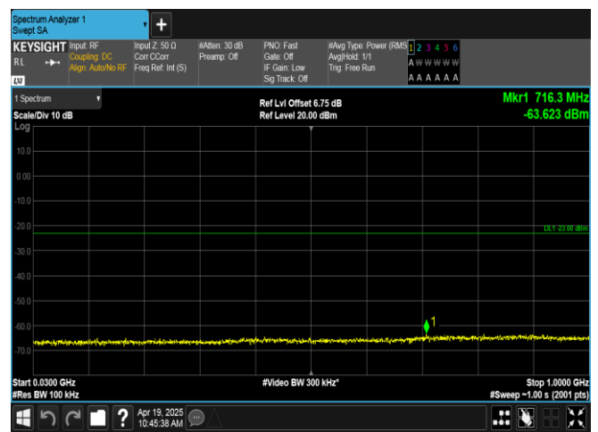
Band66-5MHz-16QAM-131997-25RB#0-30~1000-PASS
