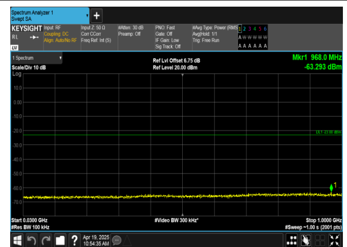
Band66-5MHz-16QAM-132647-1RB#0-30~1000-PASS
