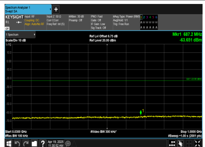
Band66-10MHz-QPSK-132322-1RB#0-30~1000-PASS
