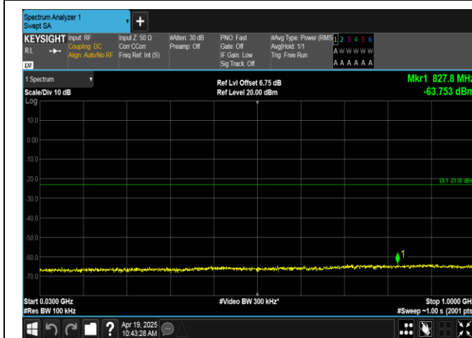
Band66-5MHz-16QAM-131997-1RB#24-30~1000-PASS
