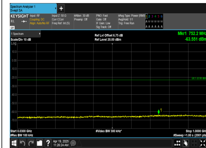
Band66-10MHz-QPSK-132022-1RB#0-30~1000-PASS
