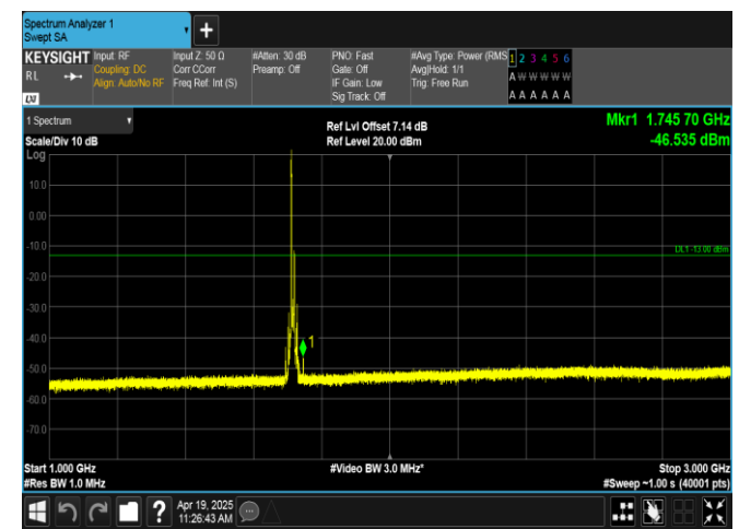
Band66-10MHz-QPSK-132022-1RB#0-1000~3000-PASS
