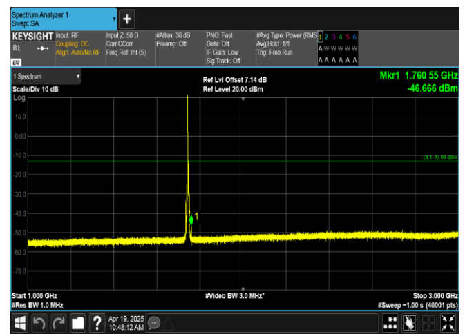
Band66-5MHz-16QAM-132322-1RB#0-1000~3000-PASS
