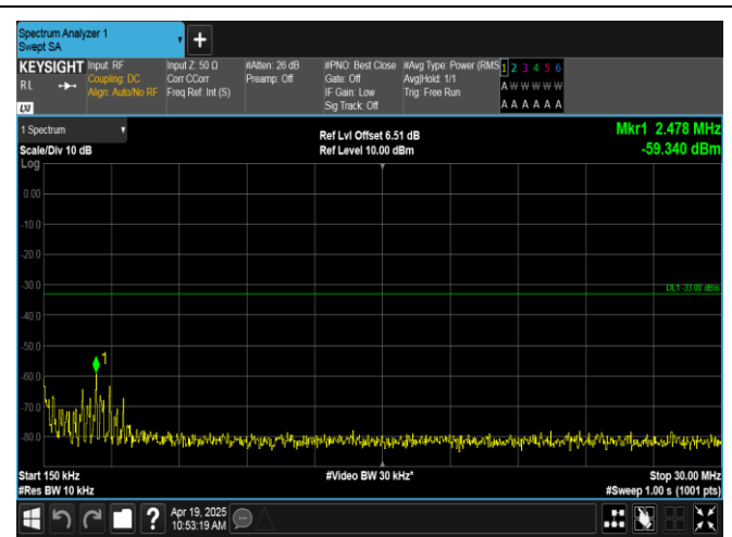
Band66-5MHz-QPSK-132647-1RB#0-0.15~30-PASS
