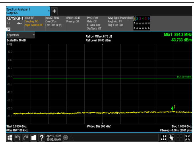
Band66-5MHz-QPSK-132647-1RB#24-30~1000-PASS
