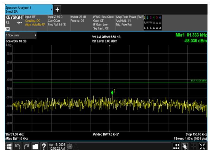
Band66-5MHz-QPSK-132647-1RB#24-0.009~0.15-PASS
