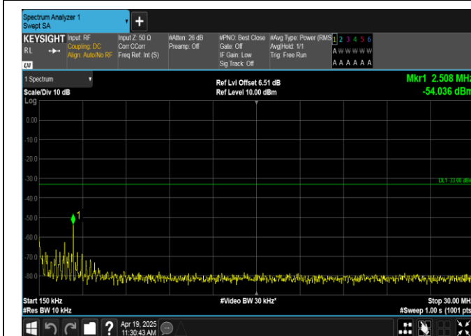
Band66-10MHz-QPSK-132322-1RB#0-0.15~30-PASS
