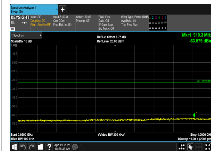
Band66-5MHz-16QAM-132647-1RB#24-30~1000-PASS
