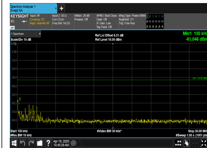
Band66-5MHz-16QAM-131997-25RB#0-0.15~30-PASS
