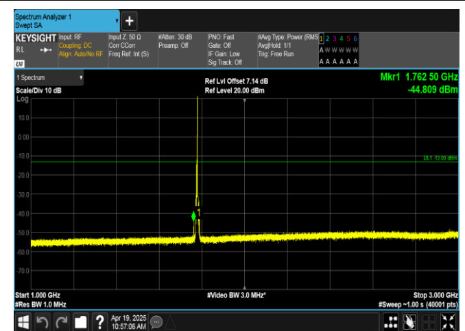
Band66-5MHz-16QAM-132647-1RB#24-1000~3000-PASS
