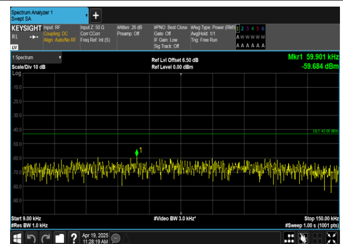
Band66-10MHz-QPSK-132022-1RB#49-0.009~0.15-PASS
