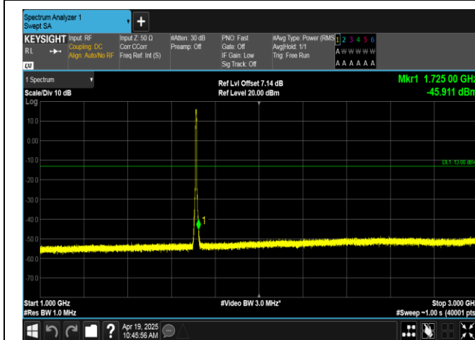
Band66-5MHz-16QAM-131997-25RB#0-1000~3000-PASS
