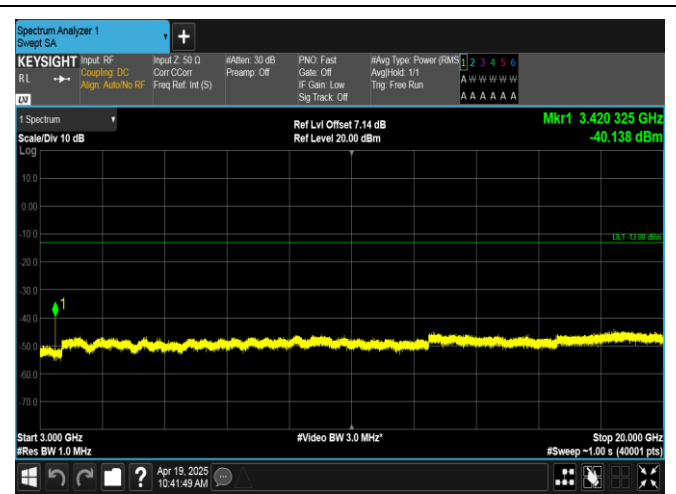
Band66-5MHz-16QAM-131997-1RB#0-3000~20000-PASS
