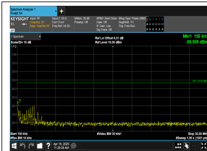
Band66-10MHz-QPSK-132022-1RB#49-0.15~30-PASS
