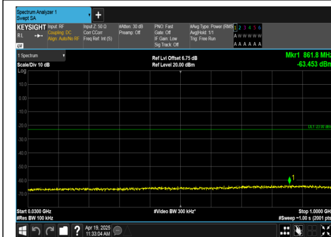
Band66-10MHz-QPSK-132322-1RB#49-30~1000-PASS
