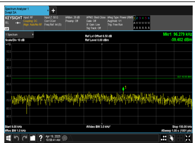
Band66-5MHz-16QAM-132647-25RB#0-0.009~0.15-PASS
