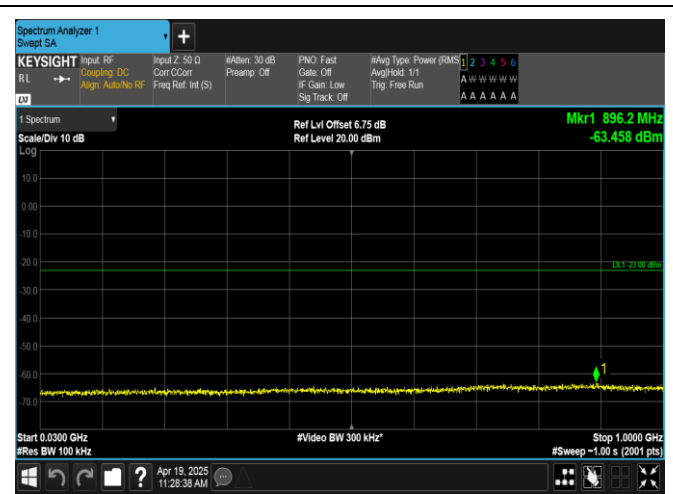
Band66-10MHz-QPSK-132022-1RB#49-30~1000-PASS
