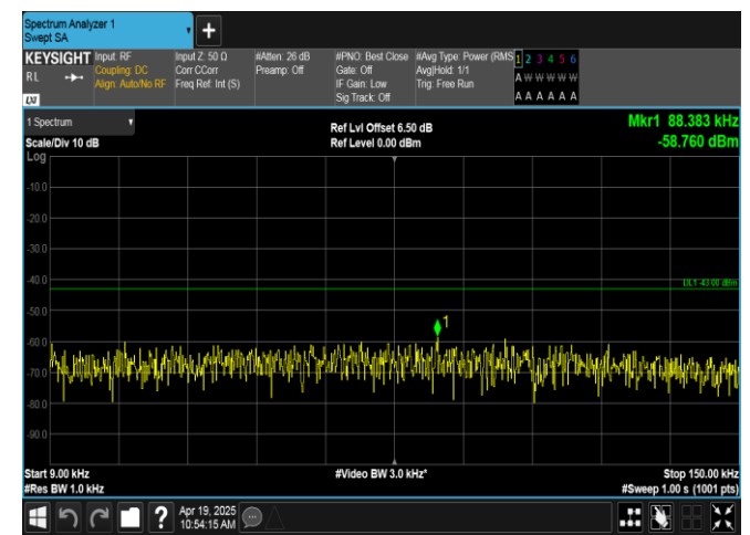
Band66-5MHz-16QAM-132647-1RB#0-0.009~0.15-PASS
