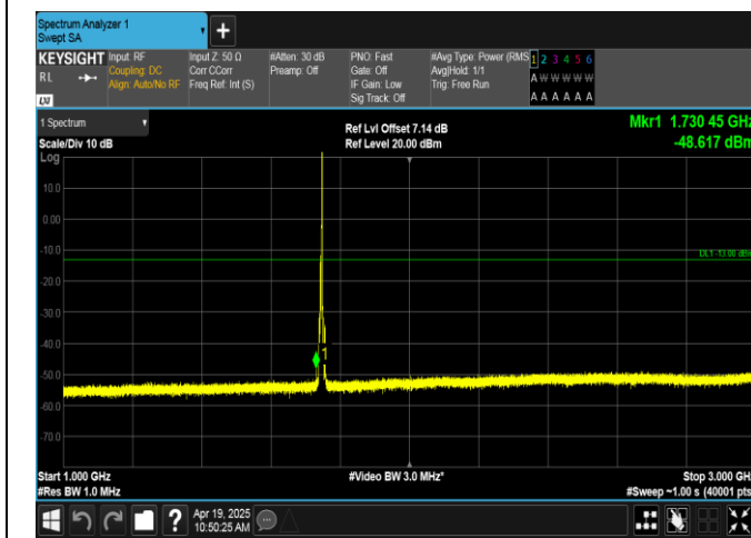
Band66-5MHz-16QAM-132322-1RB#24-1000~3000-PASS
