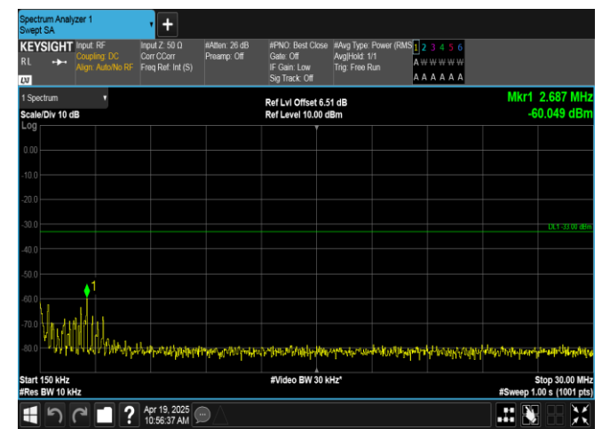
Band66-5MHz-16QAM-132647-1RB#24-0.15~30-PASS
