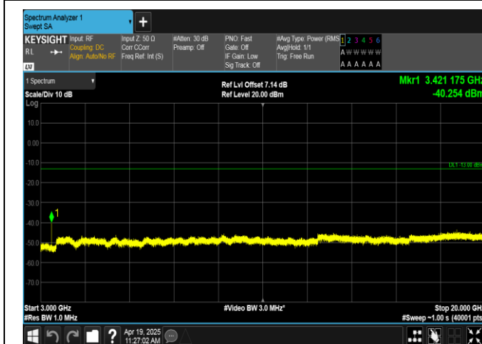
Band66-10MHz-QPSK-132022-1RB#0-3000~20000-PASS
