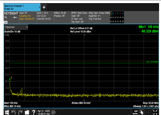
Band66-10MHz-QPSK-132022-50RB#0-0.15~30-PASS
