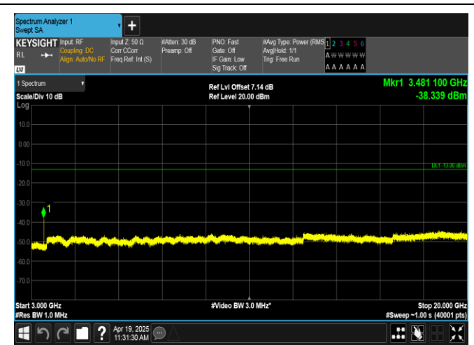
Band66-10MHz-QPSK-132322-1RB#0-3000~20000-PASS
