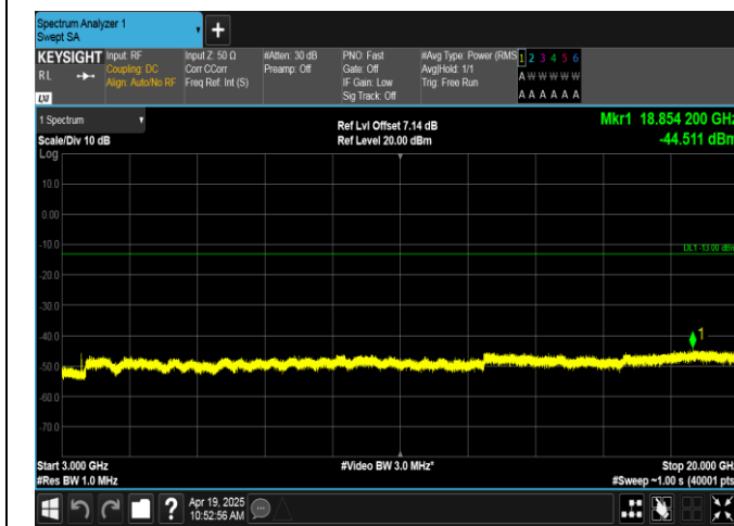
Band66-5MHz-16QAM-132322-25RB#0-3000~20000-PASS
