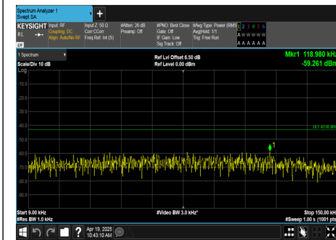
Band66-5MHz-16QAM-131997-1RB#24-0.009~0.15-PASS
