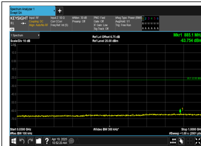
Band66-5MHz-16QAM-132322-25RB#0-30~1000-PASS
