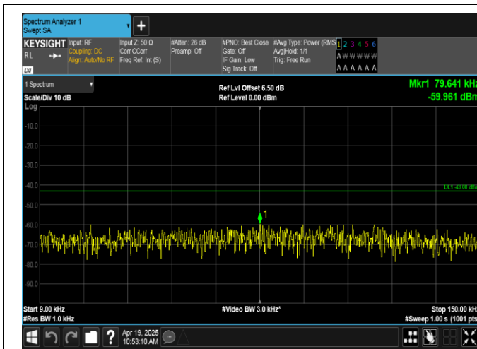
Band66-5MHz-QPSK-132647-1RB#0-0.009~0.15-PASS
