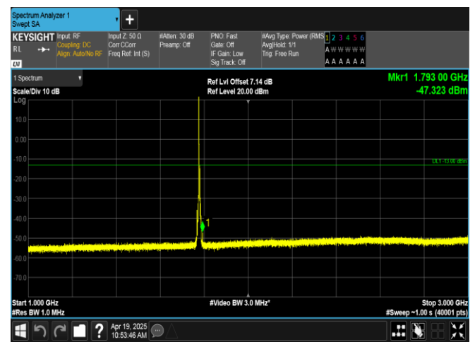
Band66-5MHz-QPSK-132647-1RB#0-1000~3000-PASS
