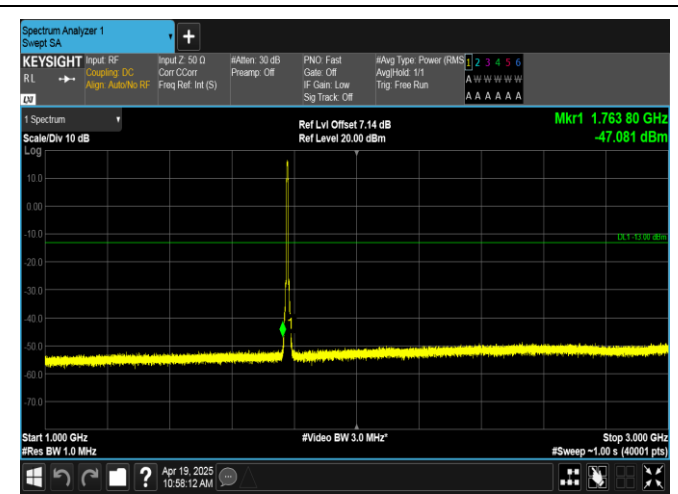
Band66-5MHz-QPSK-132647-25RB#0-1000~3000-PASS
