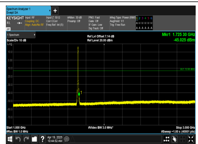
Band66-5MHz-QPSK-131997-25RB#0-1000~3000-PASS
