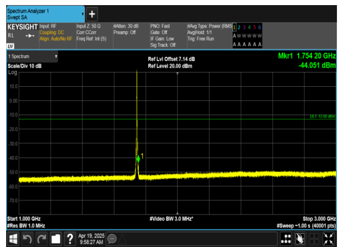
Band66-3MHz-16QAM-132322-1RB#0-1000~3000-PASS
