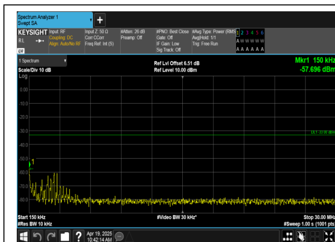
Band66-5MHz-QPSK-131997-1RB#24-0.15~30-PASS
