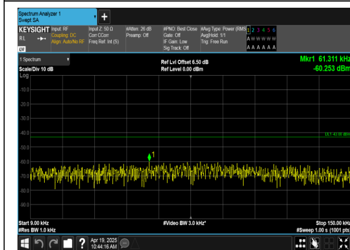
Band66-5MHz-QPSK-131997-25RB#0-0.009~0.15-PASS
