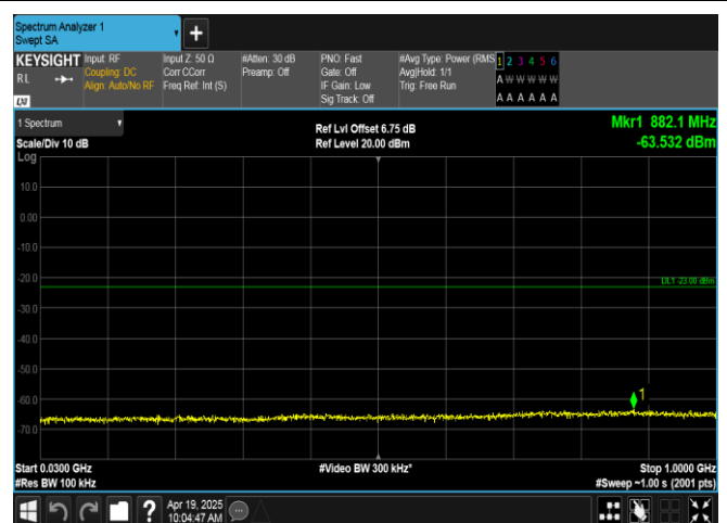
Band66-3MHz-16QAM-132657-1RB#0-30~1000-PASS
