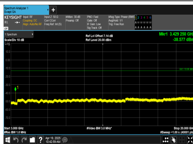
Band66-5MHz-QPSK-131997-1RB#24-3000~20000-PASS
