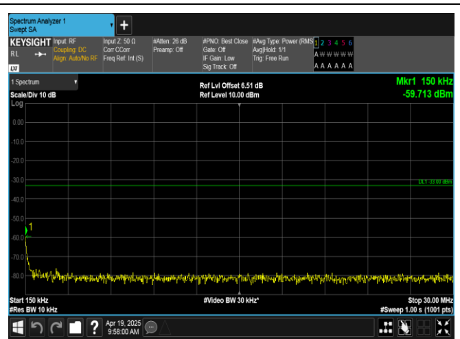
Band66-3MHz-16QAM-132322-1RB#0-0.15~30-PASS
