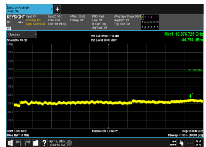
Band66-5MHz-QPSK-132322-25RB#0-3000~20000-PASS
