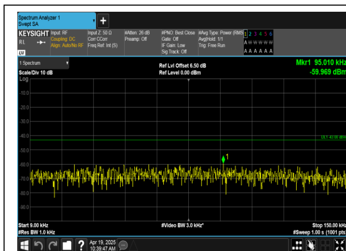
Band66-5MHz-QPSK-131997-1RB#0-0.009~0.15-PASS
