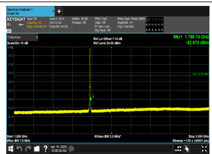
Band66-3MHz-QPSK-132657-15RB#0-1000~3000-PASS
