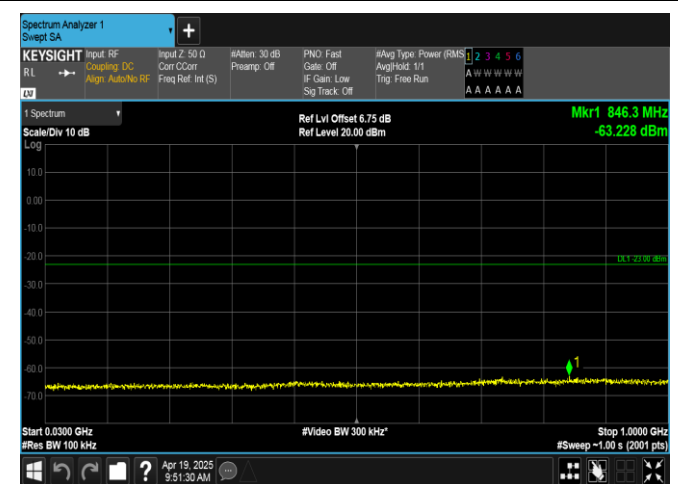
Band66-3MHz-16QAM-131987-1RB#0-30~1000-PASS
