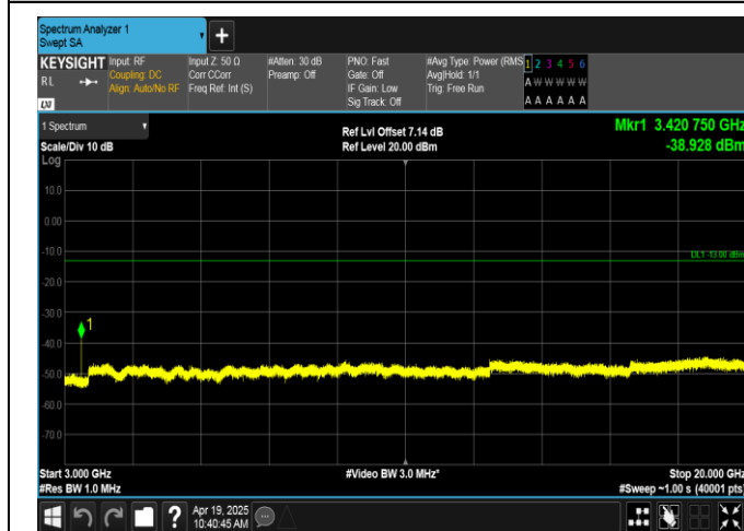
Band66-5MHz-QPSK-131997-1RB#0-3000~20000-PASS
