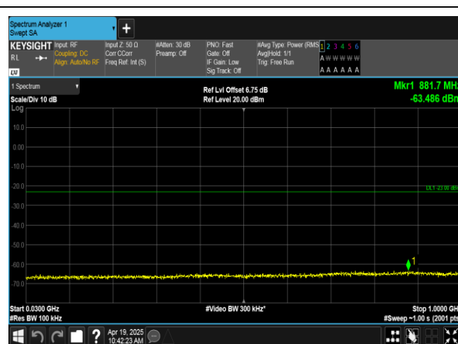
Band66-5MHz-QPSK-131997-1RB#24-30~1000-PASS
