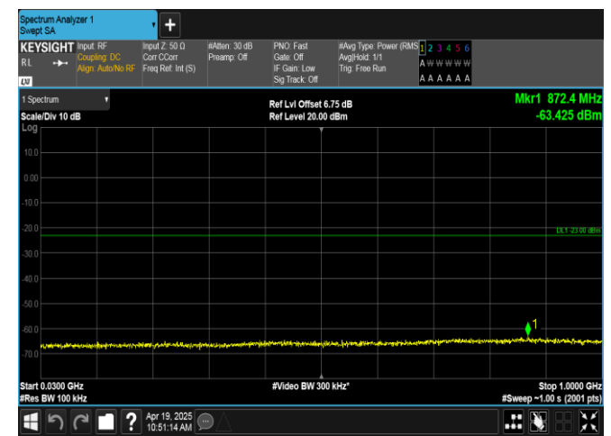
Band66-5MHz-QPSK-132322-25RB#0-30~1000-PASS
