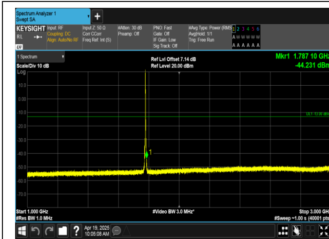
Band66-3MHz-16QAM-132657-1RB#0-1000~3000-PASS
