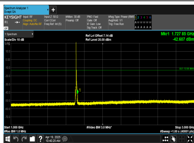
Band66-5MHz-QPSK-131997-1RB#0-1000~3000-PASS
