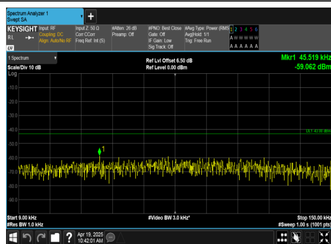
Band66-5MHz-QPSK-131997-1RB#24-0.009~0.15-PASS
