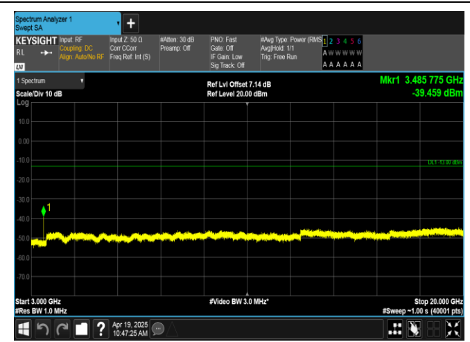
Band66-5MHz-QPSK-132322-1RB#0-3000~20000-PASS
