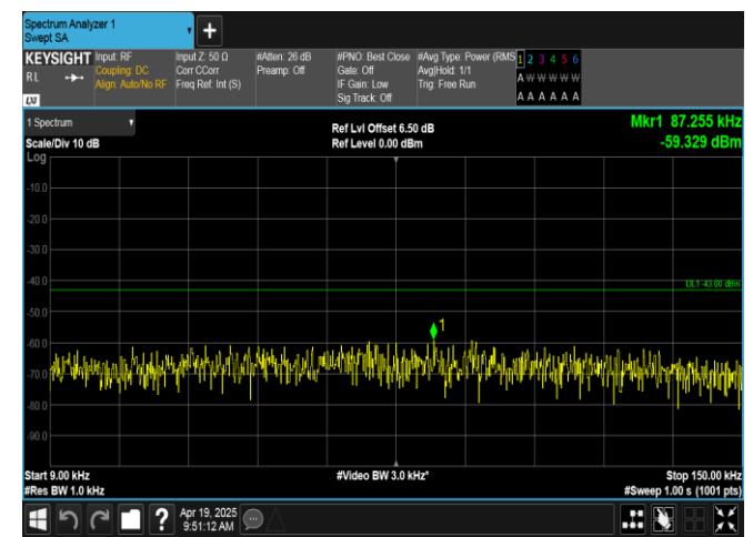
Band66-3MHz-16QAM-131987-1RB#0-0.009~0.15-PASS
