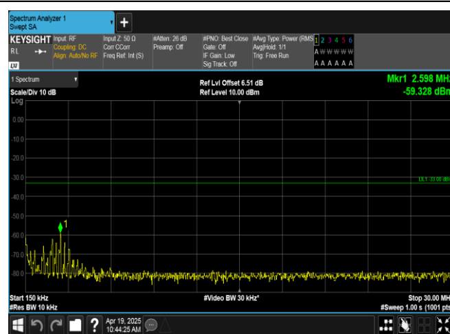
Band66-5MHz-QPSK-131997-25RB#0-0.15~30-PASS
