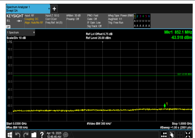
Band66-5MHz-QPSK-132322-1RB#0-30~1000-PASS
