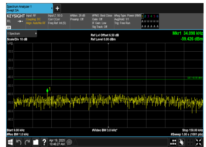
Band66-5MHz-QPSK-132322-1RB#0-0.009~0.15-PASS
