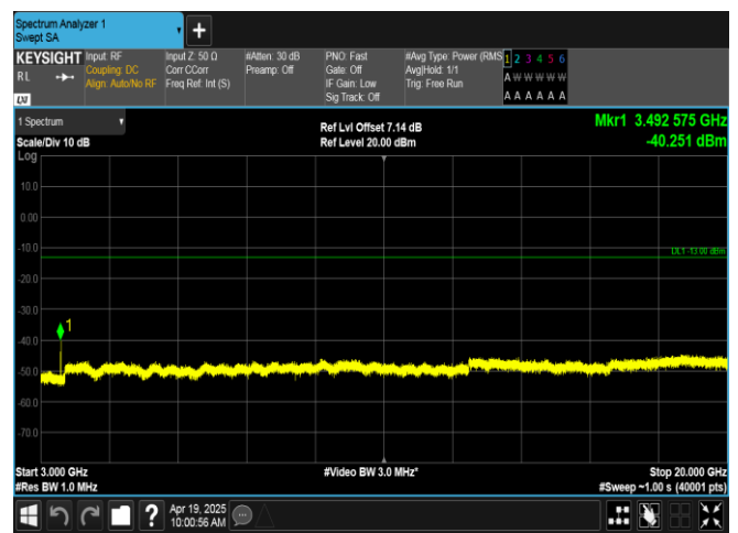
Band66-3MHz-16QAM-132322-1RB#14-3000~20000-PASS
