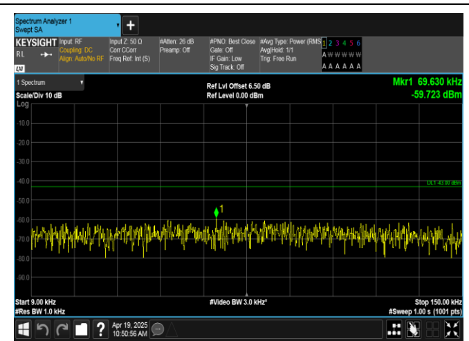
Band66-5MHz-QPSK-132322-25RB#0-0.009~0.15-PASS
