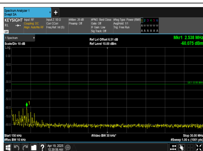
Band66-5MHz-QPSK-131997-1RB#0-0.15~30-PASS
