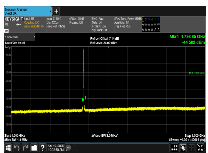
Band66-3MHz-16QAM-132322-15RB#0-1000~3000-PASS
