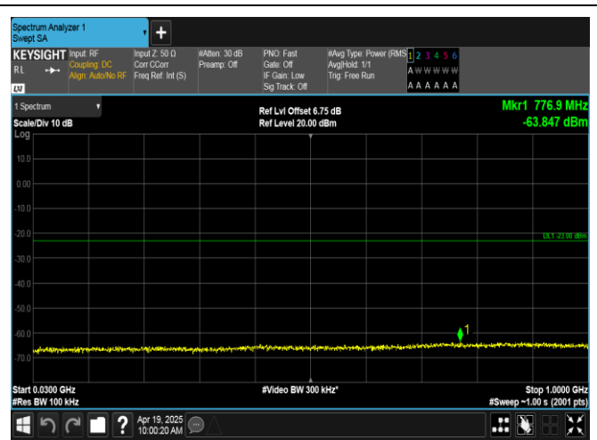
Band66-3MHz-16QAM-132322-1RB#14-30~1000-PASS
