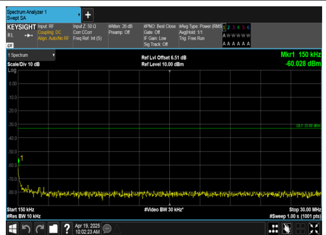
Band66-3MHz-16QAM-132322-15RB#0-0.15~30-PASS
