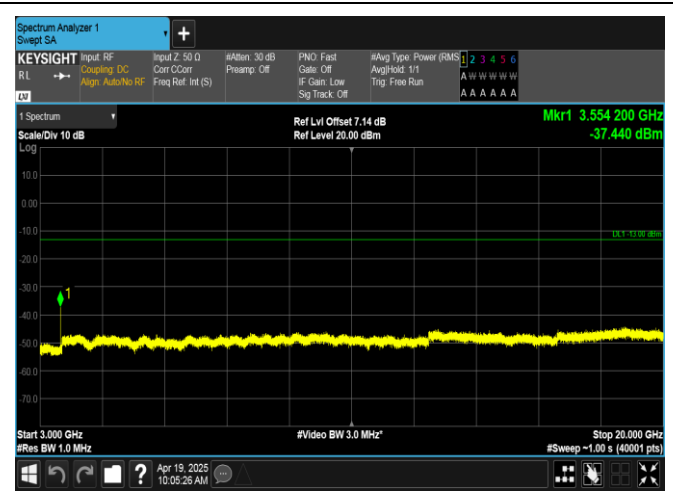
Band66-3MHz-16QAM-132657-1RB#0-3000~20000-PASS
