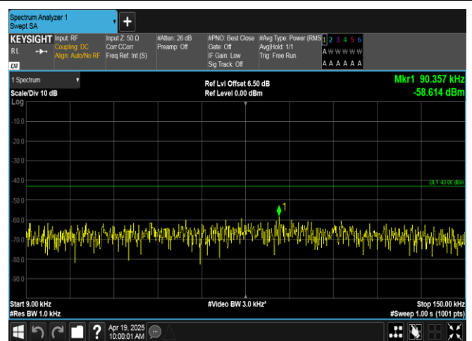
Band66-3MHz-16QAM-132322-1RB#14-0.009~0.15-PASS
