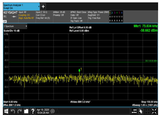
Band66-3MHz-16QAM-132657-1RB#0-0.009~0.15-PASS
