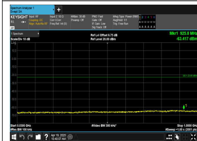
Band66-5MHz-QPSK-131997-1RB#0-30~1000-PASS
