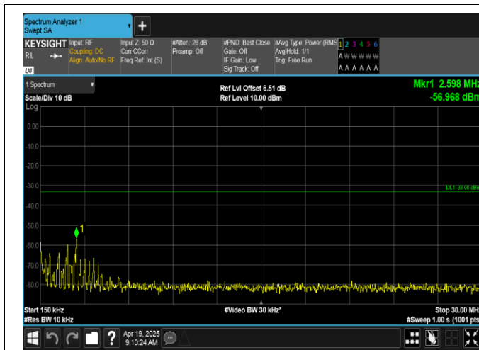
Band66-1.4MHz-16QAM-132322-1RB#5-0.15~30-PASS
