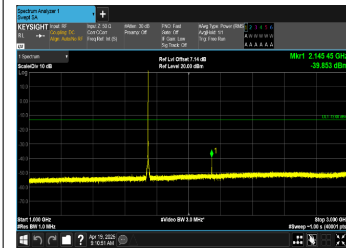
Band66-1.4MHz-16QAM-132322-1RB#5-1000~3000-PASS
