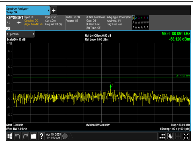
Band66-1.4MHz-16QAM-132665-6RB#0-0.009~0.15-PASS
