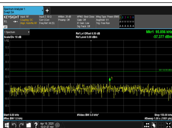
Band66-3MHz-QPSK-132322-15RB#0-0.009~0.15-PASS
