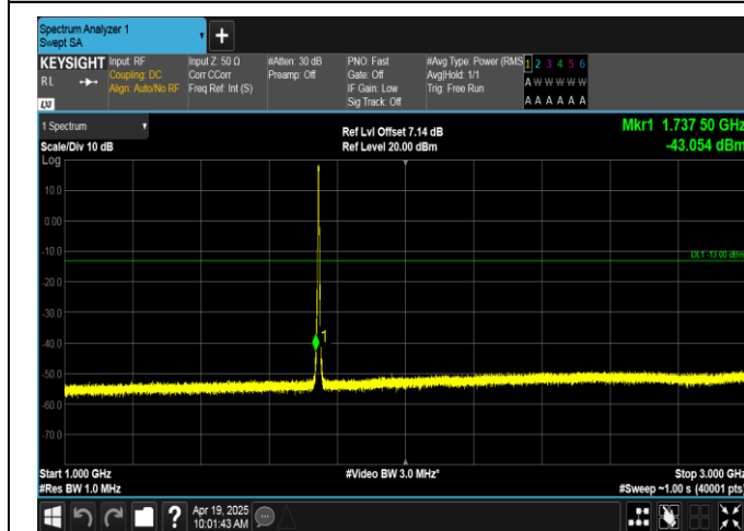
Band66-3MHz-QPSK-132322-15RB#0-1000~3000-PASS
