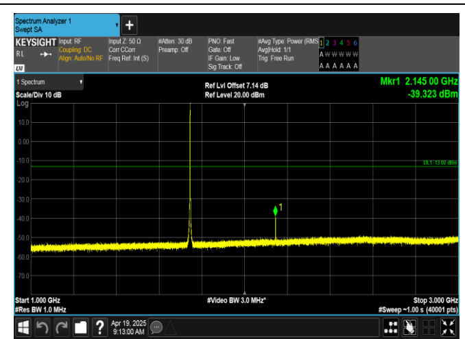
Band66-1.4MHz-16QAM-132322-6RB#0-1000~3000-PASS
