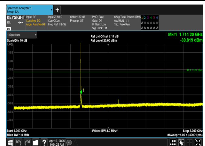
Band66-1.4MHz-16QAM-131979-1RB#5-1000~3000-PASS
