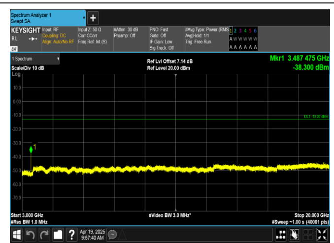
Band66-3MHz-QPSK-132322-1RB#0-3000~20000-PASS
