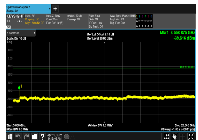
Band66-1.4MHz-16QAM-132665-6RB#0-3000~20000-PASS
