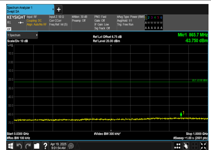
Band66-1.4MHz-16QAM-131979-1RB#0-30~1000-PASS
