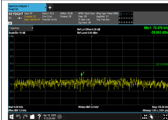
Band66-1.4MHz-16QAM-132322-6RB#0-0.009~0.15-PASS
