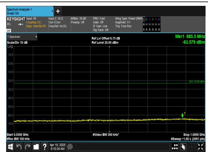
Band66-1.4MHz-16QAM-132322-1RB#5-30~1000-PASS
