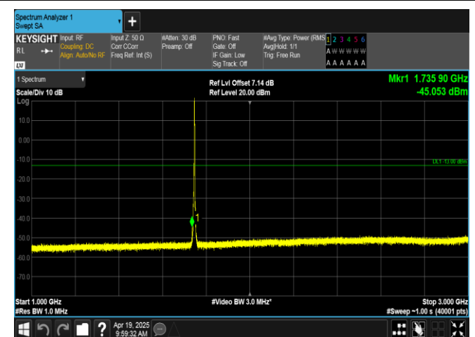
Band66-3MHz-QPSK-132322-1RB#14-1000~3000-PASS
