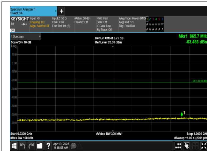
Band66-1.4MHz-QPSK-132665-6RB#0-30~1000-PASS
