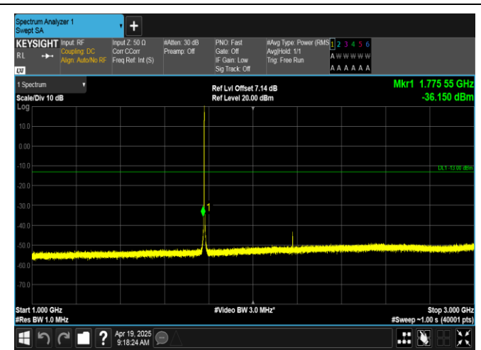
Band66-1.4MHz-QPSK-132665-6RB#0-1000~3000-PASS
