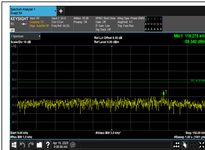
Band66-1.4MHz-16QAM-132322-1RB#0-0.009~0.15-PASS
