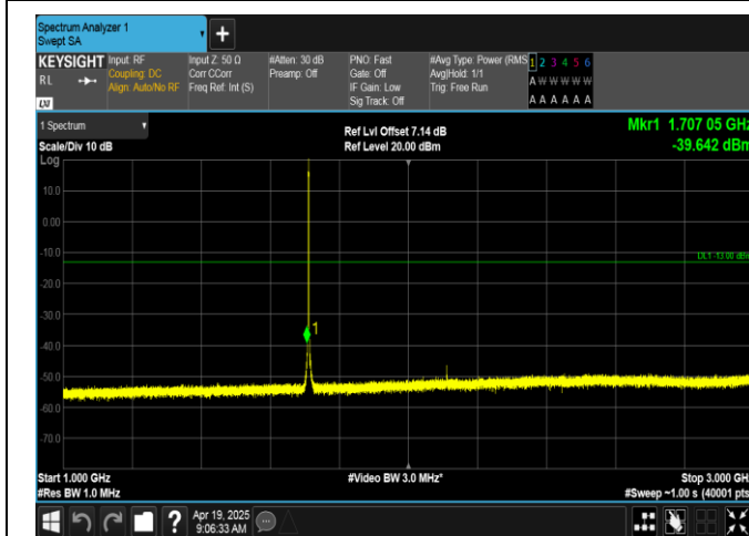
Band66-1.4MHz-16QAM-131979-6RB#0-1000~3000-PASS
