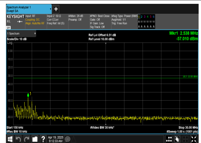
Band66-1.4MHz-16QAM-132322-6RB#0-0.15~30-PASS
