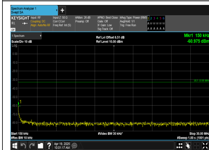
Band66-3MHz-QPSK-132322-15RB#0-0.15~30-PASS
