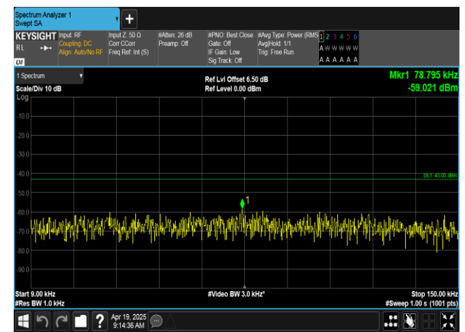
Band66-1.4MHz-16QAM-132665-1RB#0-0.009~0.15-PASS
