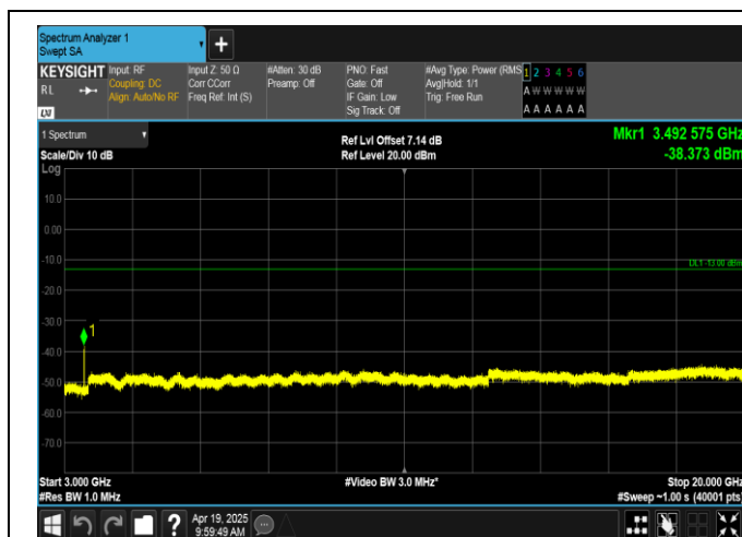
Band66-3MHz-QPSK-132322-1RB#14-3000~20000-PASS
