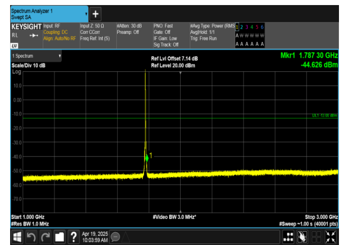
Band66-3MHz-QPSK-132657-1RB#0-1000~3000-PASS
