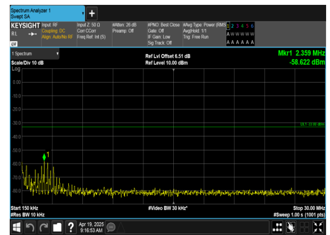
Band66-1.4MHz-16QAM-132665-1RB#5-0.15~30-PASS
