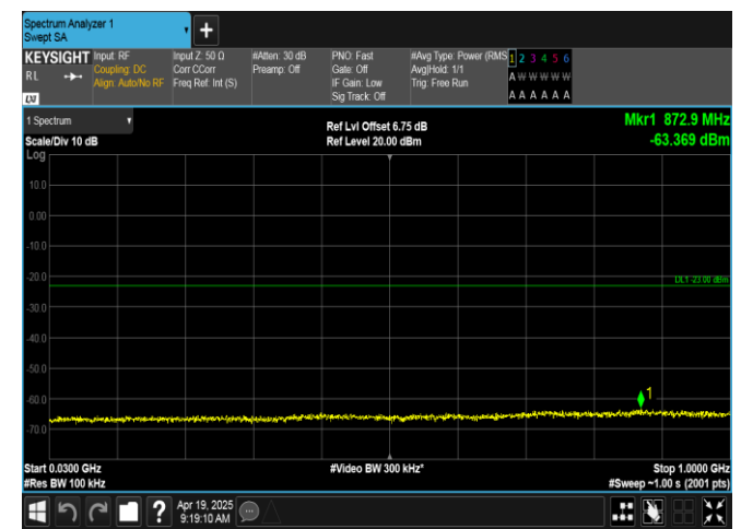
Band66-1.4MHz-16QAM-132665-6RB#0-30~1000-PASS
