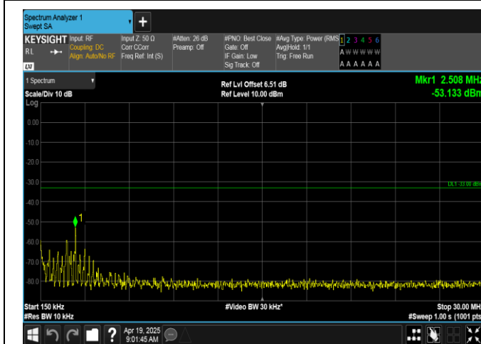
Band66-1.4MHz-16QAM-131979-1RB#0-0.15~30-PASS
