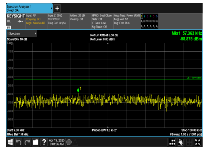
Band66-1.4MHz-16QAM-131979-1RB#0-0.009~0.15-PASS
