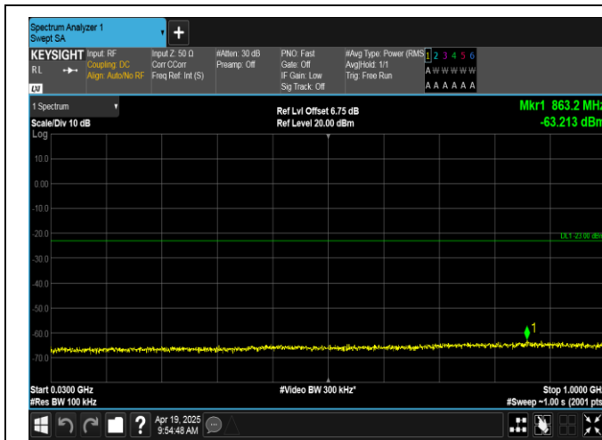
Band66-3MHz-QPSK-131987-15RB#0-30~1000-PASS
