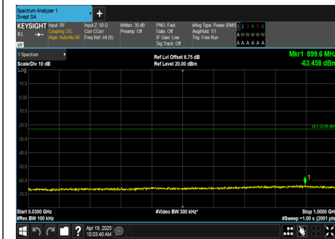
Band66-3MHz-QPSK-132657-1RB#0-30~1000-PASS
