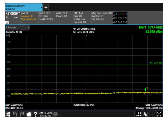
Band66-1.4MHz-16QAM-132665-1RB#0-30~1000-PASS
