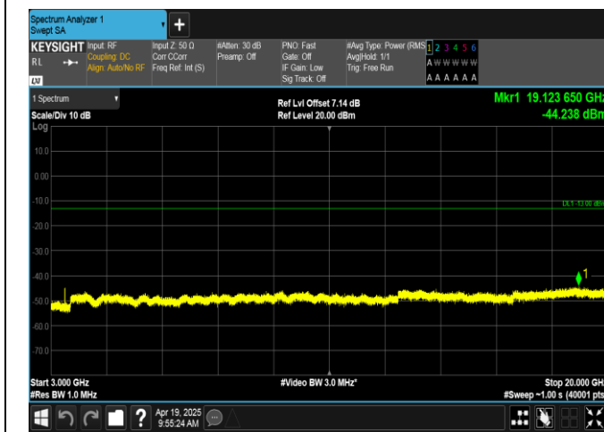
Band66-3MHz-QPSK-131987-15RB#0-3000~20000-PASS
