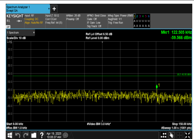
Band66-3MHz-QPSK-132657-1RB#14-0.009~0.15-PASS
