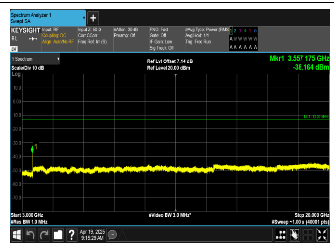
Band66-1.4MHz-16QAM-132665-1RB#0-3000~20000-PASS
