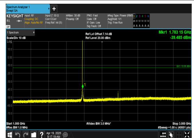
Band66-1.4MHz-16QAM-132665-1RB#5-1000~3000-PASS
