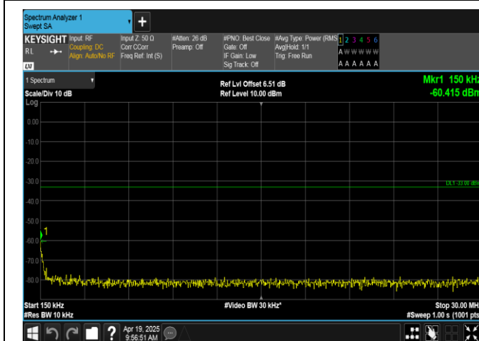
Band66-3MHz-QPSK-132322-1RB#0-0.15~30-PASS
