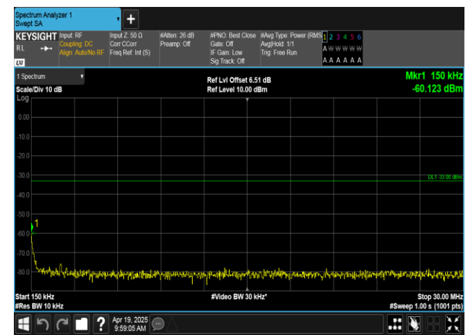
Band66-3MHz-QPSK-132322-1RB#14-0.15~30-PASS
