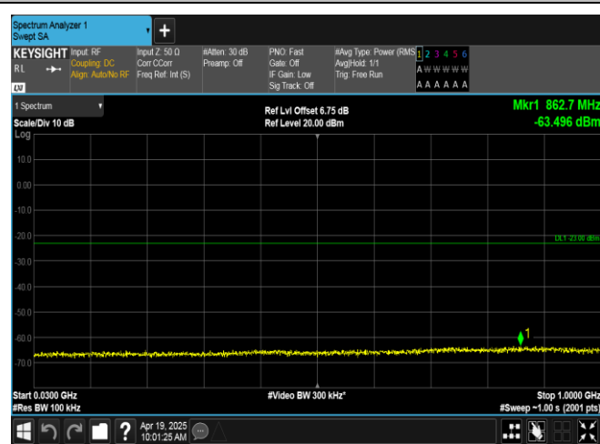
Band66-3MHz-QPSK-132322-15RB#0-30~1000-PASS
