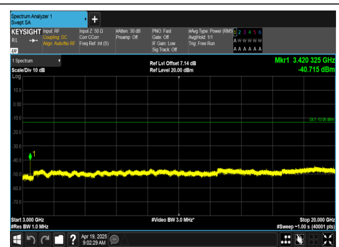
Band66-1.4MHz-16QAM-131979-1RB#0-3000~20000-PASS
