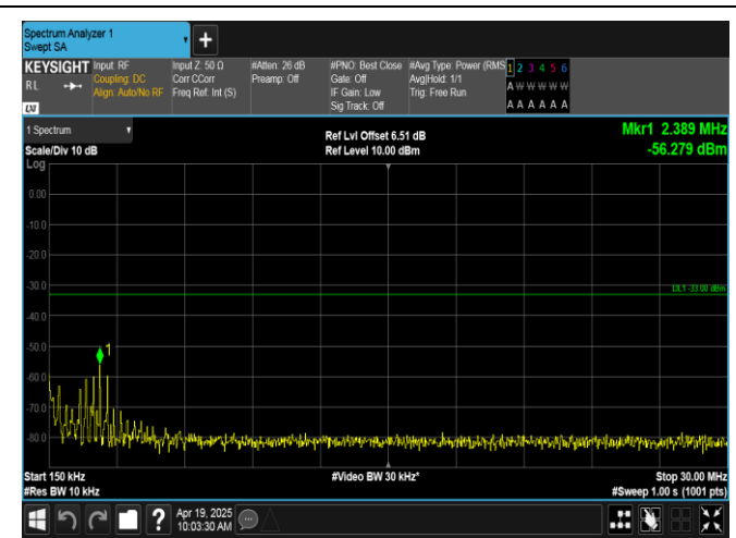
Band66-3MHz-QPSK-132657-1RB#0-0.15~30-PASS
