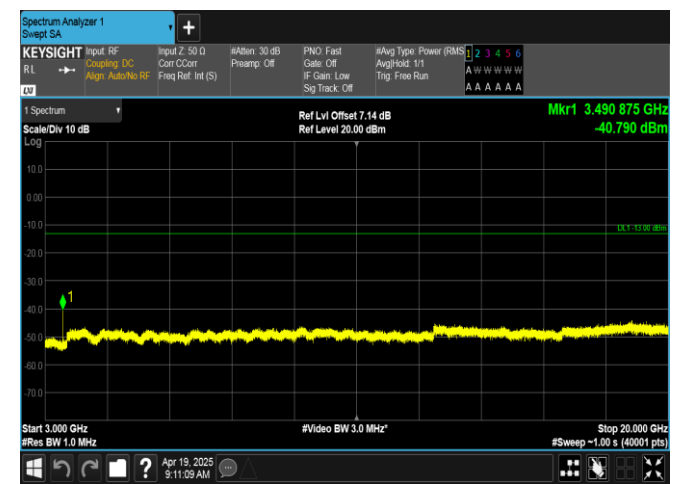
Band66-1.4MHz-16QAM-132322-1RB#5-3000~20000-PASS
