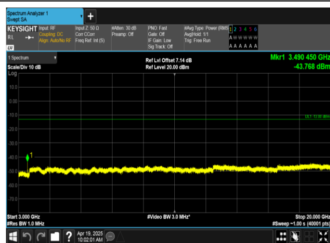
Band66-3MHz-QPSK-132322-15RB#0-3000~20000-PASS
