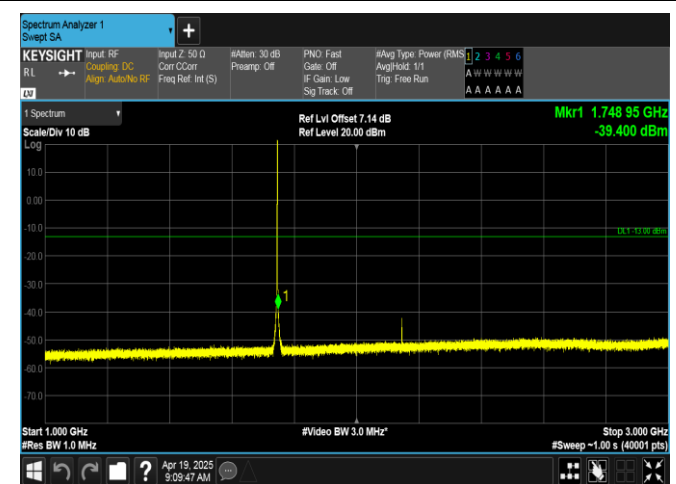
Band66-1.4MHz-QPSK-132322-1RB#5-1000~3000-PASS
