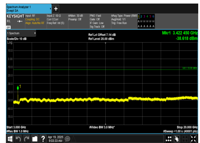
Band66-1.4MHz-QPSK-131979-1RB#5-3000~20000-PASS
