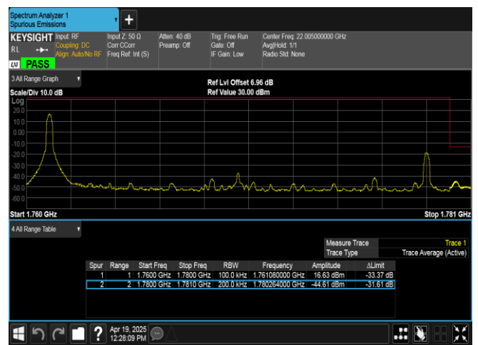
Band66-20MHz-16QAM-132572-1RB#0-PASS
