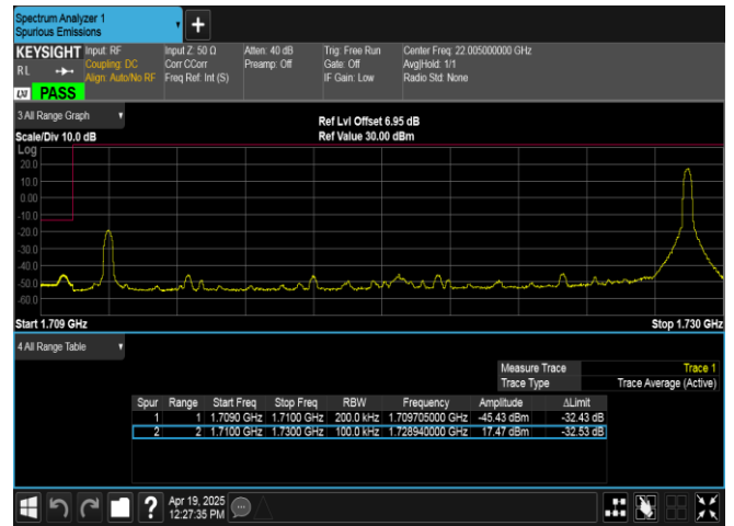
Band66-20MHz-16QAM-132072-1RB#99-PASS
