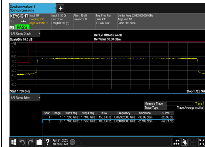
Band66-15MHz-16QAM-132047-75RB#0-PASS
