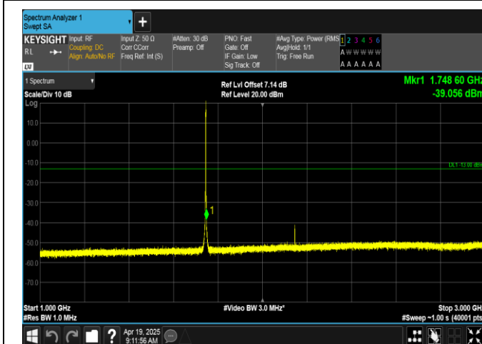
Band66-1.4MHz-QPSK-132322-6RB#0-1000~3000-PASS
