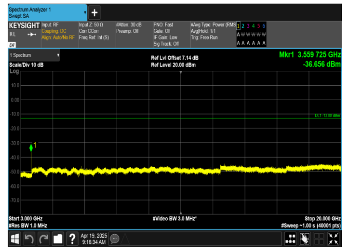
Band66-1.4MHz-QPSK-132665-1RB#5-3000~20000-PASS
