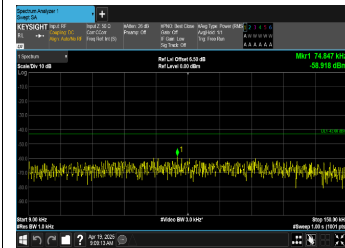
Band66-1.4MHz-QPSK-132322-1RB#5-0.009~0.15-PASS
