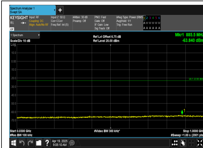
Band66-1.4MHz-QPSK-131979-6RB#0-30~1000-PASS
