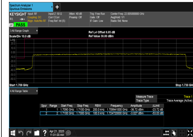
Band66-20MHz-QPSK-132072-100RB#0-PASS
