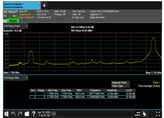
Band66-10MHz-16QAM-132022-1RB#49-PASS
