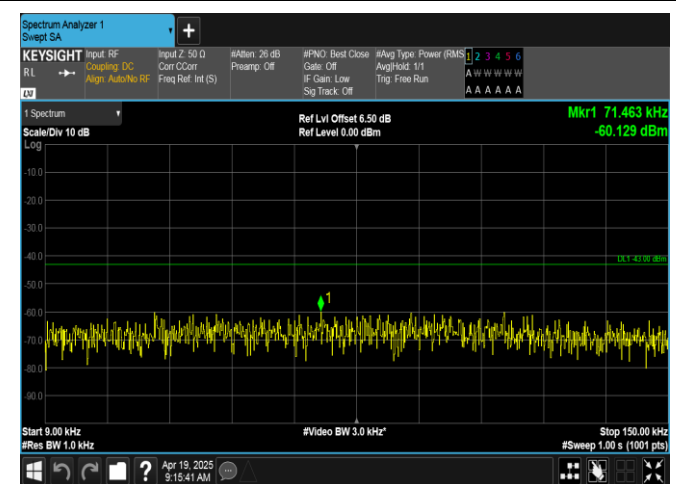
Band66-1.4MHz-QPSK-132665-1RB#5-0.009~0.15-PASS
