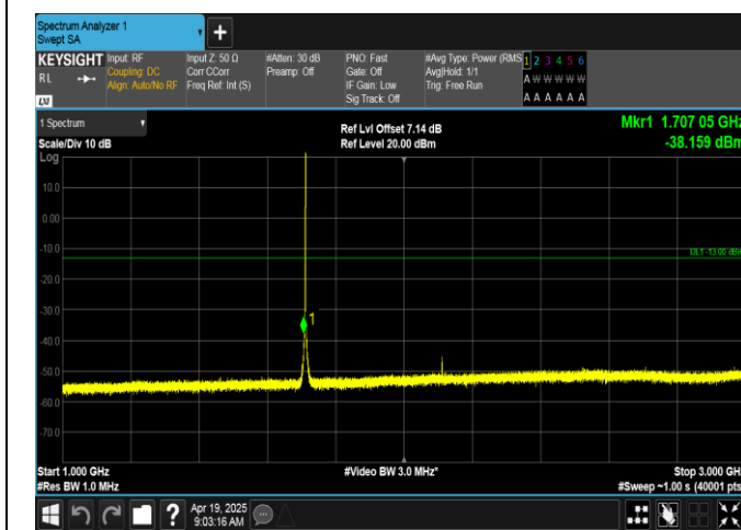
Band66-1.4MHz-QPSK-131979-1RB#5-1000~3000-PASS
