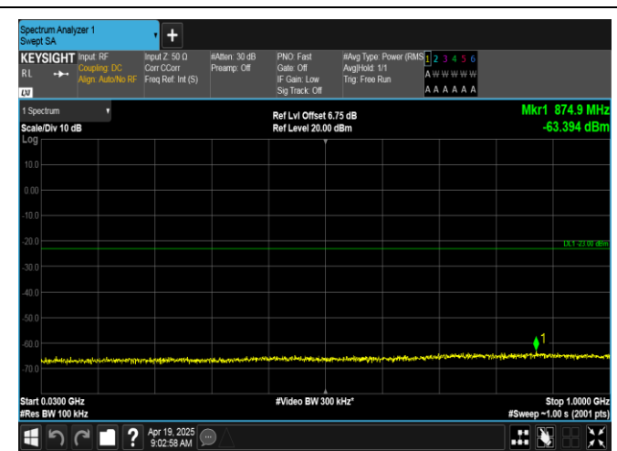
Band66-1.4MHz-QPSK-131979-1RB#5-30~1000-PASS
