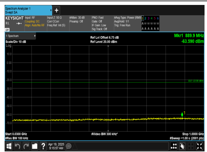
Band66-1.4MHz-QPSK-132665-1RB#5-30~1000-PASS
