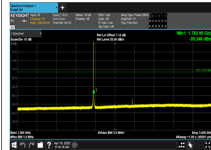
Band66-1.4MHz-QPSK-132665-1RB#5-1000~3000-PASS
