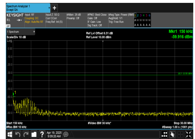
Band66-1.4MHz-QPSK-132322-1RB#5-0.15~30-PASS
