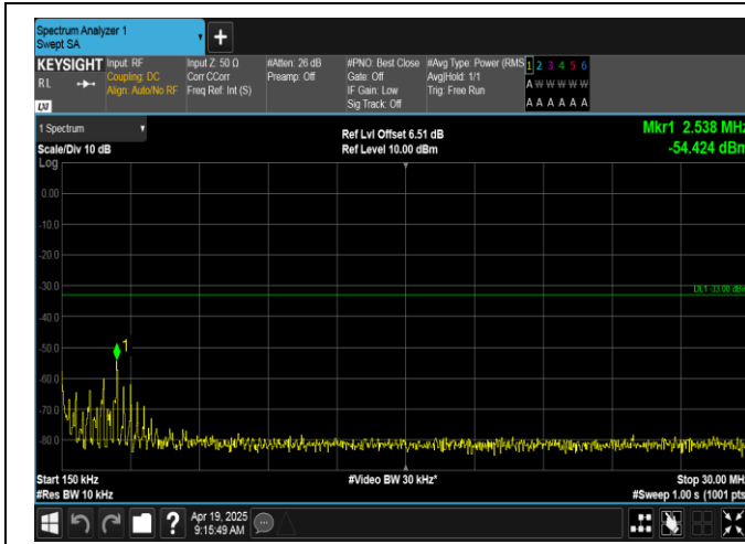
Band66-1.4MHz-QPSK-132665-1RB#5-0.15~30-PASS
