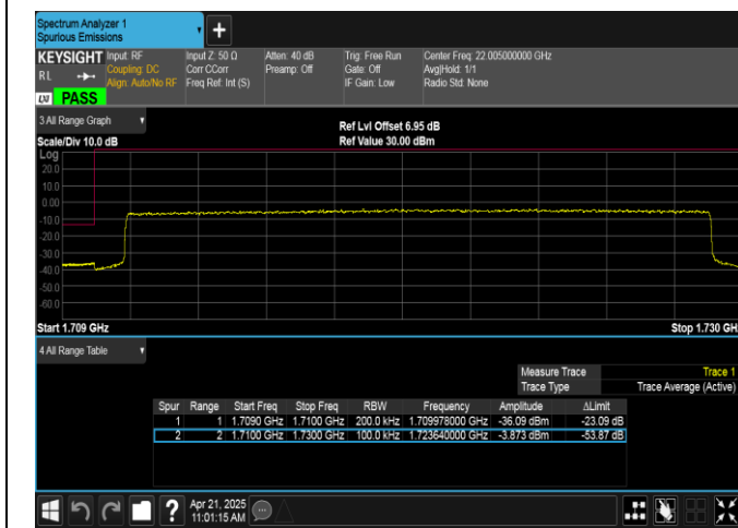
Band66-20MHz-16QAM-132072-100RB#0-PASS
