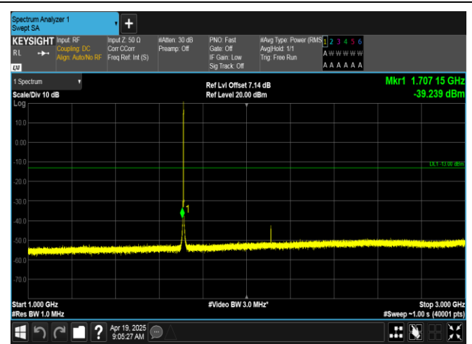
Band66-1.4MHz-QPSK-131979-6RB#0-1000~3000-PASS
