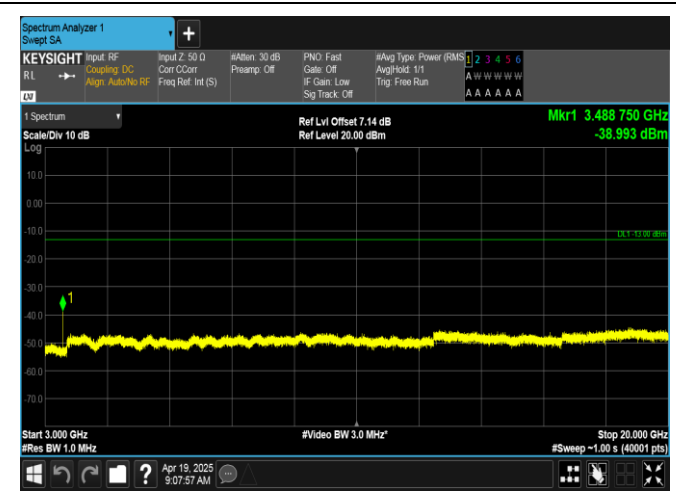
Band66-1.4MHz-QPSK-132322-1RB#0-3000~20000-PASS
