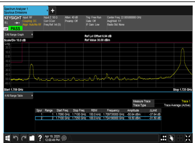
Band66-15MHz-QPSK-132047-1RB#74-PASS
