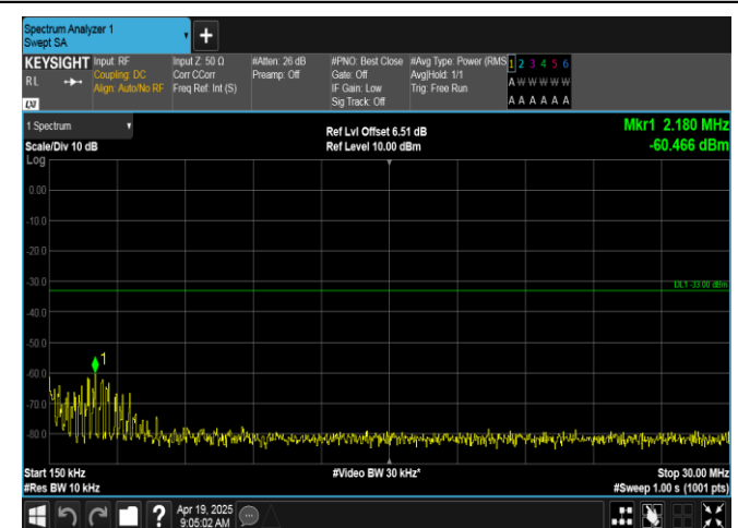
Band66-1.4MHz-QPSK-131979-6RB#0-0.15~30-PASS
