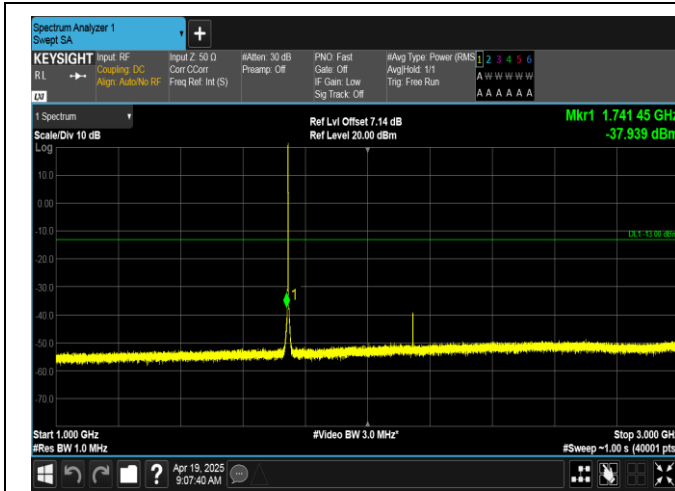
Band66-1.4MHz-QPSK-132322-1RB#0-1000~3000-PASS
