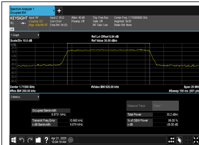
Band66-10MHz-QPSK-132022-50RB#0-PASS
