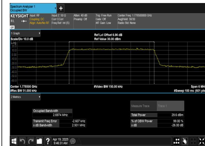
Band66-3MHz-QPSK-132657-15RB#0-PASS
