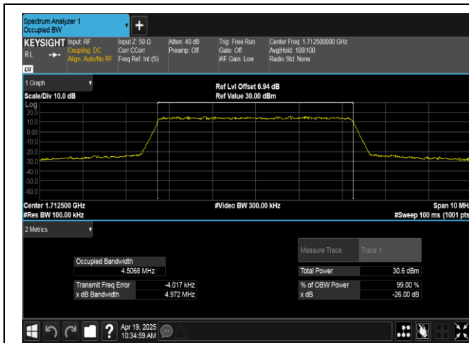
Band66-5MHz-QPSK-131997-25RB#0-PASS
