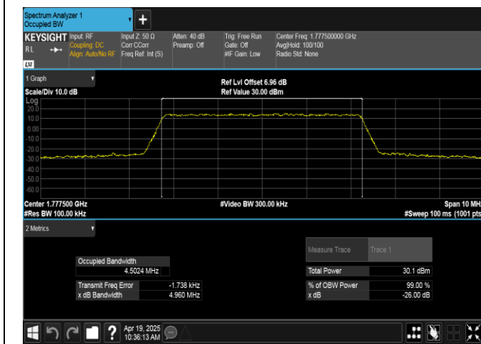
Band66-5MHz-QPSK-132647-25RB#0-PASS
