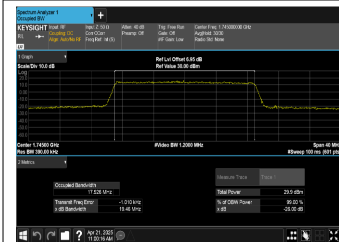
Band66-20MHz-16QAM-132322-100RB#0-PASS
