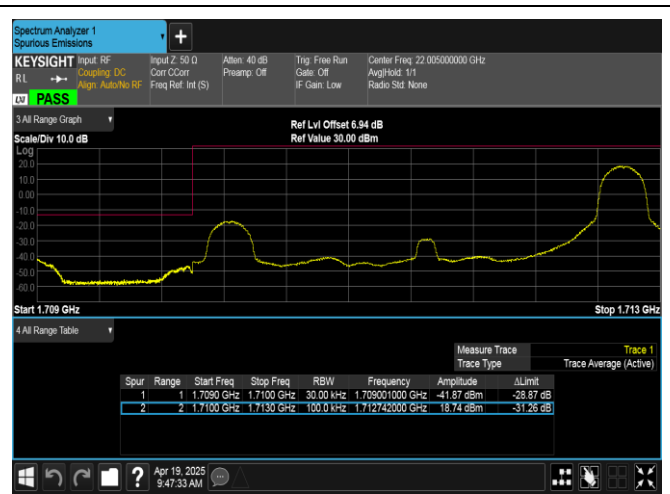
Band66-3MHz-QPSK-131987-1RB#14-PASS
