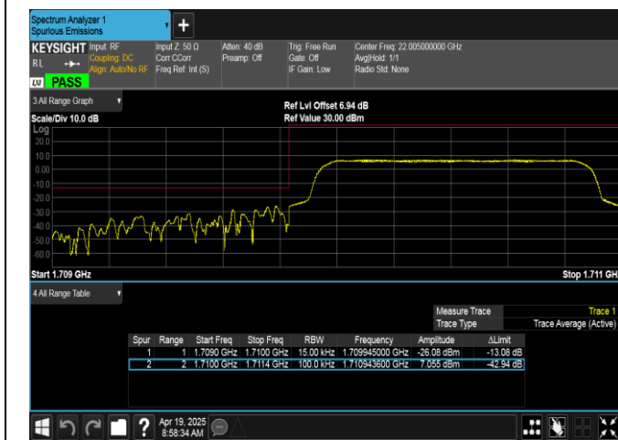
Band66-1.4MHz-16QAM-131979-6RB#0-PASS
