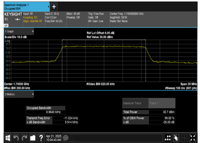
Band66-10MHz-QPSK-132322-50RB#0-PASS
