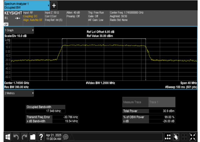
Band66-20MHz-QPSK-132322-100RB#0-PASS
