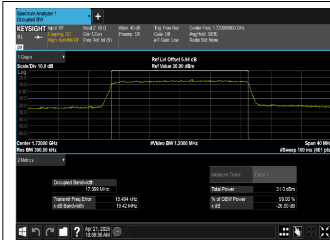
Band66-20MHz-QPSK-132072-100RB#0-PASS
