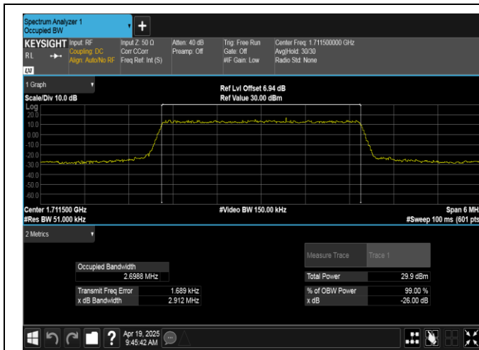
Band66-3MHz-QPSK-131987-15RB#0-PASS
