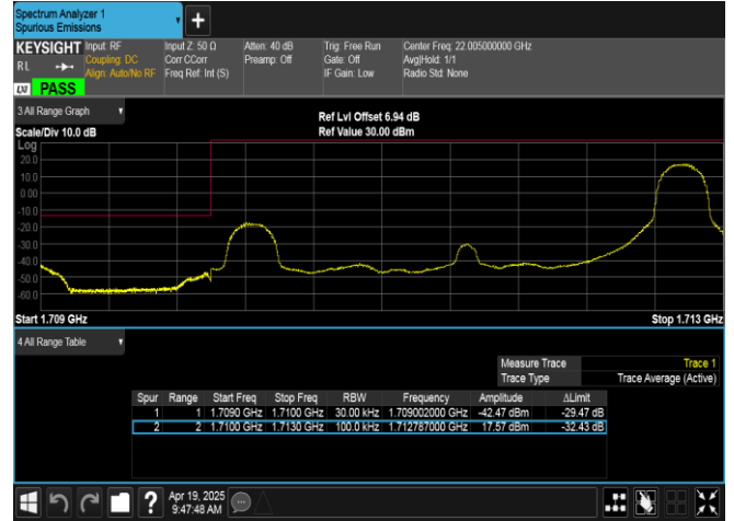
Band66-3MHz-16QAM-131987-1RB#14-PASS
