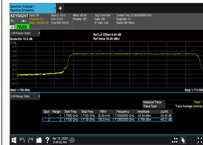
Band66-3MHz-QPSK-131987-15RB#0-PASS
