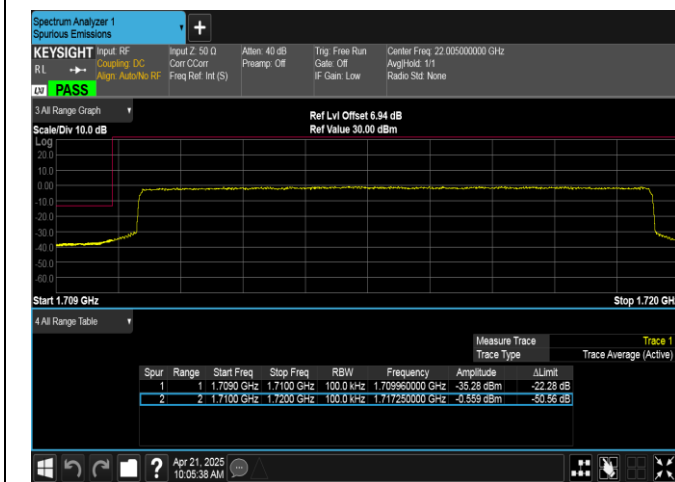
Band66-10MHz-QPSK-132022-50RB#0-PASS
