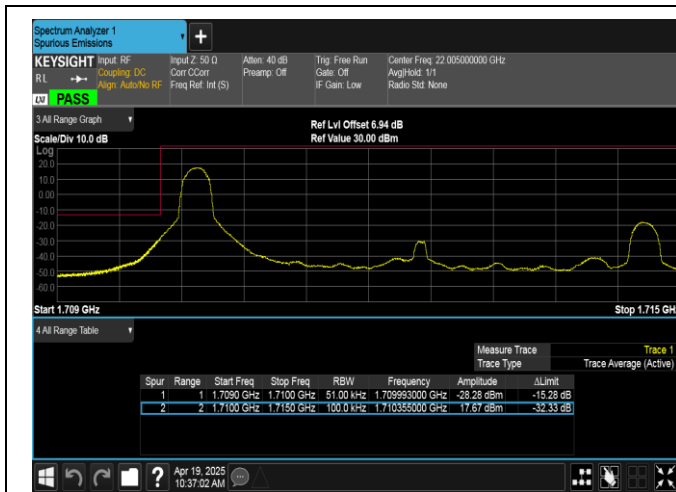
Band66-5MHz-16QAM-131997-1RB#0-PASS
