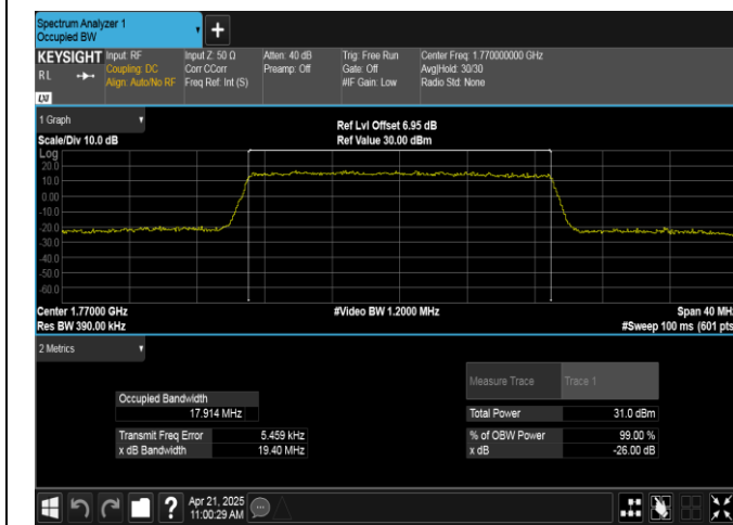
Band66-20MHz-QPSK-132572-100RB#0-PASS
