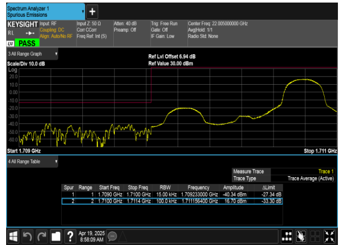
Band66-1.4MHz-16QAM-131979-1RB#5-PASS
