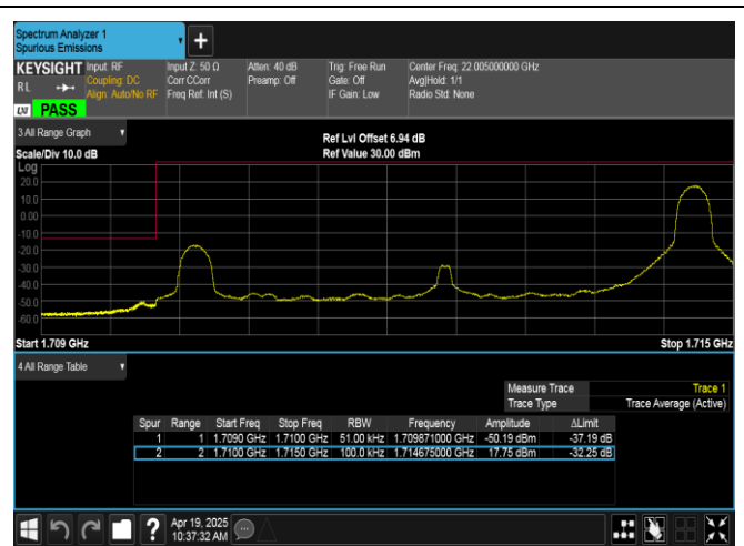
Band66-5MHz-16QAM-131997-1RB#24-PASS
