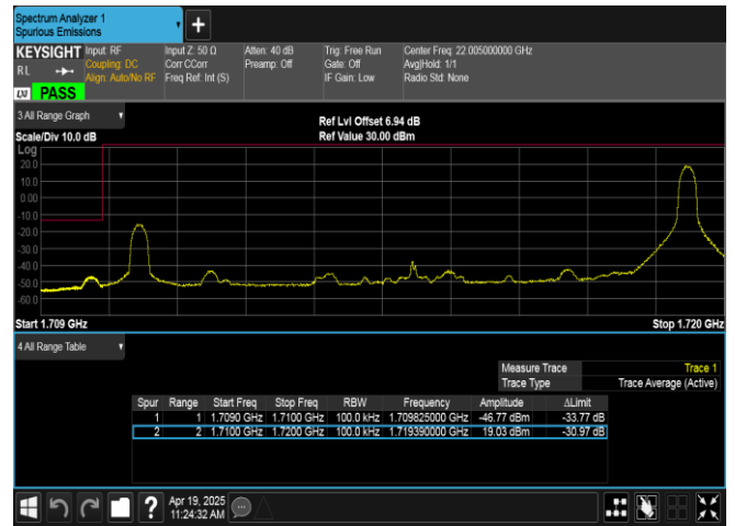
Band66-10MHz-QPSK-132022-1RB#49-PASS
