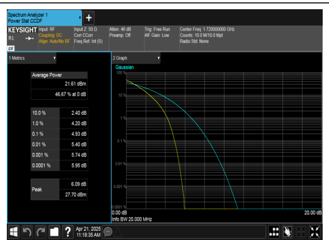
Band66-20MHz-QPSK-132072-100RB#0-PASS
