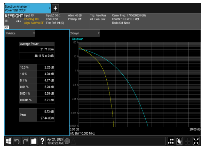
Band66-10MHz-QPSK-132322-50RB#0-PASS
