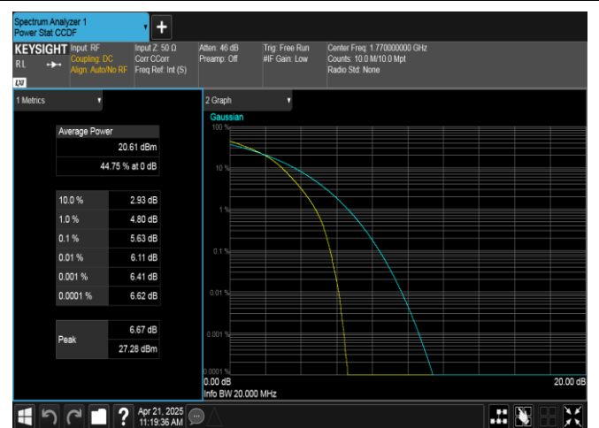
Band66-20MHz-16QAM-132572-100RB#0-PASS
