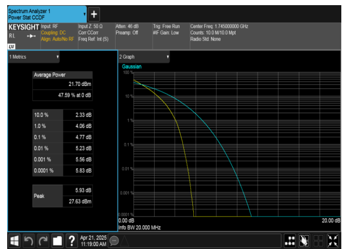
Band66-20MHz-QPSK-132322-100RB#0-PASS
