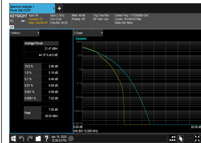
Band66-15MHz-16QAM-132597-1RB#0-PASS
