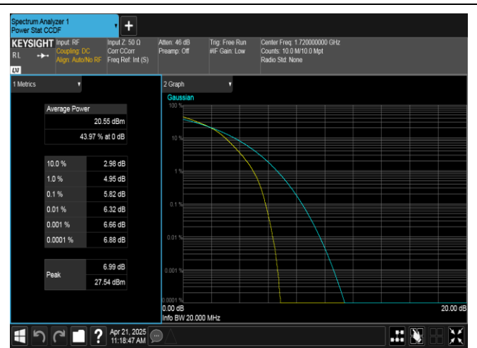
Band66-20MHz-16QAM-132072-100RB#0-PASS
