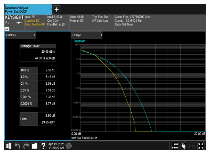
Band66-5MHz-16QAM-132647-25RB#0-PASS
