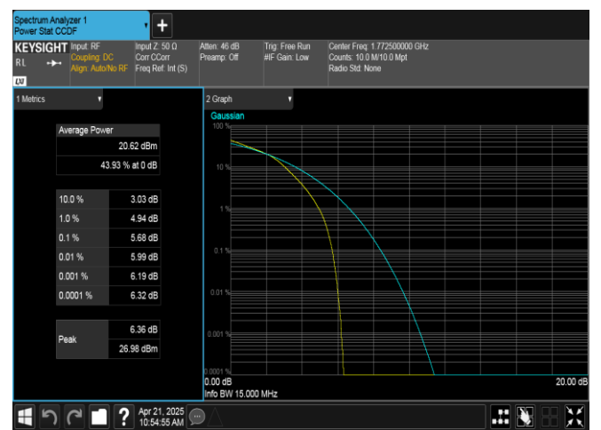
Band66-15MHz-16QAM-132597-75RB#0-PASS
