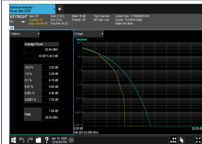
Band66-20MHz-16QAM-132572-1RB#0-PASS
