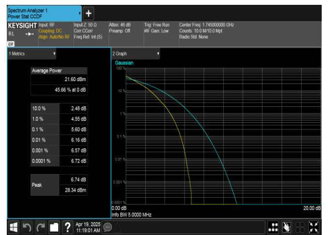
Band66-5MHz-QPSK-132322-25RB#0-PASS
