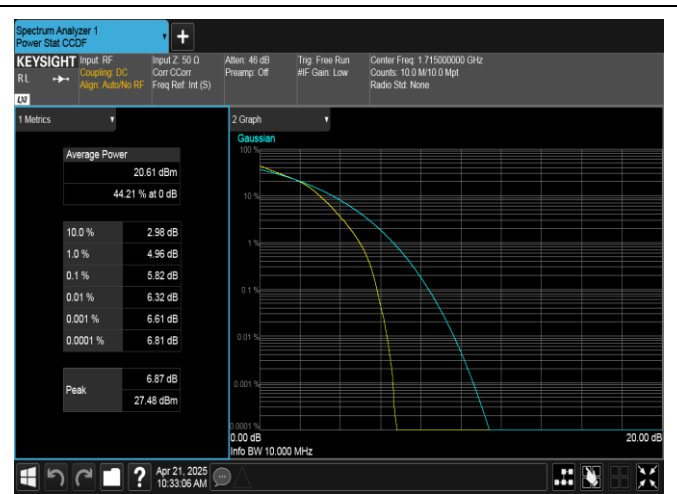
Band66-10MHz-16QAM-132022-50RB#0-PASS
