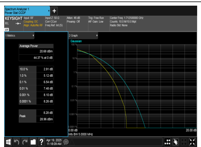
Band66-5MHz-16QAM-131997-25RB#0-PASS
