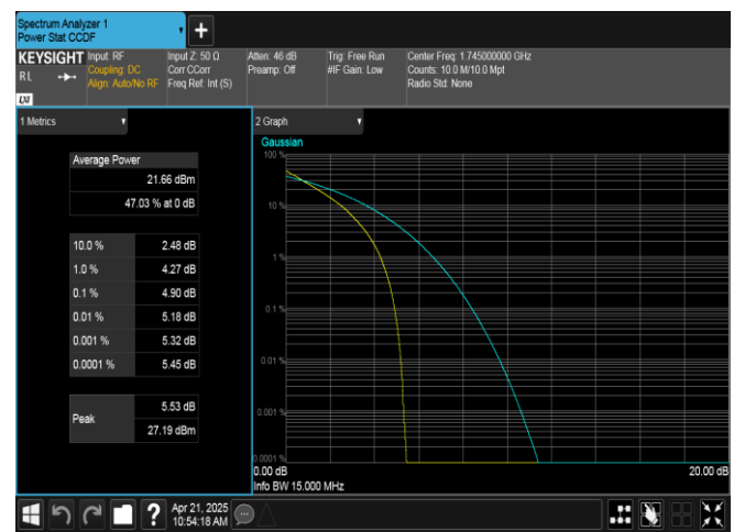
Band66-15MHz-QPSK-132322-75RB#0-PASS
