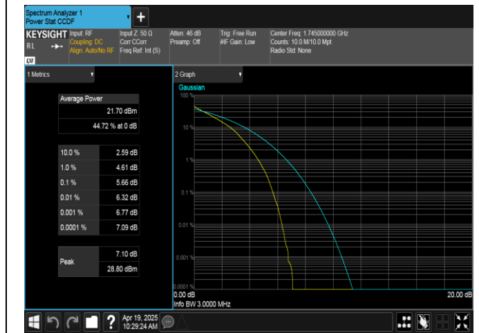
Band66-3MHz-QPSK-132322-15RB#0-PASS
