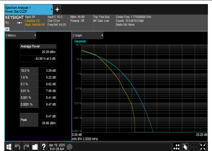
Band66-1.4MHz-16QAM-132665-6RB#0-PASS
