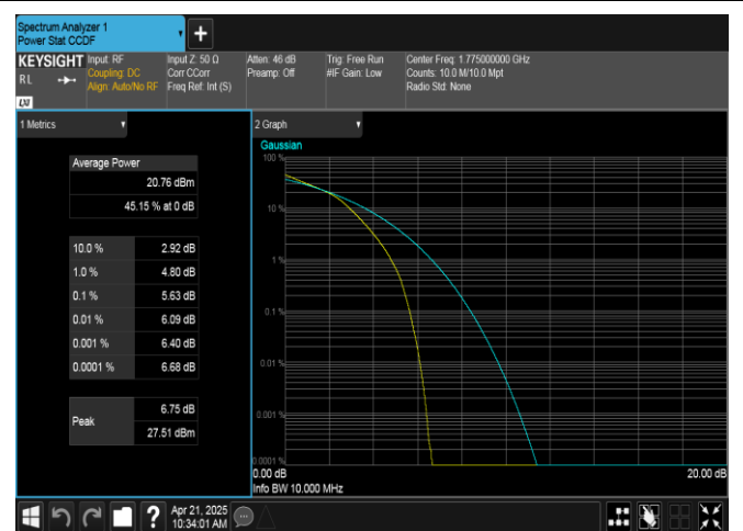
Band66-10MHz-16QAM-132622-50RB#0-PASS
