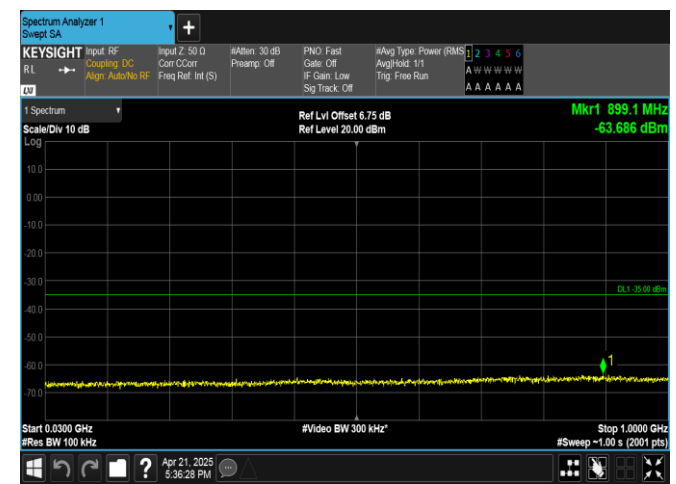
Band41-20MHz-16QAM-41490-1RB#0-30~1000-PASS
