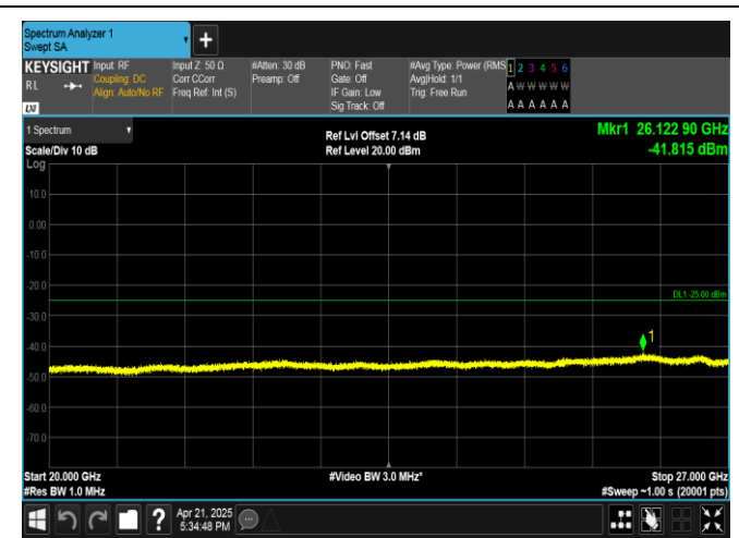
Band41-20MHz-16QAM-40620-1RB#99-20000~27000-PASS
