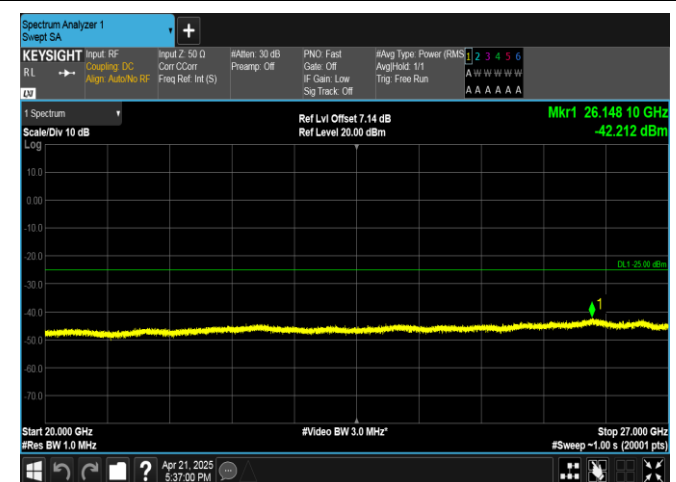
Band41-20MHz-16QAM-41490-1RB#0-20000~27000-PASS
