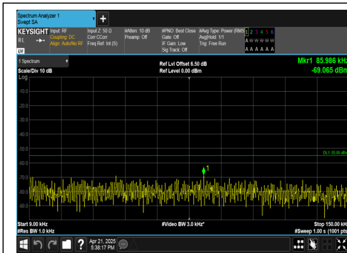
Band41-20MHz-16QAM-41490-1RB#99-0.009~0.15-PASS
