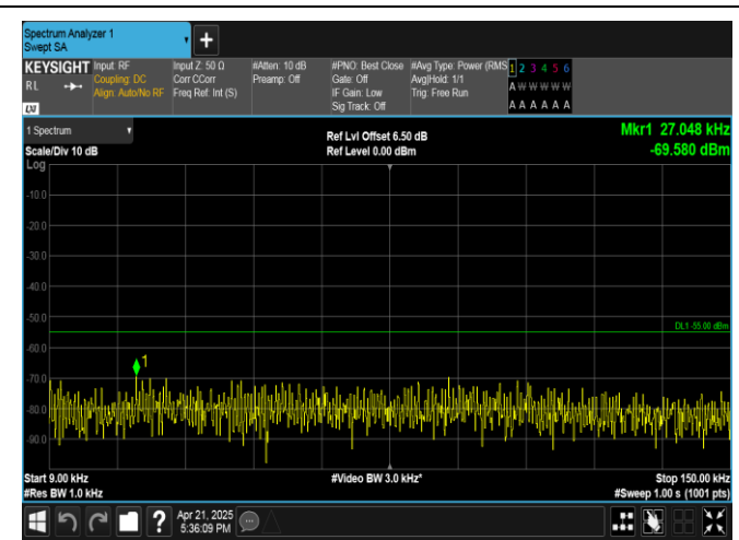
Band41-20MHz-16QAM-41490-1RB#0-0.009~0.15-PASS
