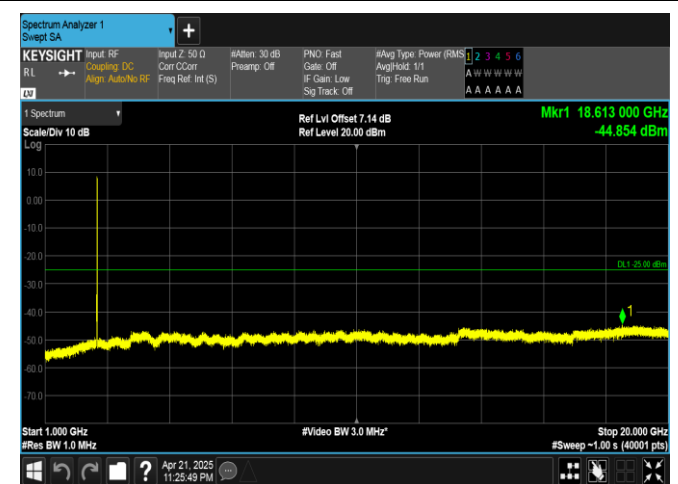
Band41-20MHz-16QAM-40620-100RB#0-1000~20000-PASS
