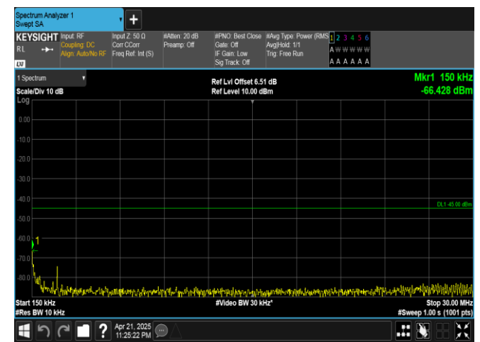
Band41-20MHz-16QAM-40620-100RB#0-0.15~30-PASS
