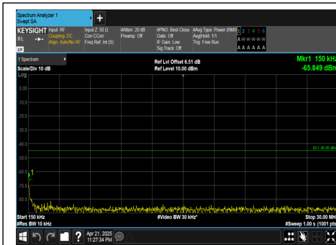
Band41-20MHz-16QAM-41490-100RB#0-0.15~30-PASS
