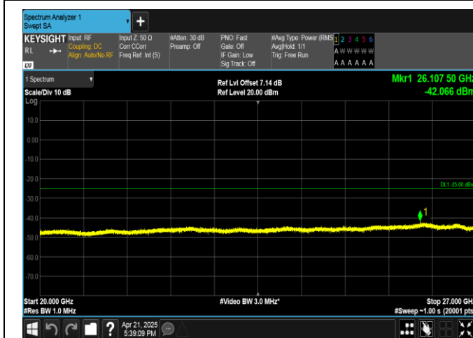
Band41-20MHz-16QAM-41490-1RB#99-20000~27000-PASS
