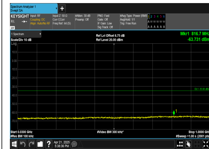
Band41-20MHz-16QAM-41490-1RB#99-30~1000-PASS
