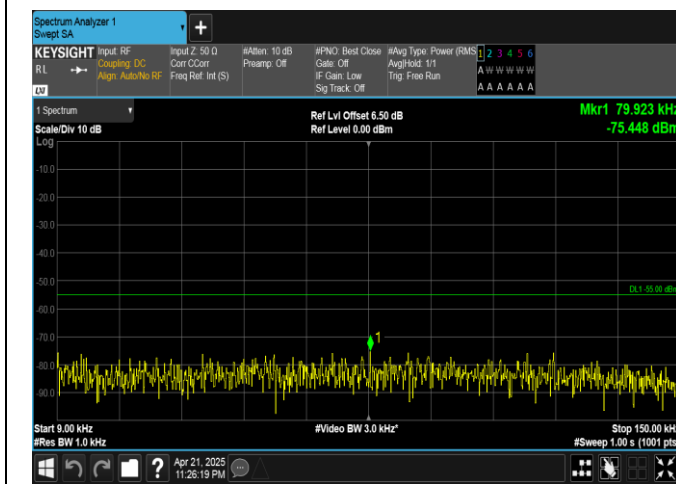
Band41-20MHz-QPSK-41490-100RB#0-0.009~0.15-PASS
