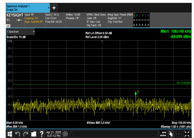
Band41-20MHz-QPSK-41490-1RB#99-0.009~0.15-PASS
