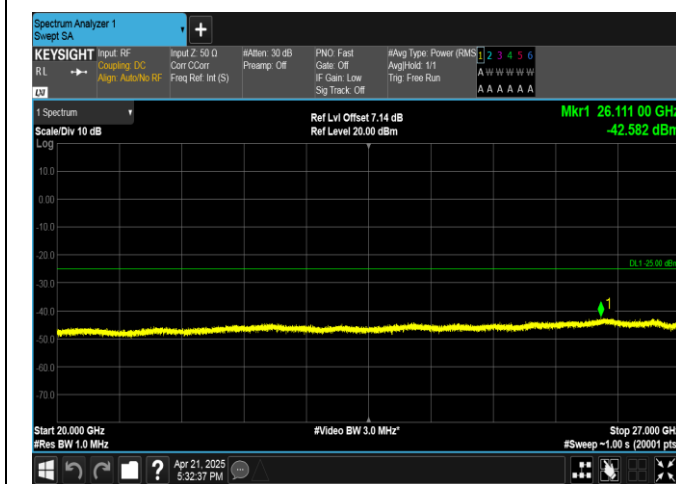
Band41-20MHz-16QAM-40620-1RB#0-20000~27000-PASS
