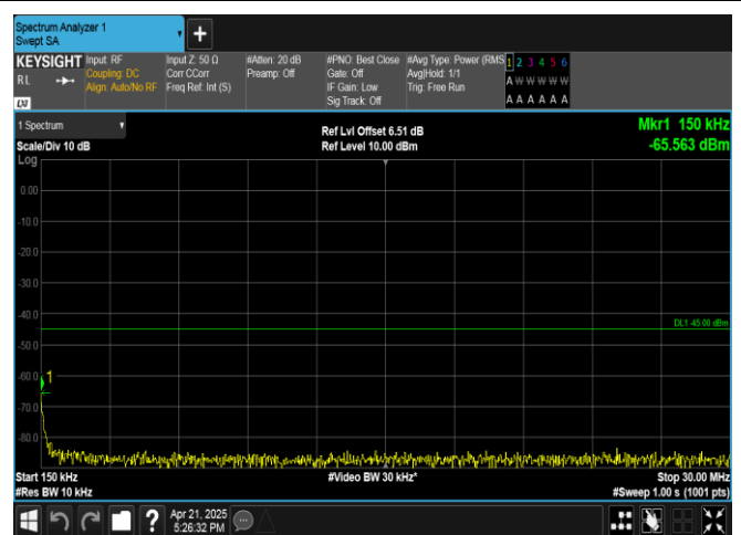
Band41-20MHz-QPSK-39750-1RB#0-0.15~30-PASS
