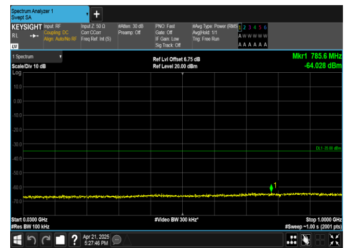
Band41-20MHz-16QAM-39750-1RB#0-30~1000-PASS
