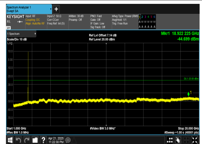
Band41-20MHz-QPSK-39750-100RB#0-1000~20000-PASS
