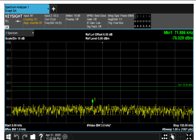
Band41-20MHz-16QAM-39750-100RB#0-0.009~0.15-PASS
