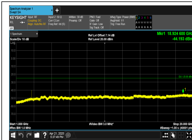
Band41-20MHz-QPSK-41490-1RB#99-1000~20000-PASS
