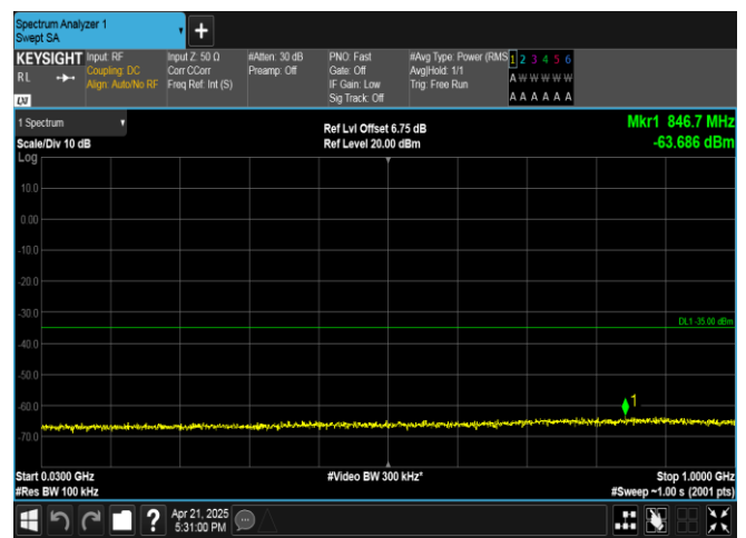
Band41-20MHz-QPSK-40620-1RB#0-30~1000-PASS
