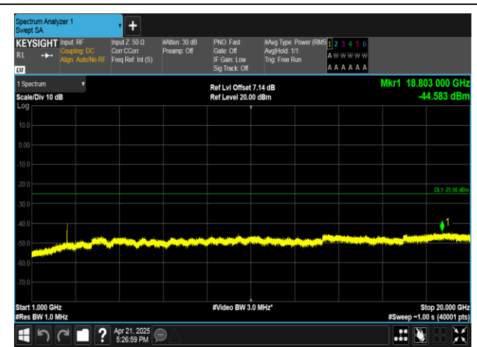
Band41-20MHz-QPSK-39750-1RB#0-1000~20000-PASS
