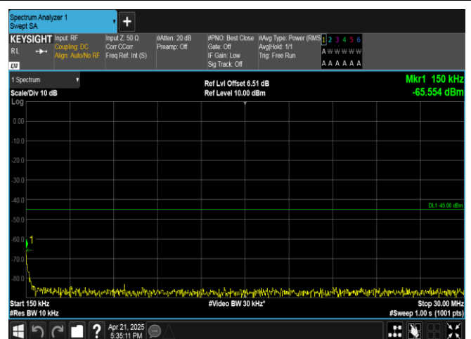
Band41-20MHz-QPSK-41490-1RB#0-0.15~30-PASS
