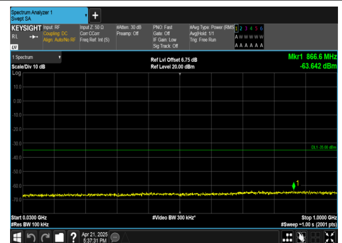
Band41-20MHz-QPSK-41490-1RB#99-30~1000-PASS
