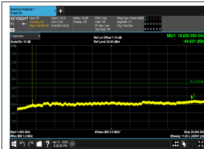
Band41-20MHz-QPSK-39750-1RB#99-1000~20000-PASS
