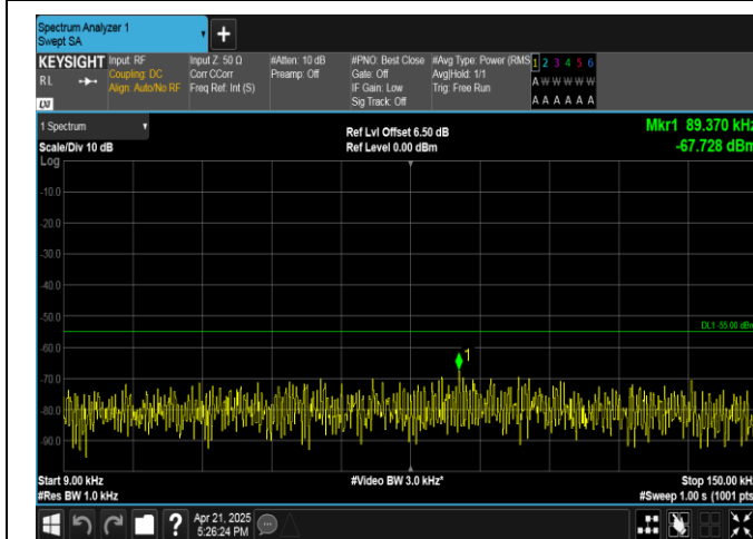
Band41-20MHz-QPSK-39750-1RB#0-0.009~0.15-PASS
