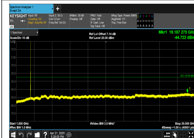
Band41-20MHz-16QAM-39750-1RB#0-1000~20000-PASS
