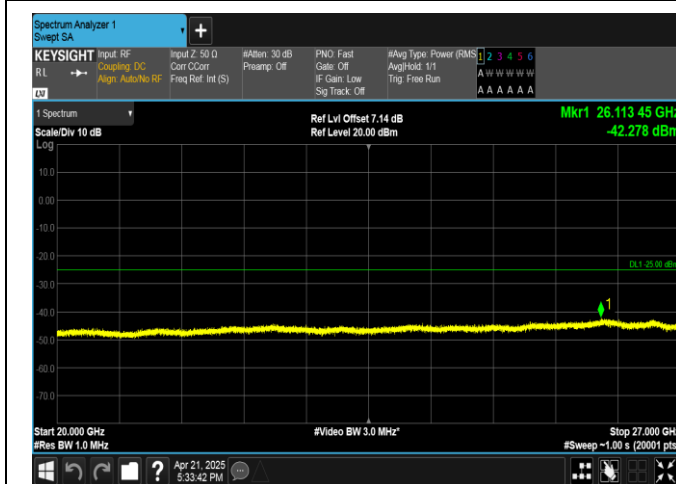
Band41-20MHz-QPSK-40620-1RB#99-20000~27000-PASS
