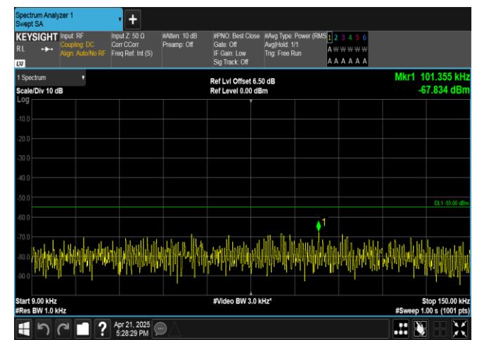
Band41-20MHz-QPSK-39750-1RB#99-0.009~0.15-PASS
