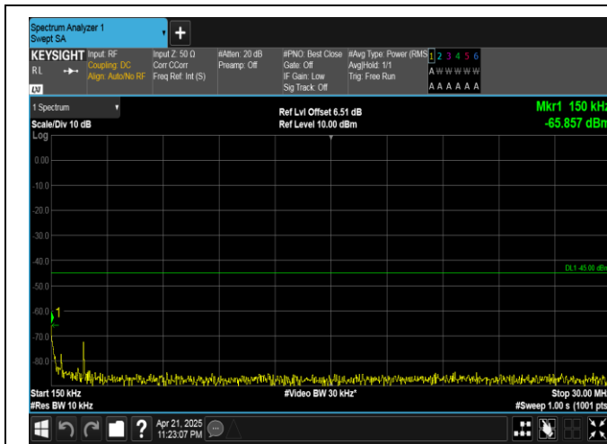
Band41-20MHz-16QAM-39750-100RB#0-0.15~30-PASS
