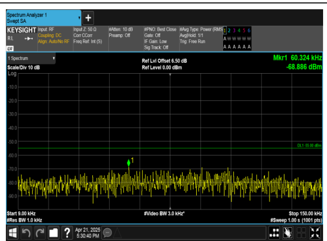
Band41-20MHz-QPSK-40620-1RB#0-0.009~0.15-PASS
