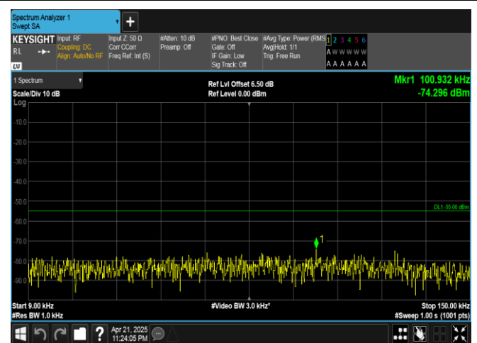
Band41-20MHz-QPSK-40620-100RB#0-0.009~0.15-PASS
