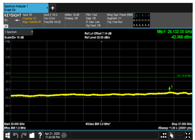
Band41-20MHz-QPSK-40620-100RB#0-20000~27000-PASS
