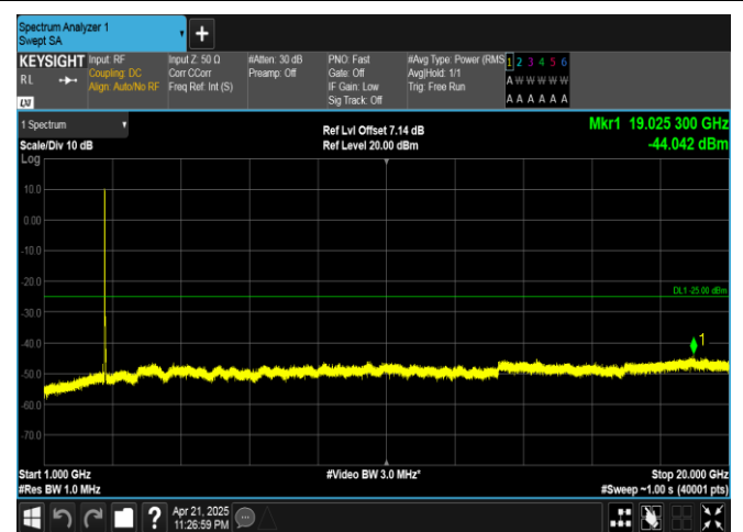
Band41-20MHz-QPSK-41490-100RB#0-1000~20000-PASS
