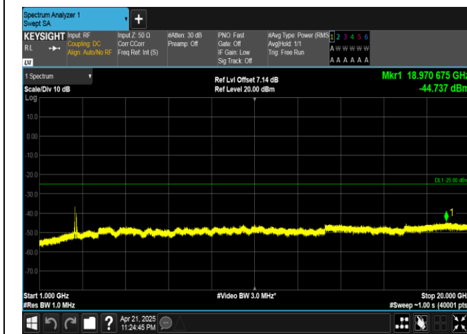
Band41-20MHz-QPSK-40620-100RB#0-1000~20000-PASS
