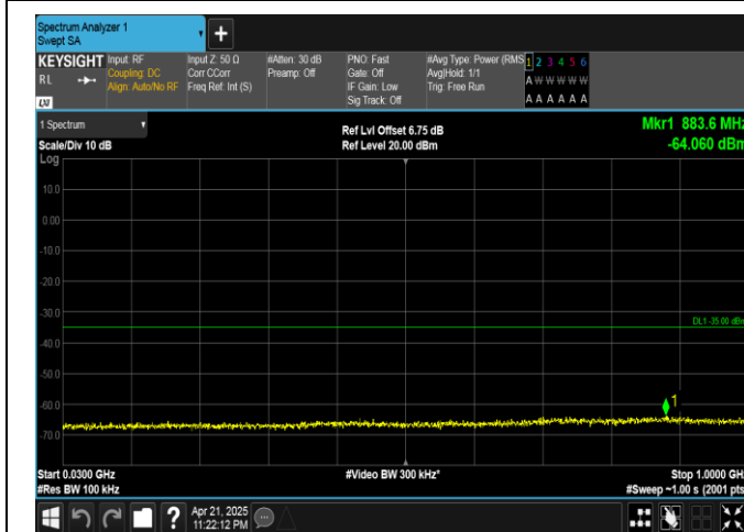
Band41-20MHz-QPSK-39750-100RB#0-30~1000-PASS
