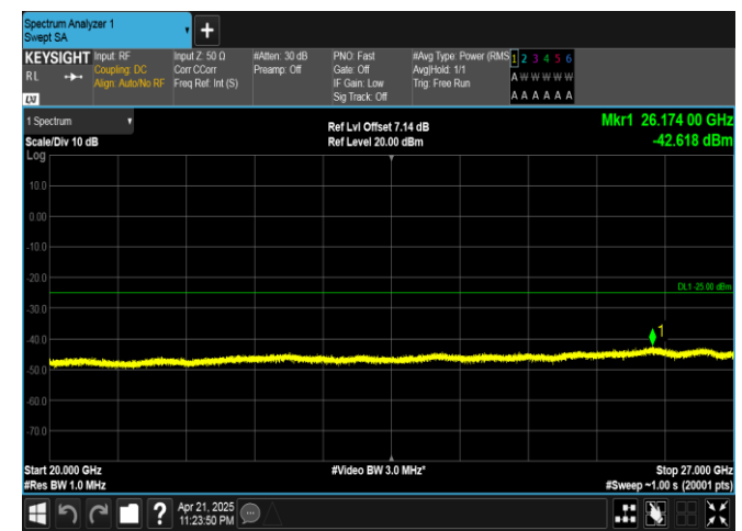
Band41-20MHz-16QAM-39750-100RB#0-20000~27000-PASS
