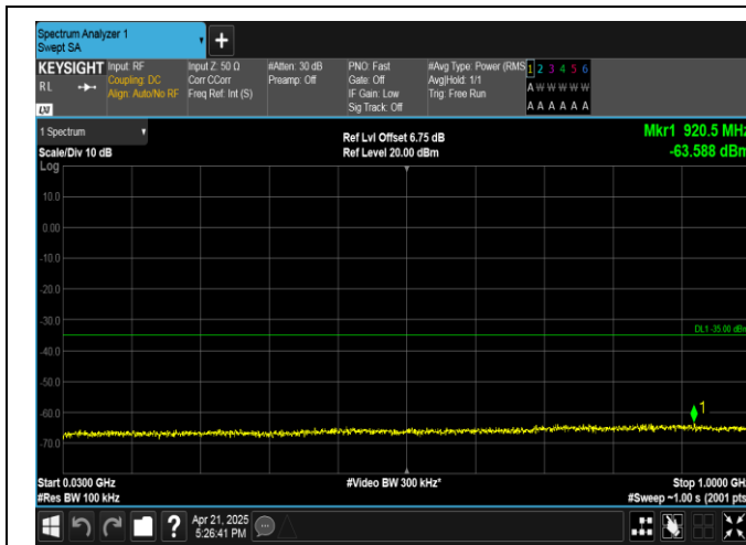
Band41-20MHz-QPSK-39750-1RB#0-30~1000-PASS
