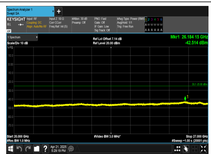
Band41-20MHz-QPSK-39750-1RB#99-20000~27000-PASS
