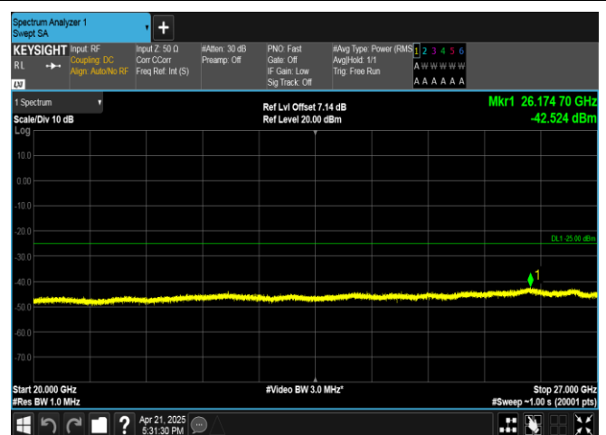
Band41-20MHz-QPSK-40620-1RB#0-20000~27000-PASS
