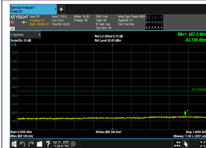
Band41-20MHz-QPSK-41490-100RB#0-30~1000-PASS
