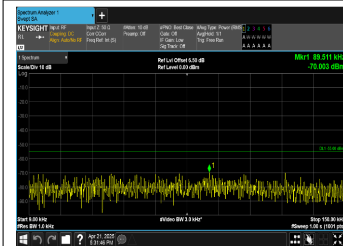
Band41-20MHz-16QAM-40620-1RB#0-0.009~0.15-PASS
