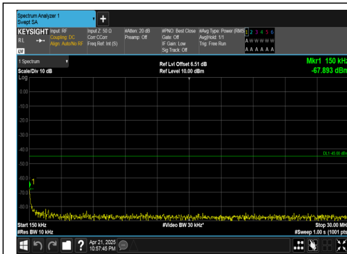
Band41-15MHz-16QAM-41515-75RB#0-0.15~30-PASS
