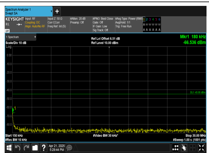
Band41-20MHz-16QAM-39750-1RB#99-0.15~30-PASS
