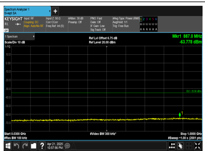
Band41-15MHz-16QAM-41515-75RB#0-30~1000-PASS
