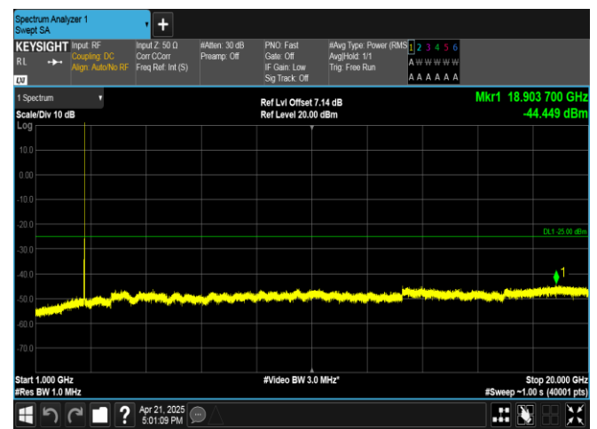
Band41-15MHz-16QAM-41515-1RB#74-1000~20000-PASS
