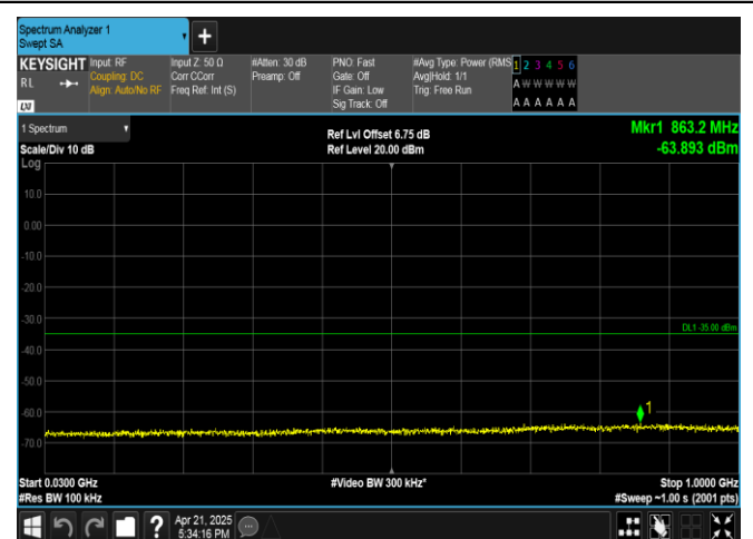
Band41-20MHz-16QAM-40620-1RB#99-30~1000-PASS
