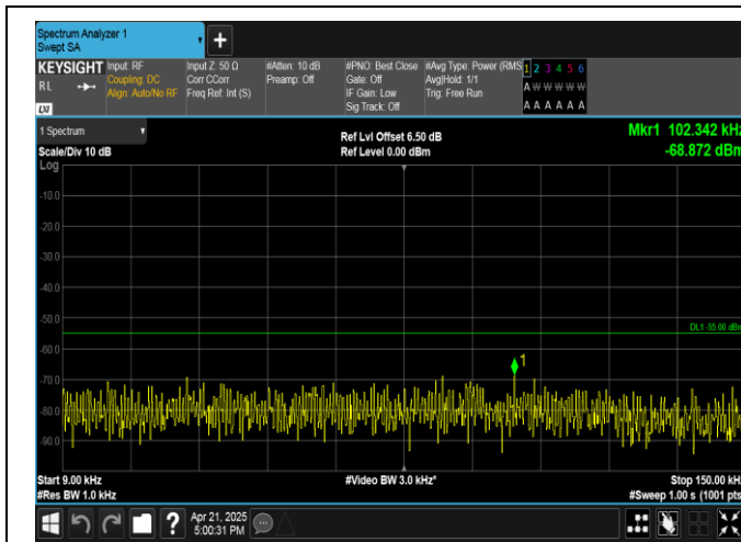
Band41-15MHz-16QAM-41515-1RB#74-0.009~0.15-PASS
