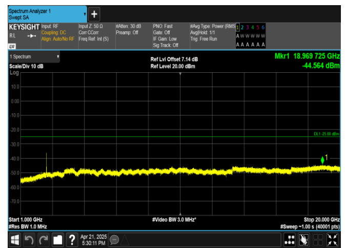
Band41-20MHz-16QAM-39750-1RB#99-1000~20000-PASS
