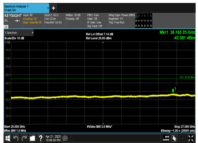
Band41-15MHz-16QAM-41515-75RB#0-20000~27000-PASS
