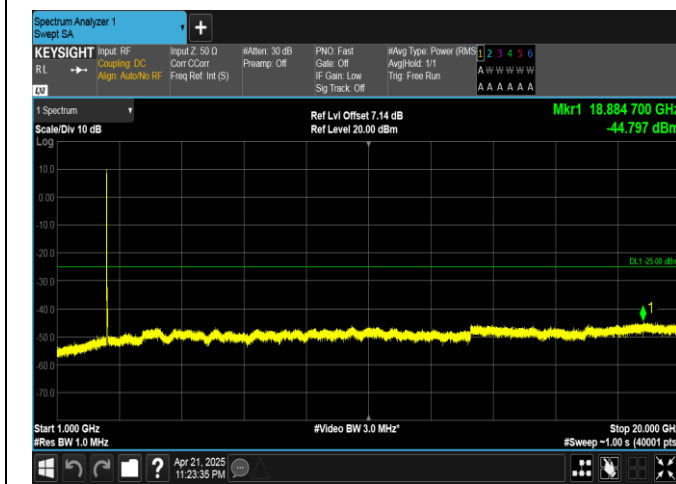
Band41-20MHz-16QAM-39750-100RB#0-1000~20000-PASS
