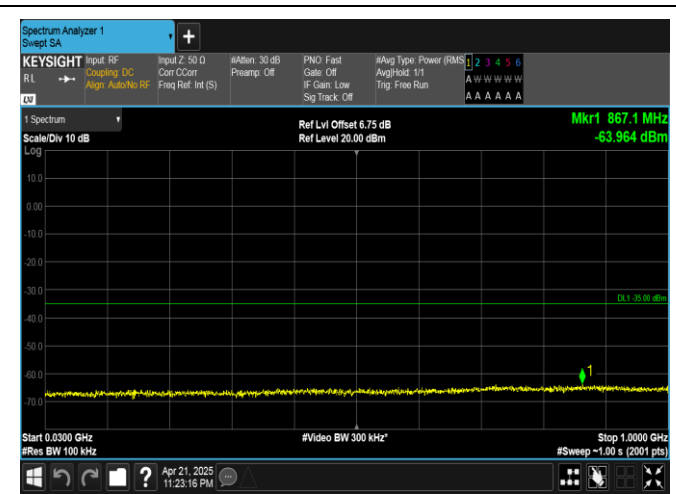
Band41-20MHz-16QAM-39750-100RB#0-30~1000-PASS
