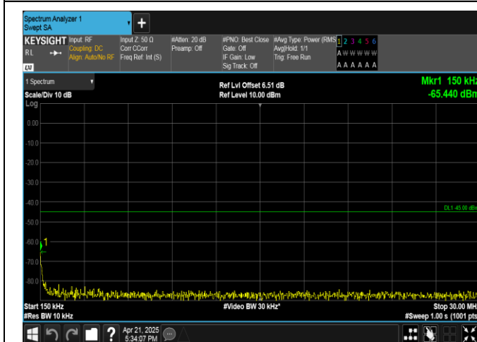
Band41-20MHz-16QAM-40620-1RB#99-0.15~30-PASS
