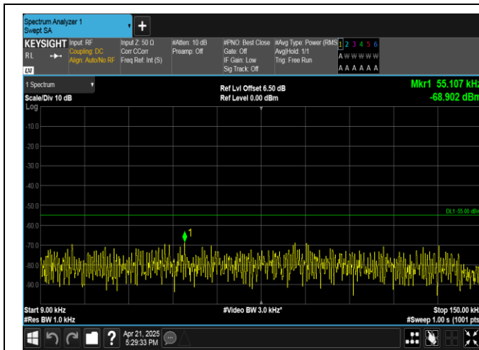
Band41-20MHz-16QAM-39750-1RB#99-0.009~0.15-PASS
