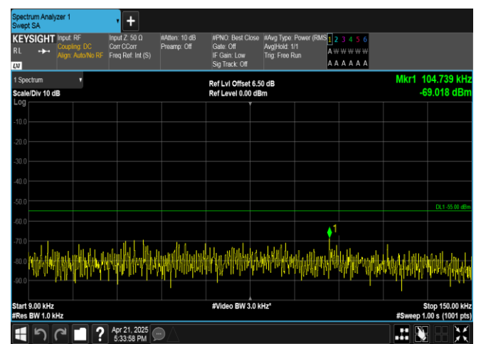
Band41-20MHz-16QAM-40620-1RB#99-0.009~0.15-PASS
