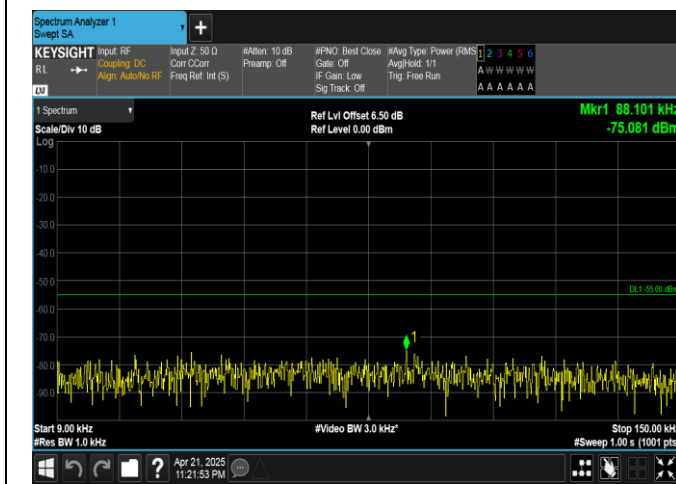
Band41-20MHz-QPSK-39750-100RB#0-0.009~0.15-PASS
