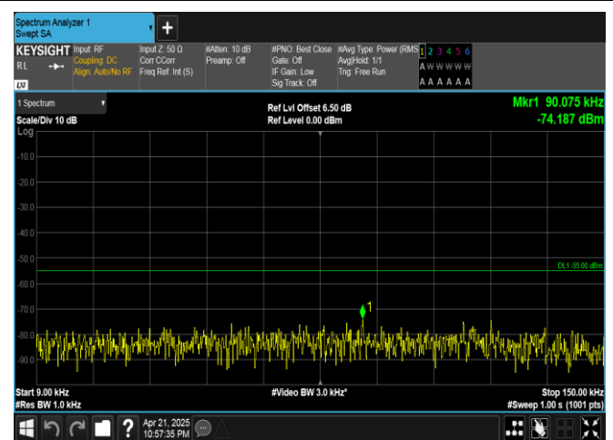
Band41-15MHz-16QAM-41515-75RB#0-0.009~0.15-PASS
