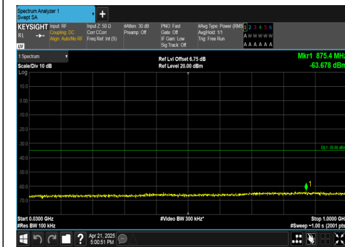
Band41-15MHz-16QAM-41515-1RB#74-30~1000-PASS
