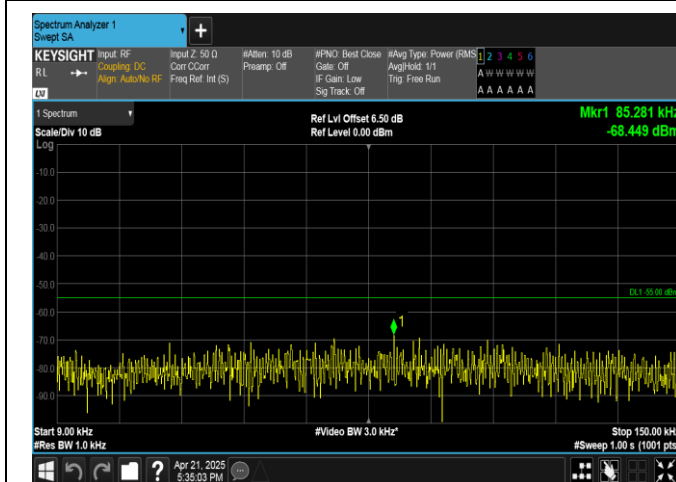
Band41-20MHz-QPSK-41490-1RB#0-0.009~0.15-PASS
