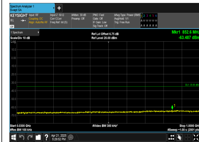
Band41-20MHz-16QAM-39750-1RB#99-30~1000-PASS
