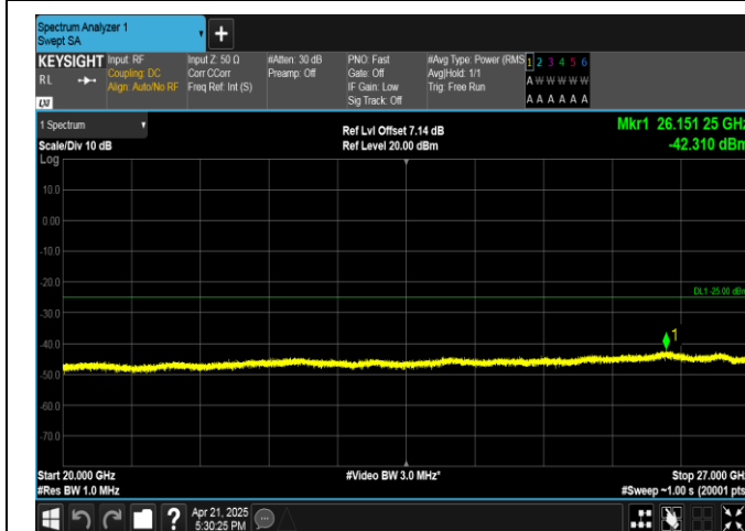
Band41-20MHz-16QAM-39750-1RB#99-20000~27000-PASS
