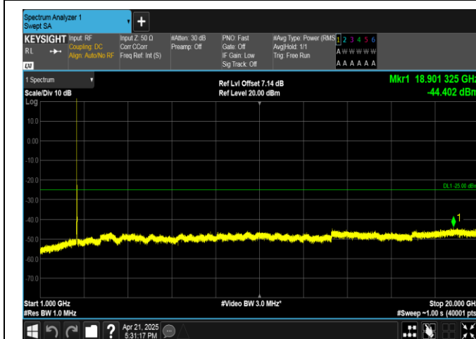
Band41-20MHz-QPSK-40620-1RB#0-1000~20000-PASS
