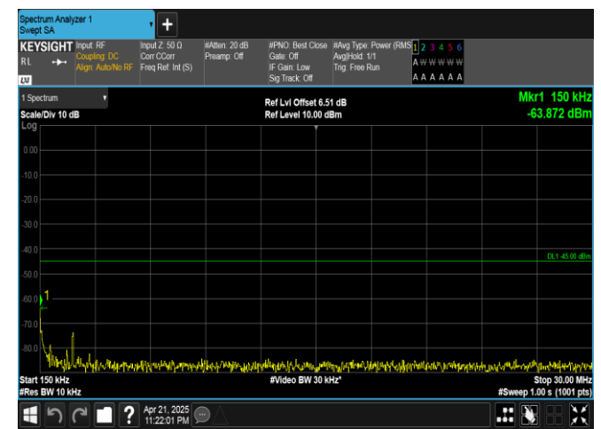
Band41-20MHz-QPSK-39750-100RB#0-0.15~30-PASS
