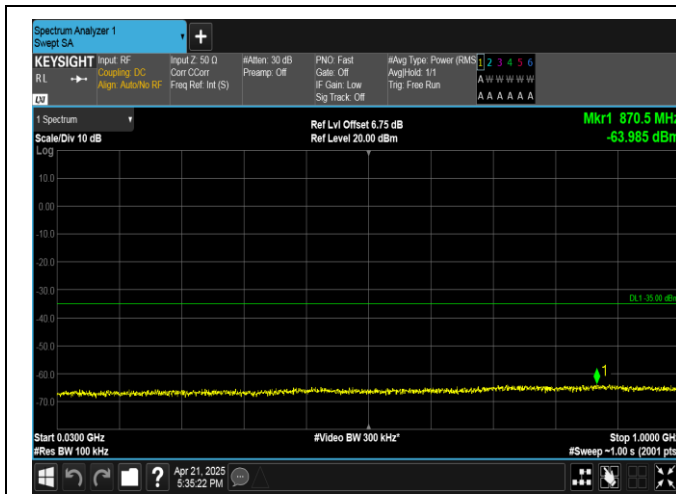
Band41-20MHz-QPSK-41490-1RB#0-30~1000-PASS
