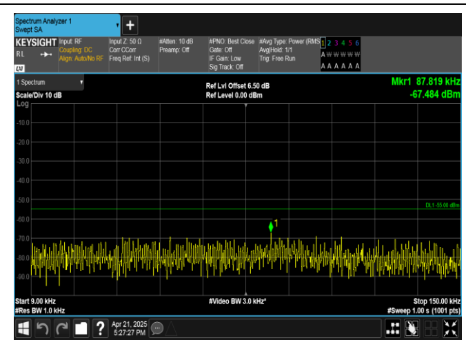
Band41-20MHz-16QAM-39750-1RB#0-0.009~0.15-PASS
