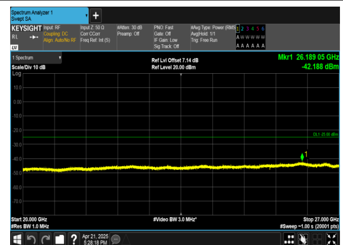
Band41-20MHz-16QAM-39750-1RB#0-20000~27000-PASS
