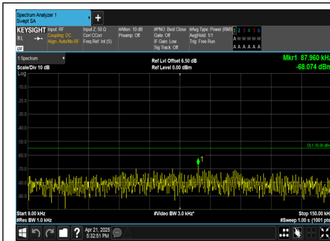
Band41-20MHz-QPSK-40620-1RB#99-0.009~0.15-PASS
