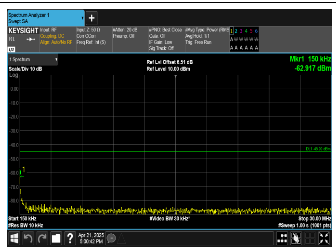
Band41-15MHz-16QAM-41515-1RB#74-0.15~30-PASS
