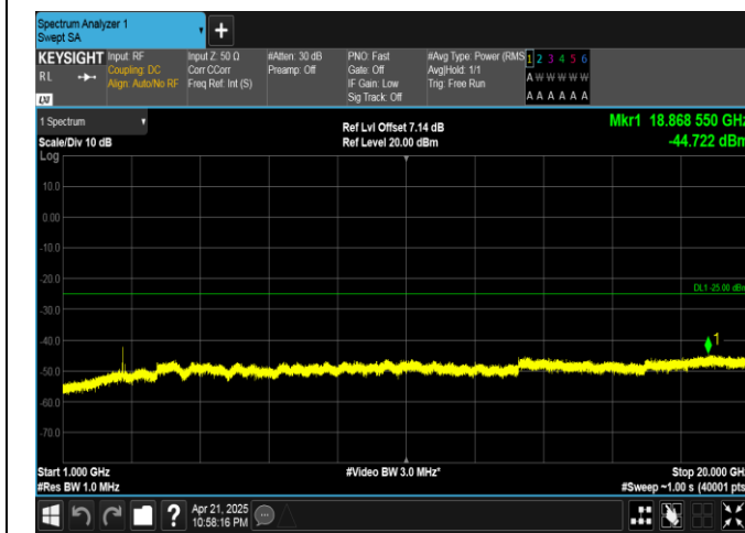
Band41-15MHz-16QAM-41515-75RB#0-1000~20000-PASS
