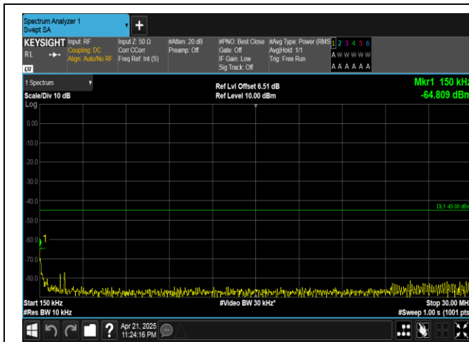
Band41-20MHz-QPSK-40620-100RB#0-0.15~30-PASS
