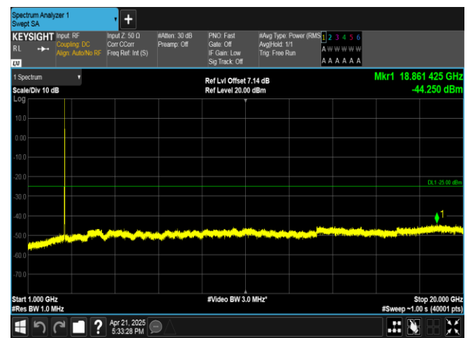
Band41-20MHz-QPSK-40620-1RB#99-1000~20000-PASS
