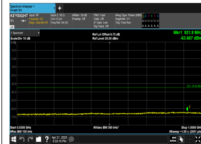
Band41-20MHz-QPSK-40620-1RB#99-30~1000-PASS
