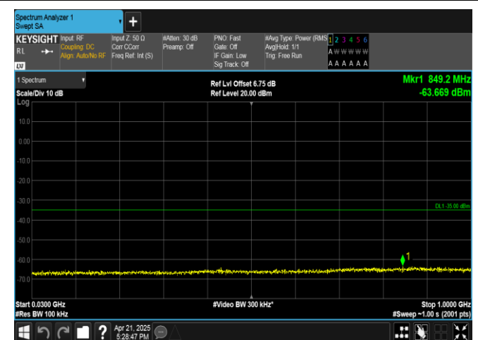
Band41-20MHz-QPSK-39750-1RB#99-30~1000-PASS
