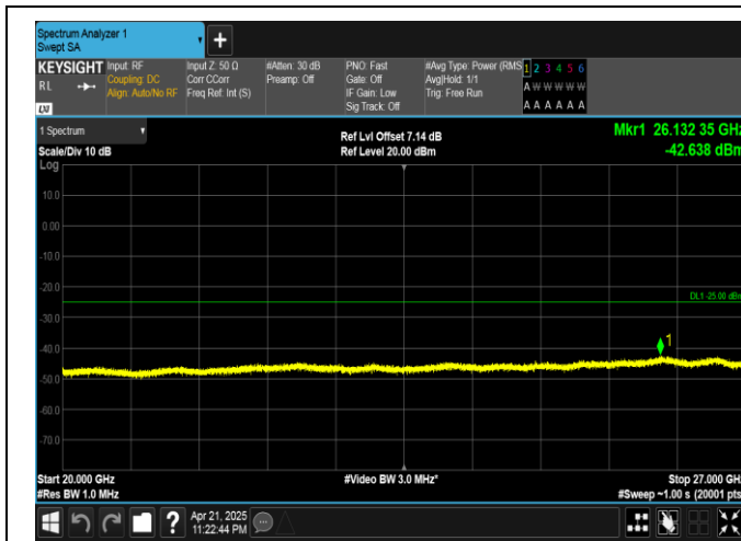
Band41-20MHz-QPSK-39750-100RB#0-20000~27000-PASS
