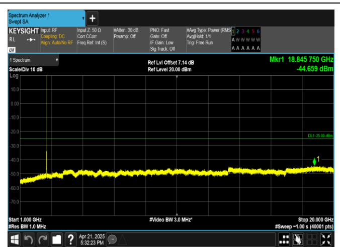
Band41-20MHz-16QAM-40620-1RB#0-1000~20000-PASS
