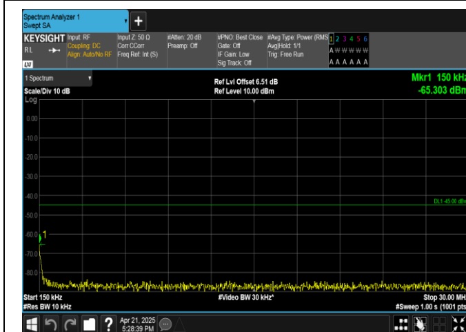
Band41-20MHz-QPSK-39750-1RB#99-0.15~30-PASS
