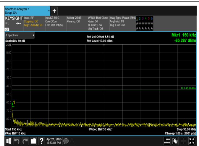
Band41-20MHz-QPSK-40620-1RB#99-0.15~30-PASS
