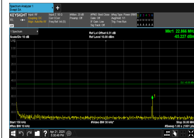
Band41-20MHz-QPSK-40620-1RB#0-0.15~30-PASS
