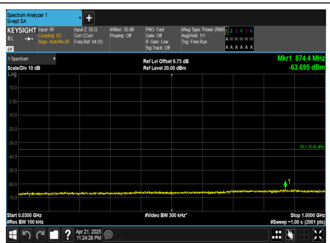
Band41-20MHz-QPSK-40620-100RB#0-30~1000-PASS
