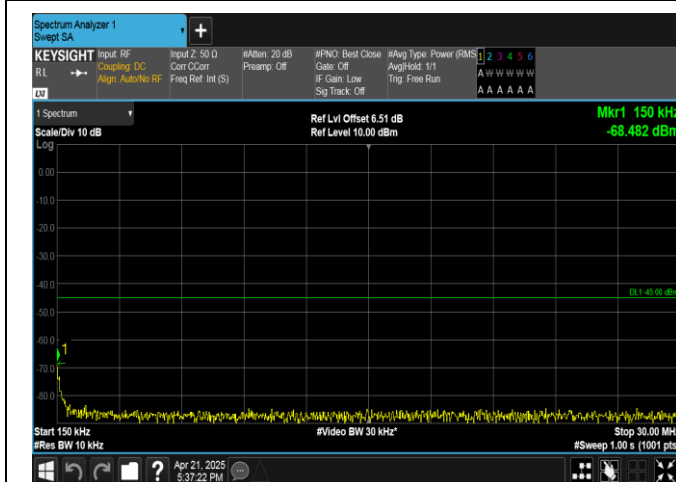
Band41-20MHz-QPSK-41490-1RB#99-0.15~30-PASS
