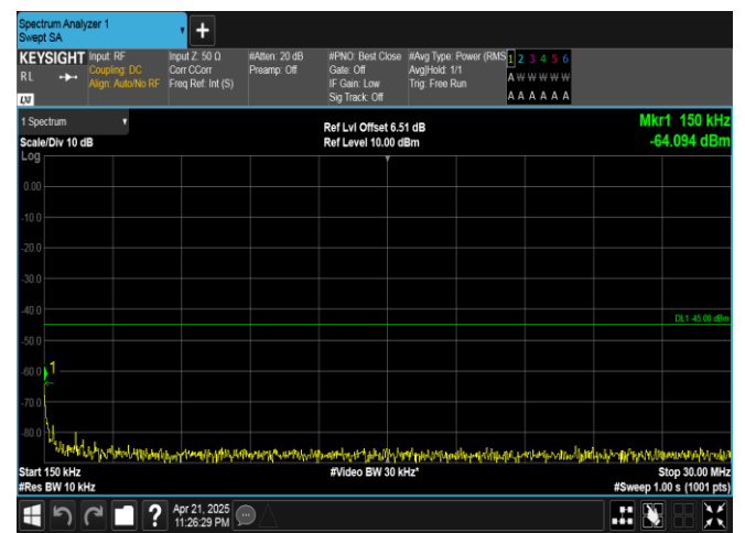
Band41-20MHz-QPSK-41490-100RB#0-0.15~30-PASS
