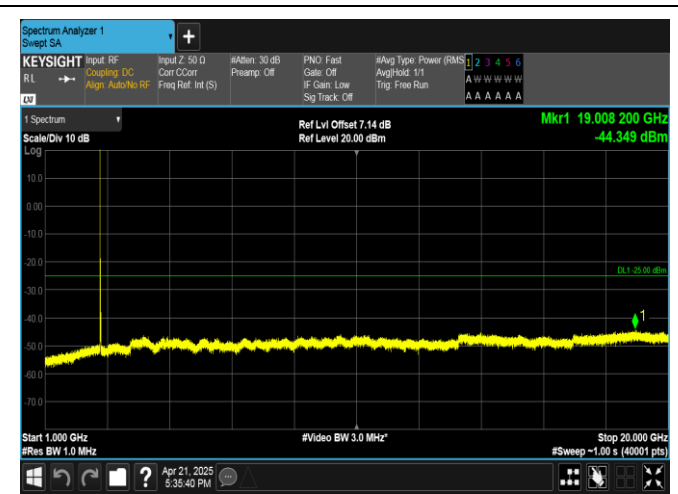
Band41-20MHz-QPSK-41490-1RB#0-1000~20000-PASS
