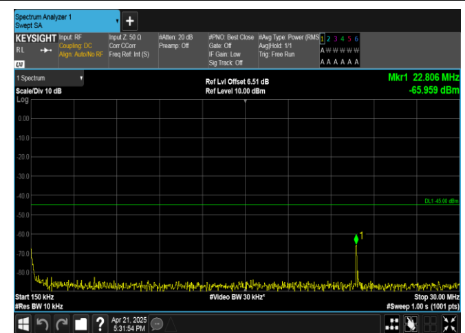
Band41-20MHz-16QAM-40620-1RB#0-0.15~30-PASS
