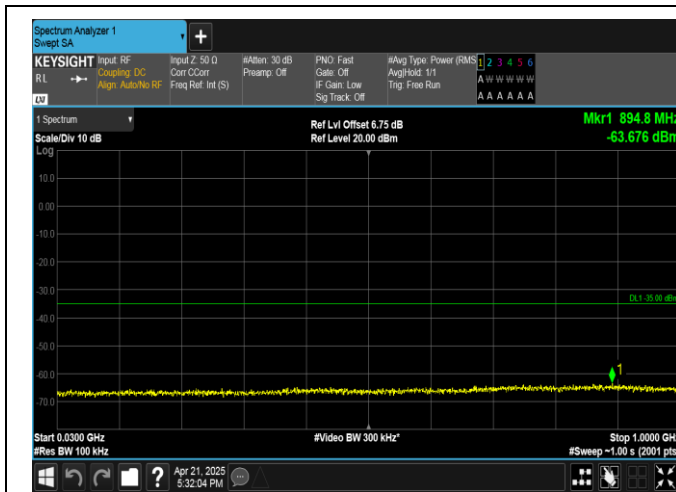
Band41-20MHz-16QAM-40620-1RB#0-30~1000-PASS
