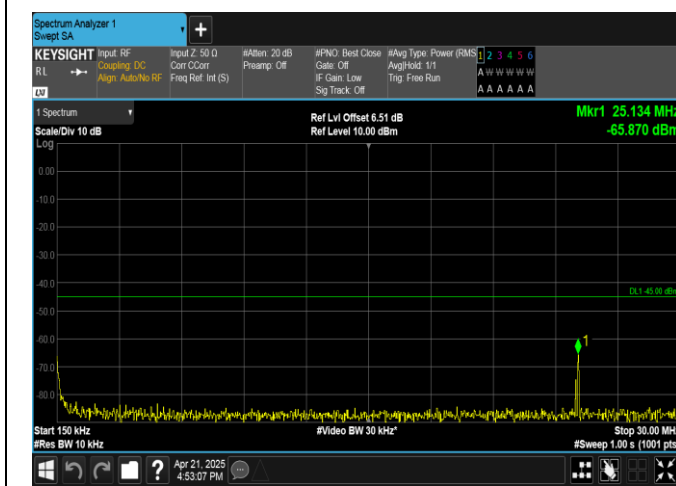
Band41-15MHz-QPSK-40620-1RB#0-0.15~30-PASS
