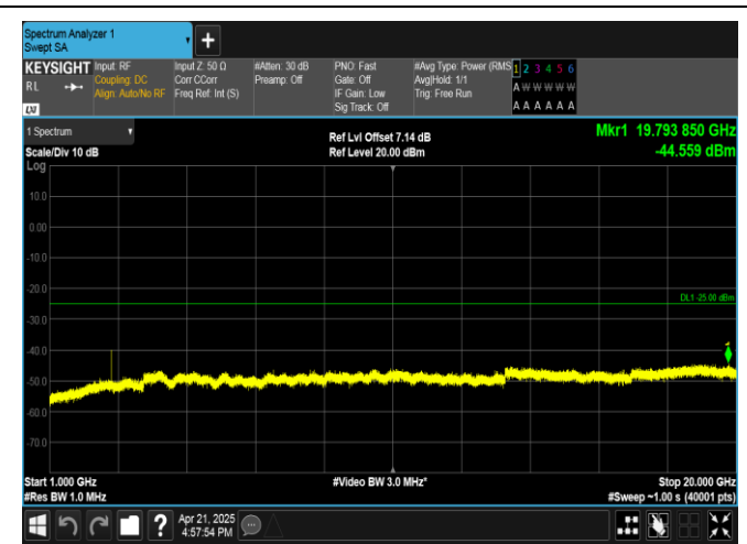
Band41-15MHz-QPSK-41515-1RB#0-1000~20000-PASS
