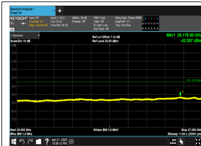
Band41-15MHz-16QAM-40620-75RB#0-20000~27000-PASS
