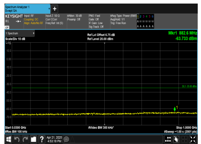
Band41-15MHz-QPSK-40620-1RB#0-30~1000-PASS
