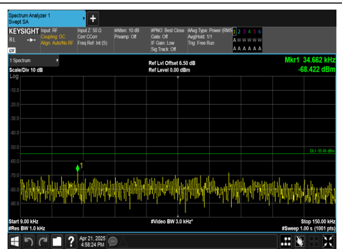
Band41-15MHz-16QAM-41515-1RB#0-0.009~0.15-PASS
