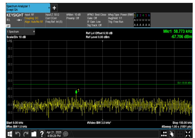
Band41-15MHz-QPSK-41515-1RB#74-0.009~0.15-PASS
