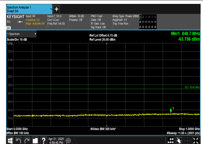
Band41-15MHz-QPSK-41515-1RB#74-30~1000-PASS
