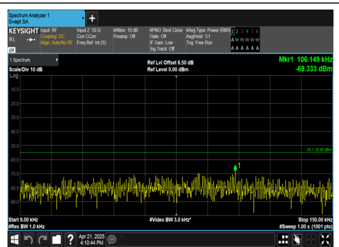
Band41-10MHz-QPSK-40620-1RB#0-0.009~0.15-PASS
