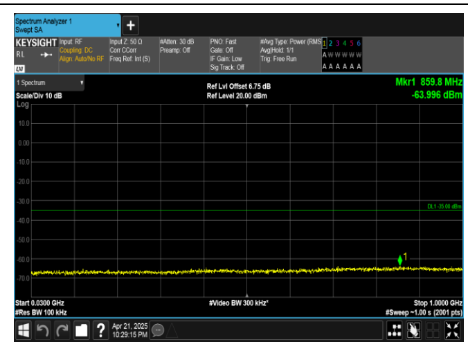
Band41-10MHz-QPSK-40620-50RB#0-30~1000-PASS
