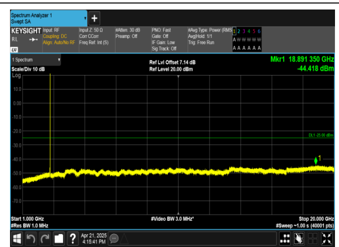
Band41-10MHz-QPSK-41540-1RB#0-1000~20000-PASS
