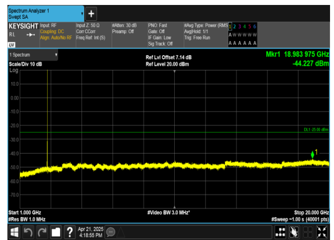
Band41-10MHz-16QAM-41540-1RB#49-1000~20000-PASS
