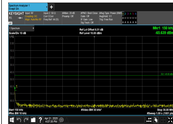
Band41-10MHz-16QAM-39700-1RB#0-0.15~30-PASS
