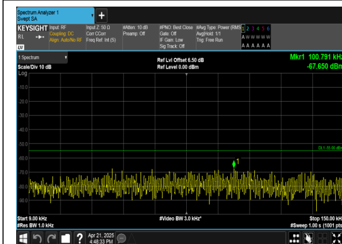
Band41-15MHz-QPSK-39725-1RB#0-0.009~0.15-PASS
