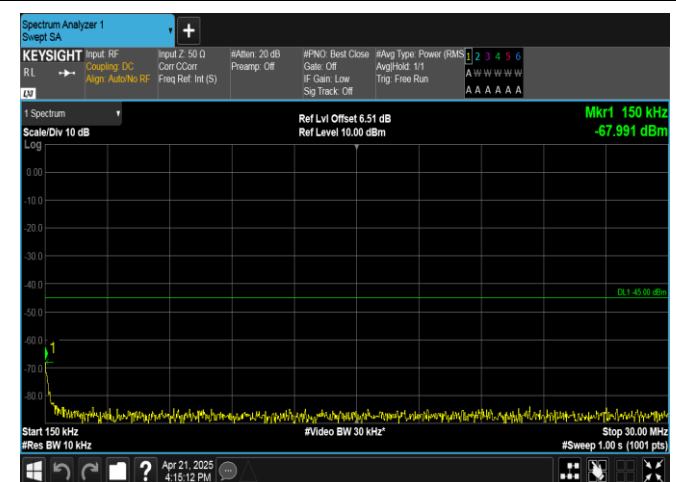
Band41-10MHz-QPSK-41540-1RB#0-0.15~30-PASS
