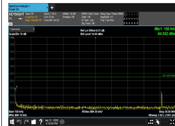
Band41-10MHz-QPSK-40620-1RB#0-0.15~30-PASS
