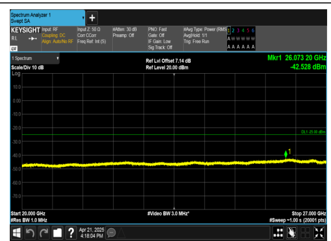
Band41-10MHz-QPSK-41540-1RB#49-20000~27000-PASS
