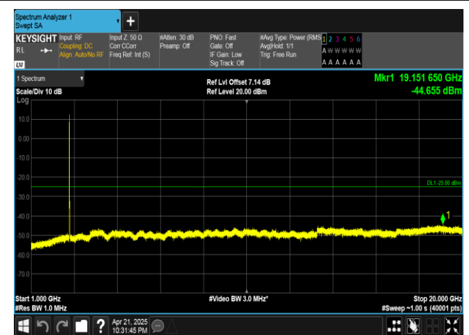
Band41-10MHz-QPSK-41540-50RB#0-1000~20000-PASS
