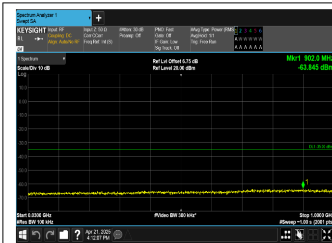
Band41-10MHz-16QAM-40620-1RB#0-30~1000-PASS
