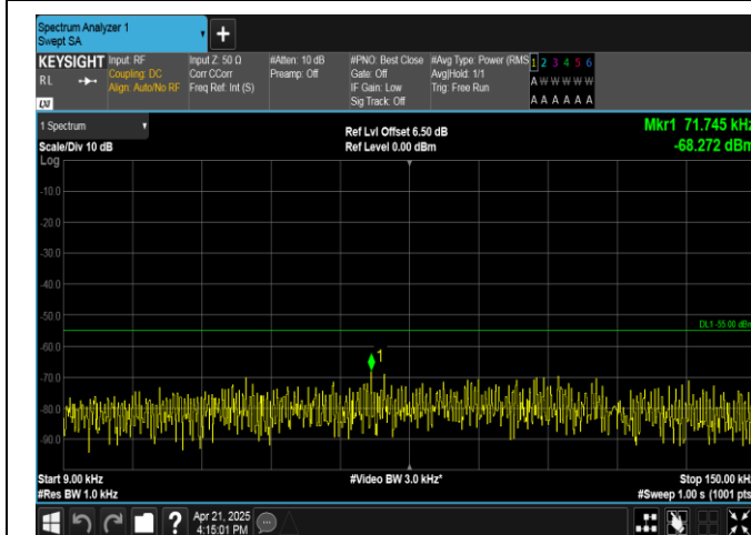
Band41-10MHz-QPSK-41540-1RB#0-0.009~0.15-PASS
