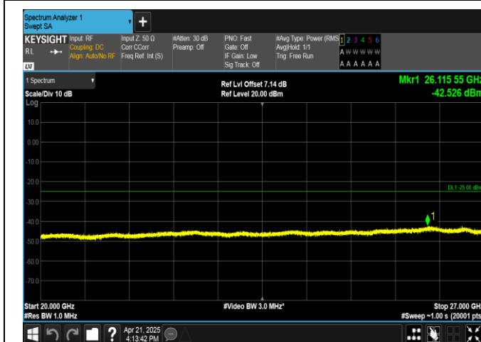
Band41-10MHz-QPSK-40620-1RB#49-20000~27000-PASS
