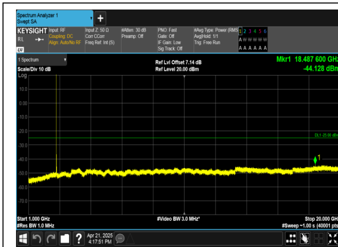
Band41-10MHz-QPSK-41540-1RB#49-1000~20000-PASS
