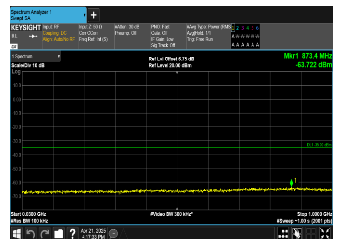
Band41-10MHz-QPSK-41540-1RB#49-30~1000-PASS
