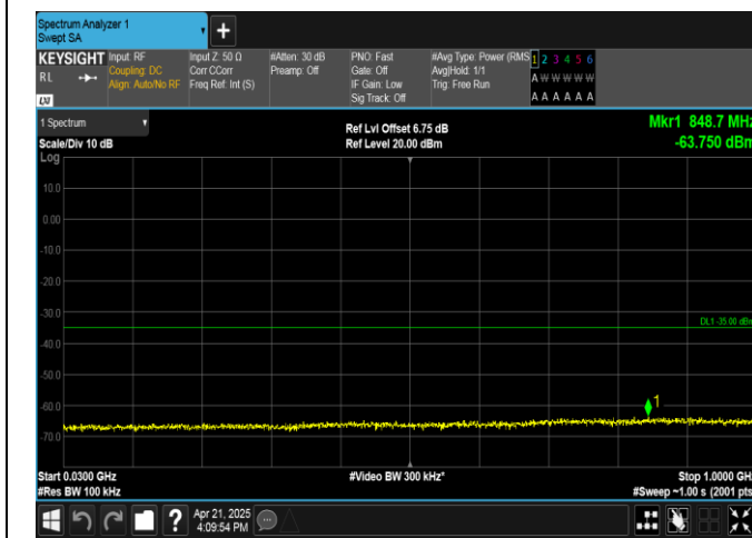
Band41-10MHz-16QAM-39700-1RB#49-30~1000-PASS
