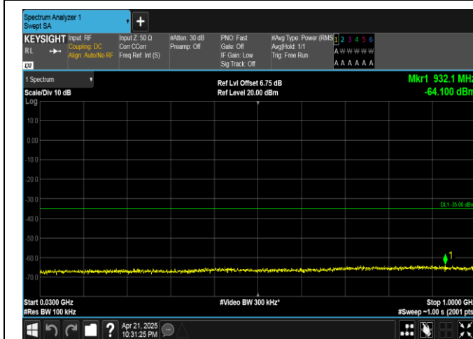
Band41-10MHz-QPSK-41540-50RB#0-30~1000-PASS
