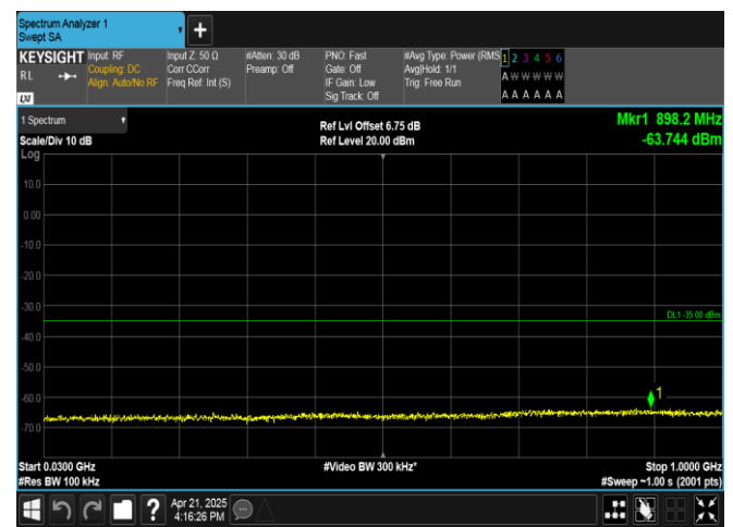
Band41-10MHz-16QAM-41540-1RB#0-30~1000-PASS
