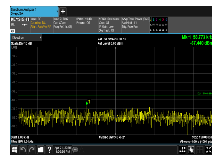
Band41-10MHz-16QAM-39700-1RB#49-0.009~0.15-PASS
