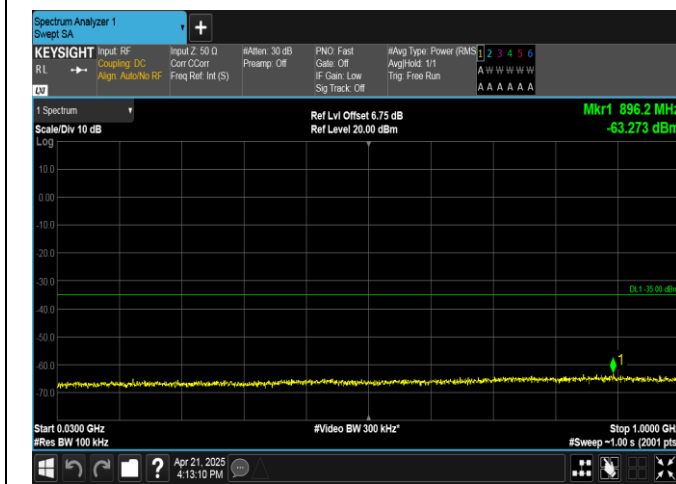
Band41-10MHz-QPSK-40620-1RB#49-30~1000-PASS
