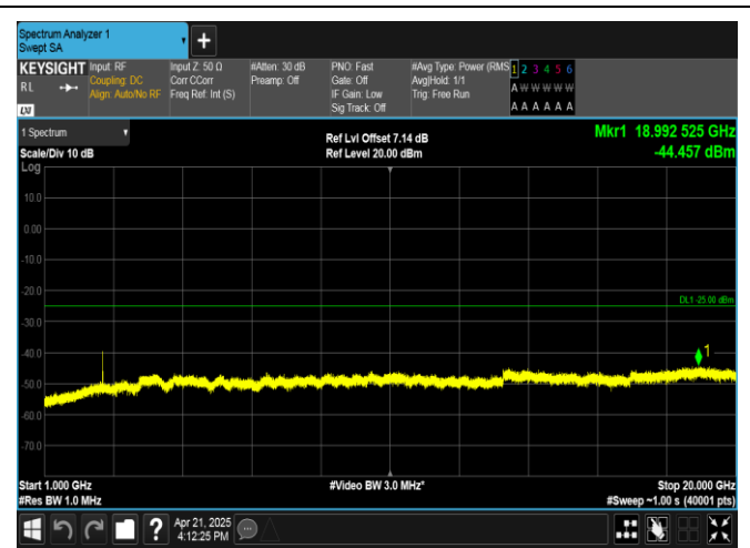
Band41-10MHz-16QAM-40620-1RB#0-1000~20000-PASS
