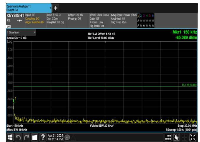
Band41-10MHz-QPSK-41540-50RB#0-0.15~30-PASS
