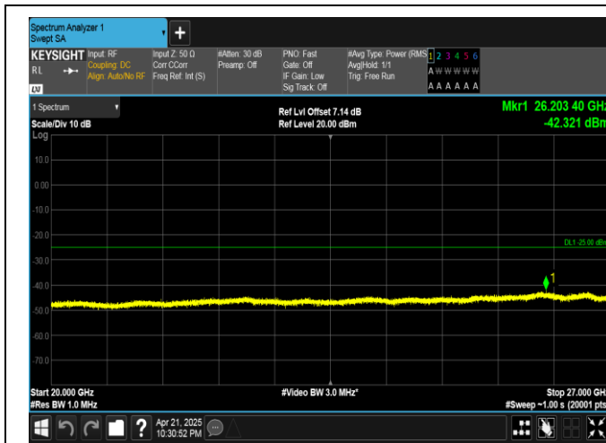
Band41-10MHz-16QAM-40620-50RB#0-20000~27000-PASS
