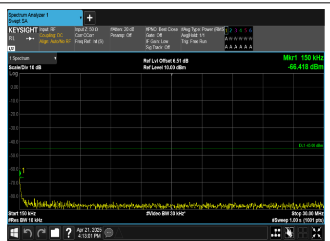
Band41-10MHz-QPSK-40620-1RB#49-0.15~30-PASS
