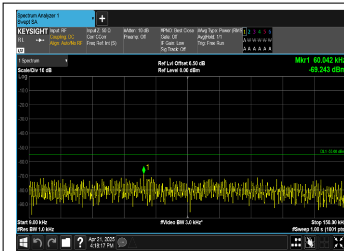
Band41-10MHz-16QAM-41540-1RB#49-0.009~0.15-PASS
