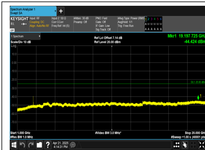
Band41-10MHz-16QAM-40620-1RB#49-1000~20000-PASS
