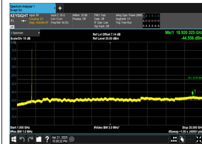
Band41-10MHz-16QAM-39700-50RB#0-1000~20000-PASS
