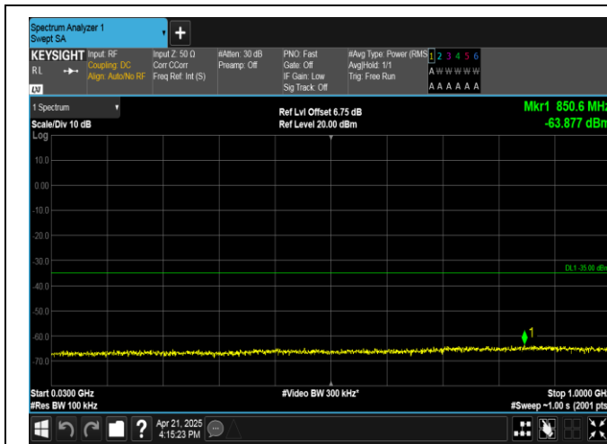
Band41-10MHz-QPSK-41540-1RB#0-30~1000-PASS
