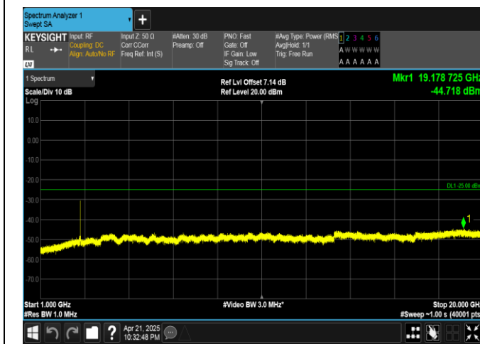
Band41-10MHz-16QAM-41540-50RB#0-1000~20000-PASS
