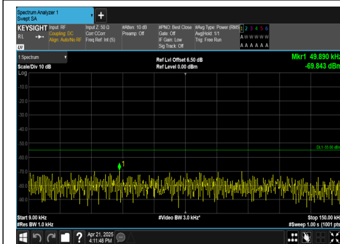
Band41-10MHz-16QAM-40620-1RB#0-0.009~0.15-PASS
