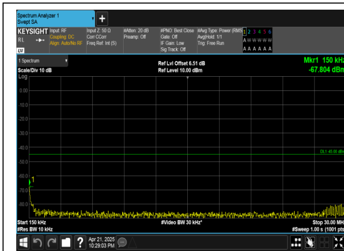
Band41-10MHz-QPSK-40620-50RB#0-0.15~30-PASS
