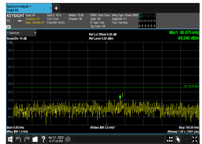
Band41-10MHz-QPSK-41540-1RB#49-0.009~0.15-PASS
