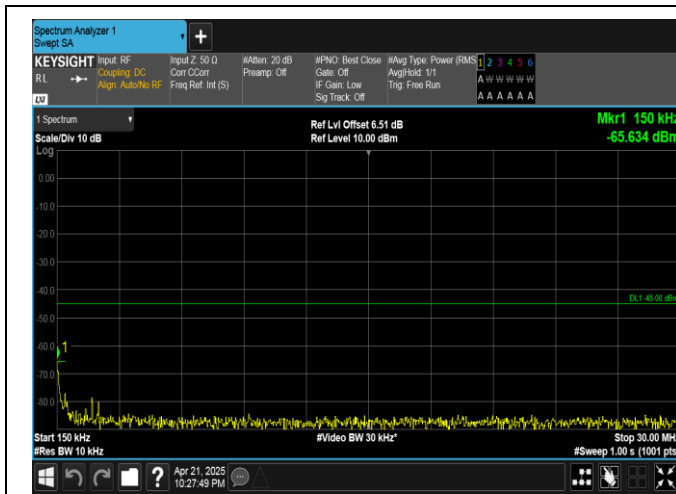
Band41-10MHz-16QAM-39700-50RB#0-0.15~30-PASS
