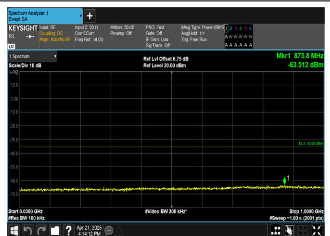
Band41-10MHz-16QAM-40620-1RB#49-30~1000-PASS
