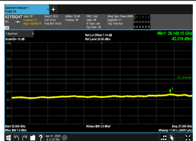
Band41-10MHz-QPSK-40620-1RB#0-20000~27000-PASS
