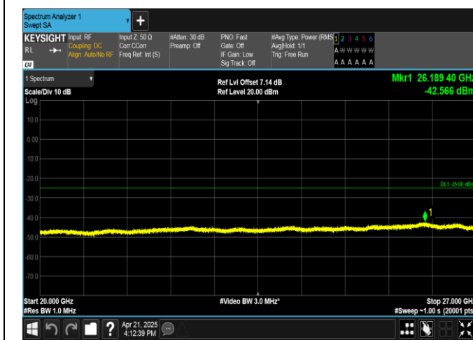
Band41-10MHz-16QAM-40620-1RB#0-20000~27000-PASS
