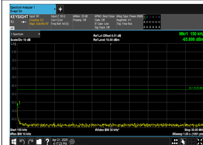
Band41-10MHz-QPSK-41540-1RB#49-0.15~30-PASS
