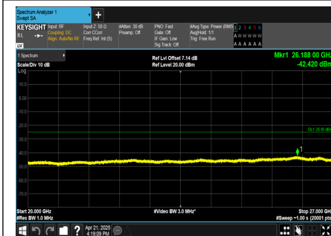
Band41-10MHz-16QAM-41540-1RB#49-20000~27000-PASS
