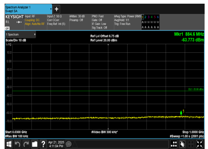
Band41-10MHz-QPSK-40620-1RB#0-30~1000-PASS
