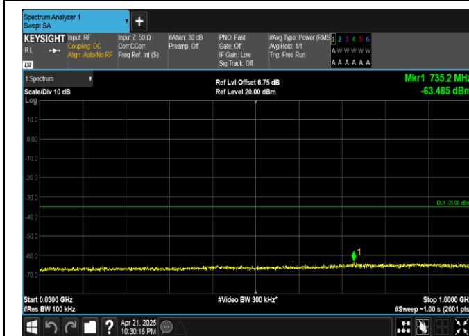
Band41-10MHz-16QAM-40620-50RB#0-30~1000-PASS
