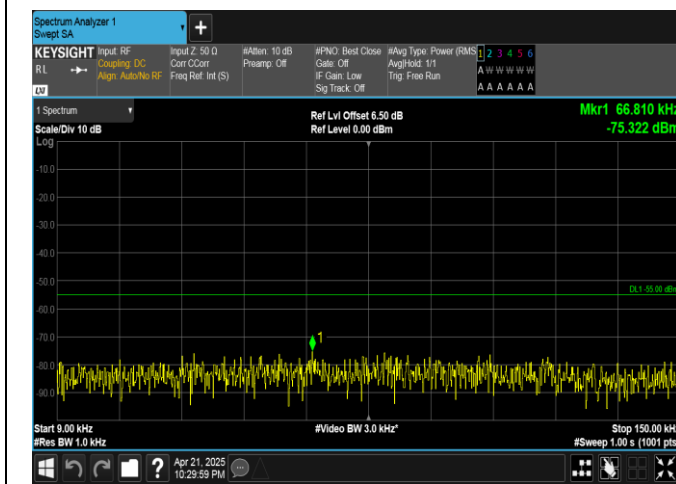
Band41-10MHz-16QAM-40620-50RB#0-0.009~0.15-PASS
