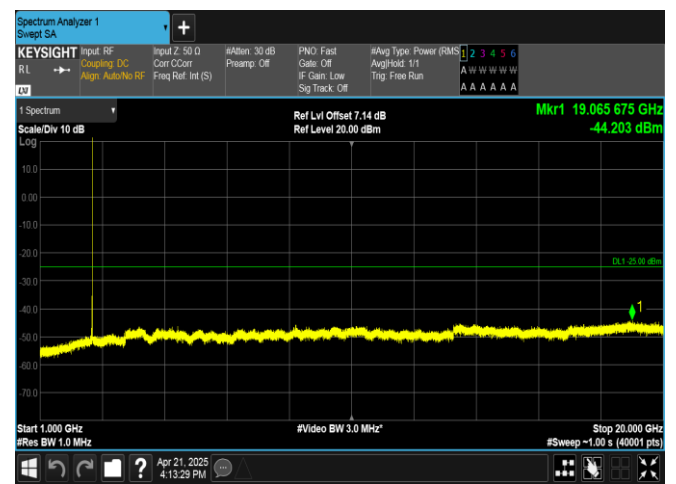
Band41-10MHz-QPSK-40620-1RB#49-1000~20000-PASS
