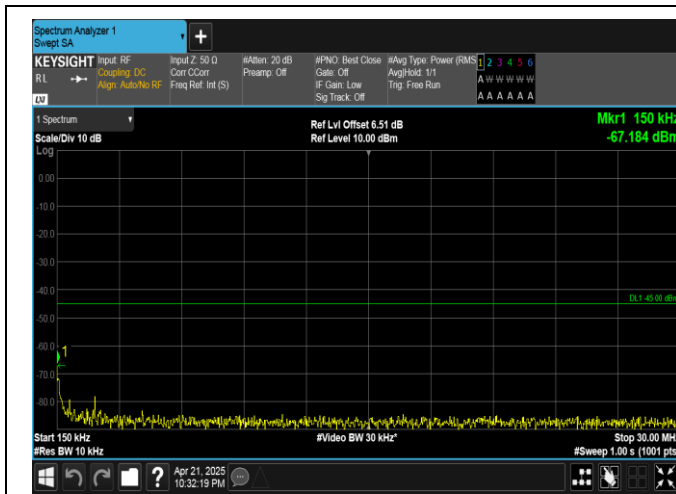
Band41-10MHz-16QAM-41540-50RB#0-0.15~30-PASS
