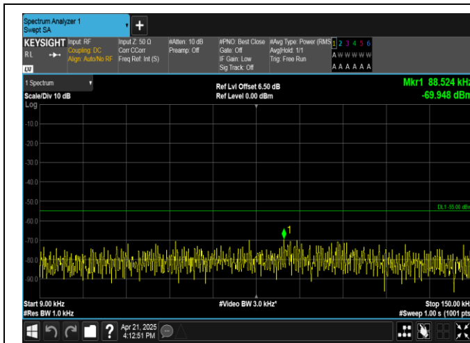
Band41-10MHz-QPSK-40620-1RB#49-0.009~0.15-PASS
