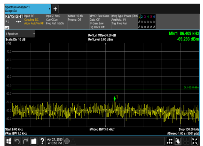
Band41-10MHz-16QAM-40620-1RB#49-0.009~0.15-PASS
