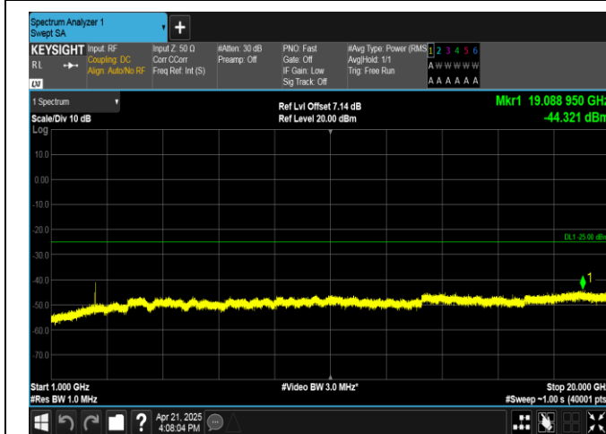
Band41-10MHz-16QAM-39700-1RB#0-1000~20000-PASS
