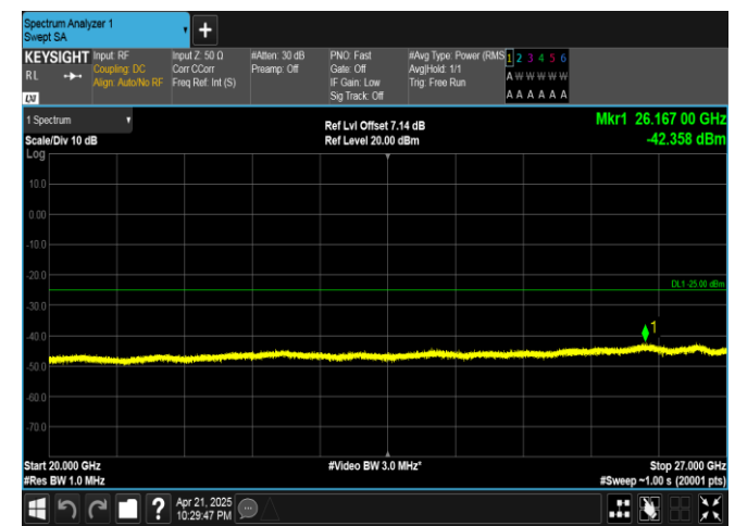
Band41-10MHz-QPSK-40620-50RB#0-20000~27000-PASS
