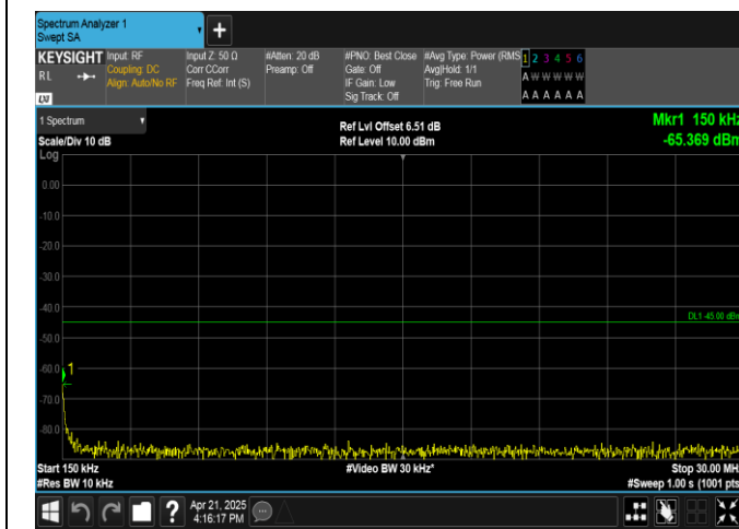
Band41-10MHz-16QAM-41540-1RB#0-0.15~30-PASS
