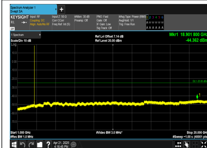
Band41-10MHz-16QAM-41540-1RB#0-1000~20000-PASS
