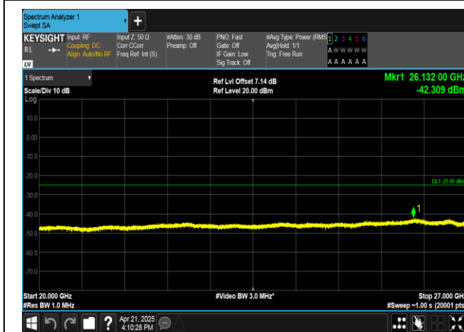
Band41-10MHz-16QAM-39700-1RB#49-20000~27000-PASS
