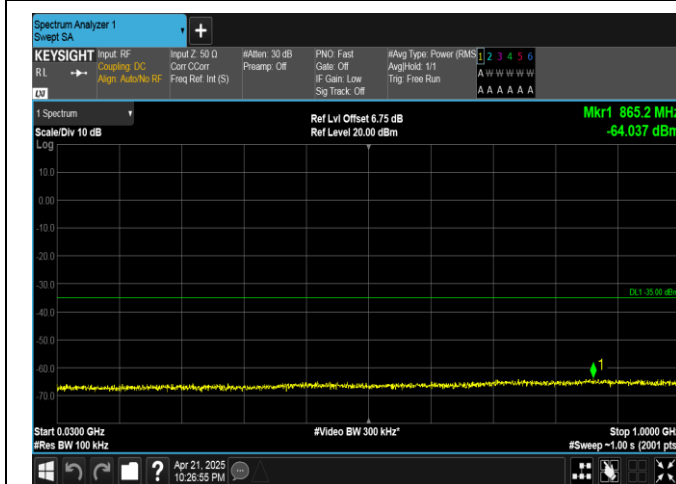
Band41-10MHz-QPSK-39700-50RB#0-30~1000-PASS
