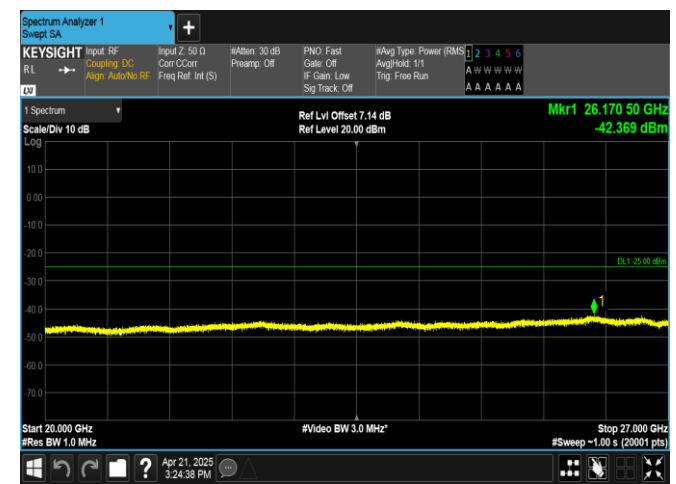
Band41-5MHz-16QAM-41565-25RB#0-20000~27000-PASS
