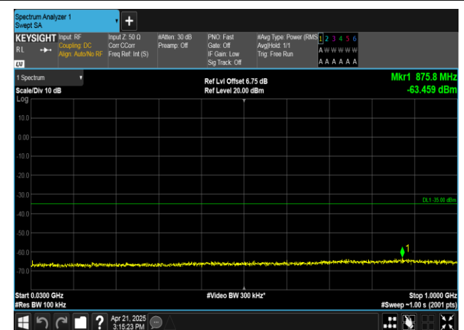
Band41-5MHz-16QAM-40620-1RB#24-30~1000-PASS
