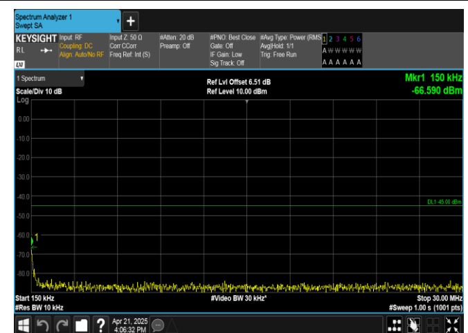
Band41-10MHz-QPSK-39700-1RB#0-0.15~30-PASS
