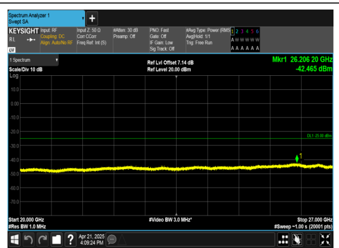
Band41-10MHz-QPSK-39700-1RB#49-20000~27000-PASS
