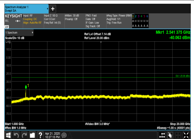
Band41-10MHz-QPSK-39700-50RB#0-1000~20000-PASS
