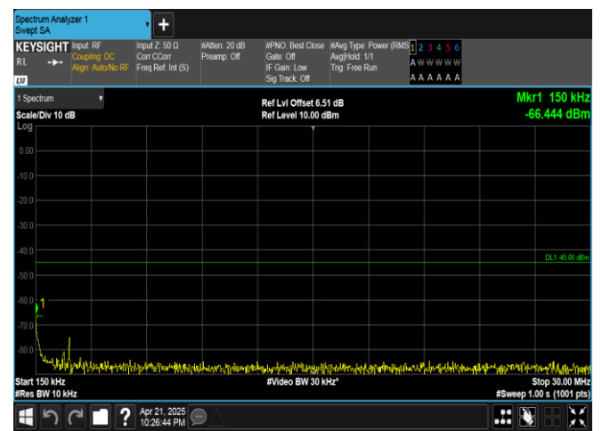
Band41-10MHz-QPSK-39700-50RB#0-0.15~30-PASS
