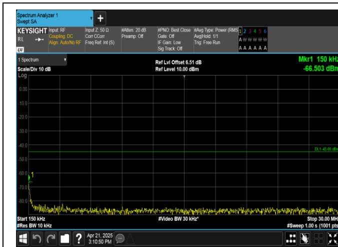
Band41-5MHz-16QAM-39675-25RB#0-0.15~30-PASS
