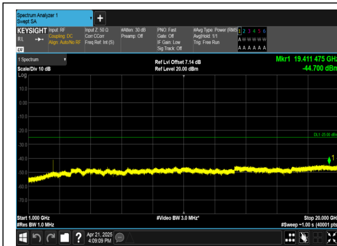
Band41-10MHz-QPSK-39700-1RB#49-1000~20000-PASS
