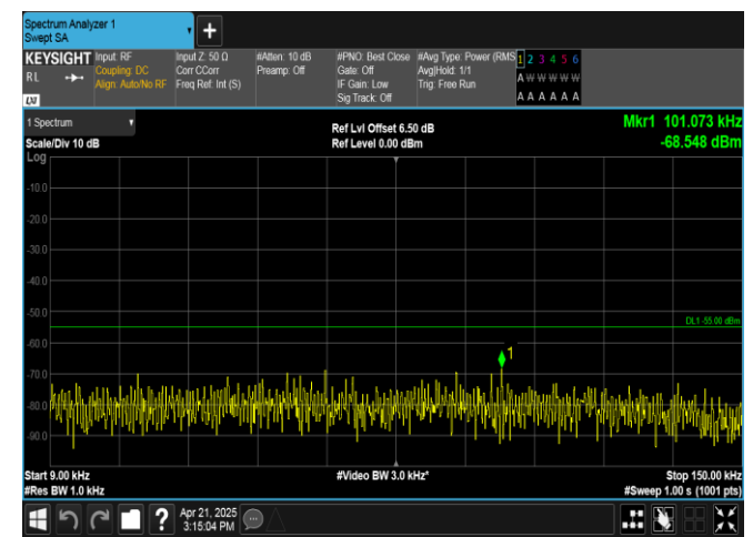
Band41-5MHz-16QAM-40620-1RB#24-0.009~0.15-PASS
