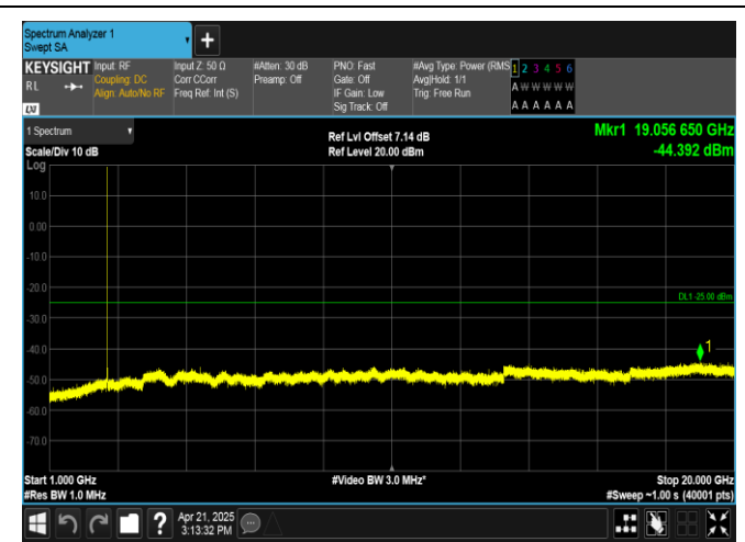
Band41-5MHz-16QAM-40620-1RB#0-1000~20000-PASS
