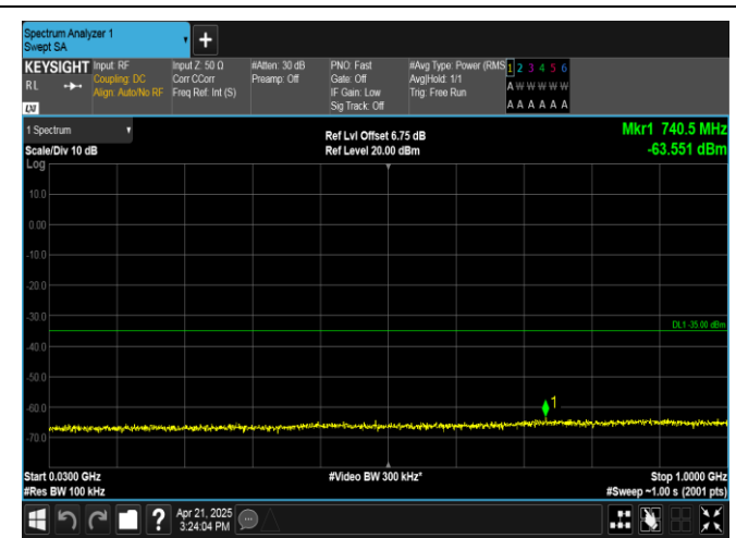
Band41-5MHz-16QAM-41565-25RB#0-30~1000-PASS
