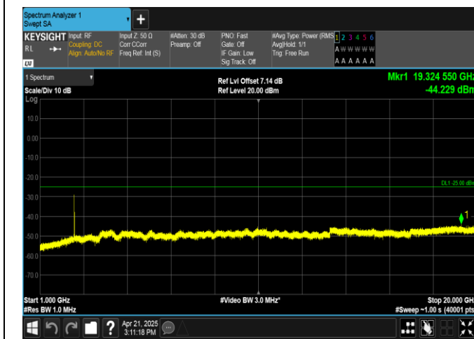
Band41-5MHz-16QAM-39675-25RB#0-1000~20000-PASS
