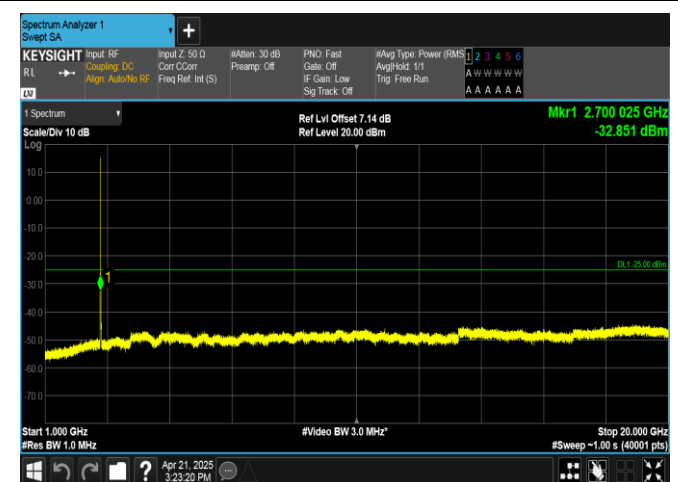
Band41-5MHz-QPSK-41565-25RB#0-1000~20000-PASS
