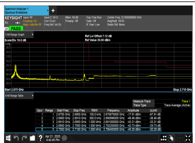
Band41-15MHz-QPSK-41515-1RB#0-PASS
