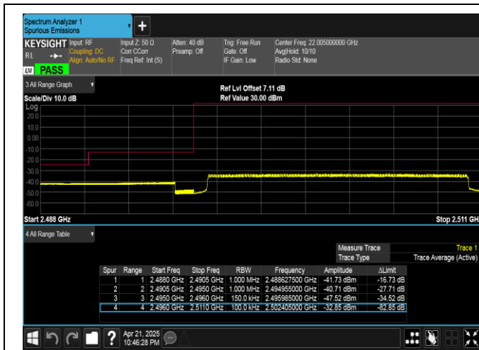
Band41-15MHz-QPSK-39725-75RB#0-PASS
