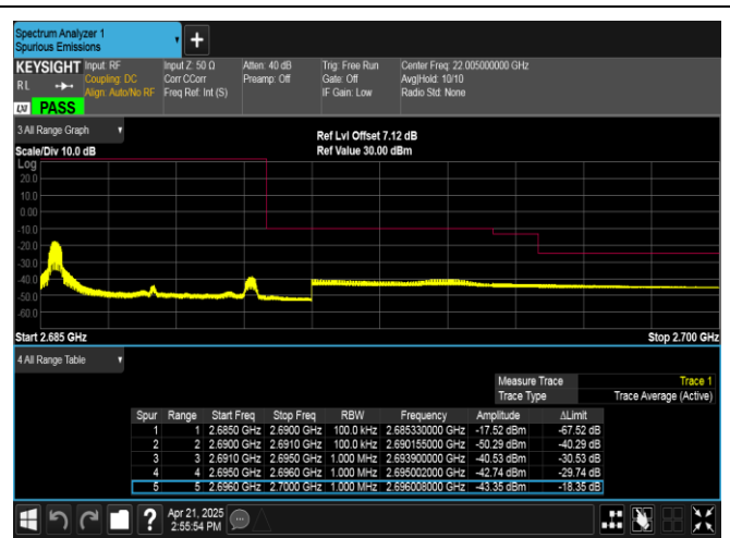
Band41-5MHz-QPSK-41565-1RB#0-PASS
