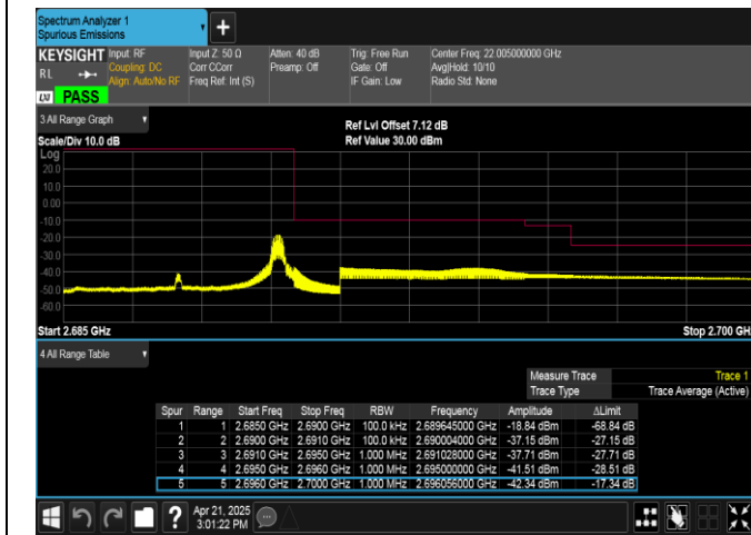
Band41-5MHz-16QAM-41565-1RB#24-PASS
