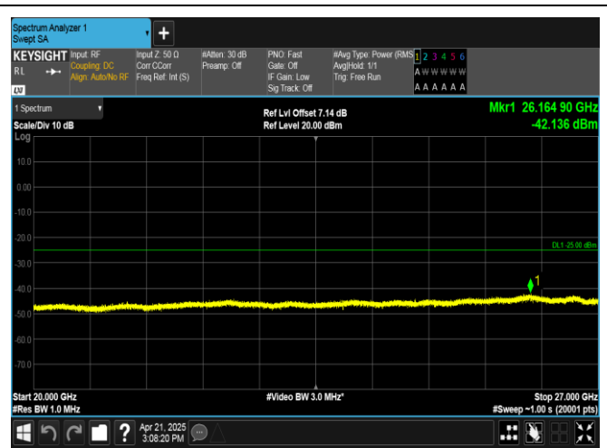
Band41-5MHz-QPSK-39675-1RB#24-20000~27000-PASS
