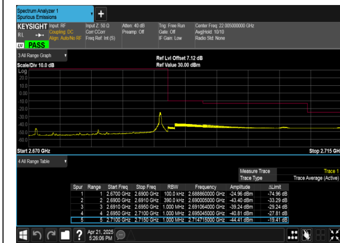
Band41-20MHz-16QAM-41490-1RB#99-PASS
