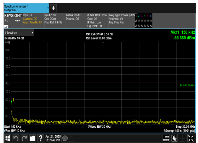
Band41-5MHz-QPSK-39675-25RB#0-0.15~30-PASS
