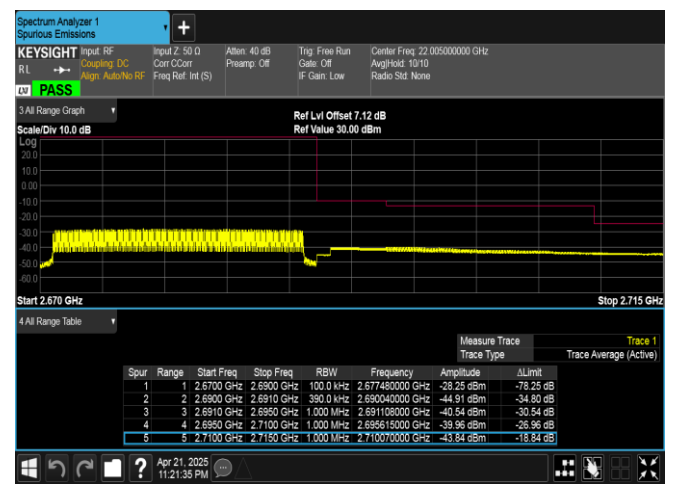
Band41-20MHz-16QAM-41490-100RB#0-PASS
