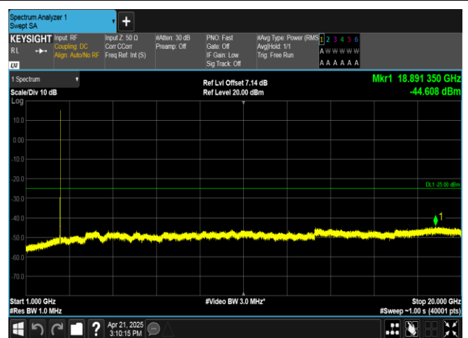
Band41-5MHz-QPSK-39675-25RB#0-1000~20000-PASS
